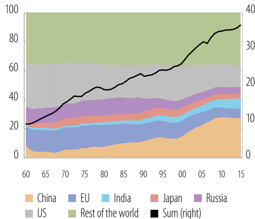
Figure 3 Geographical contribution to world CO 2 emissions (left axis: %; right axis: CO 2 in billions of tonnes)
