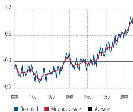
Figure 1 Deviation in land-ocean temperature index (°C)
