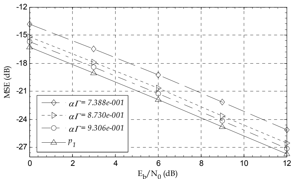
Fig. 8. Channel estimation MSE performance
