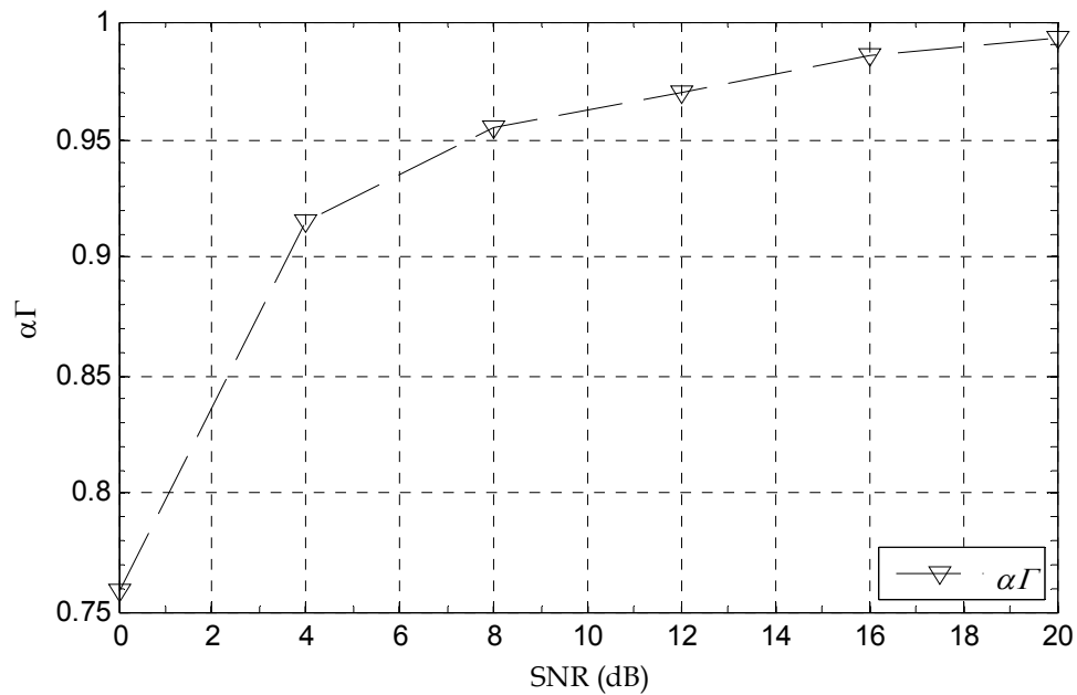
Fig. 5. \alpha_{(k)}\Gamma_{(k)} vs. SNR
