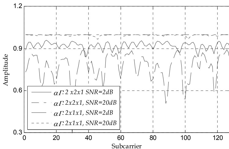
Fig. 6. \alpha_{(k)}\Gamma_{(k)} per subcarriers
