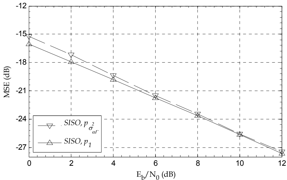
Fig. 7. Channel estimation MSE performance
