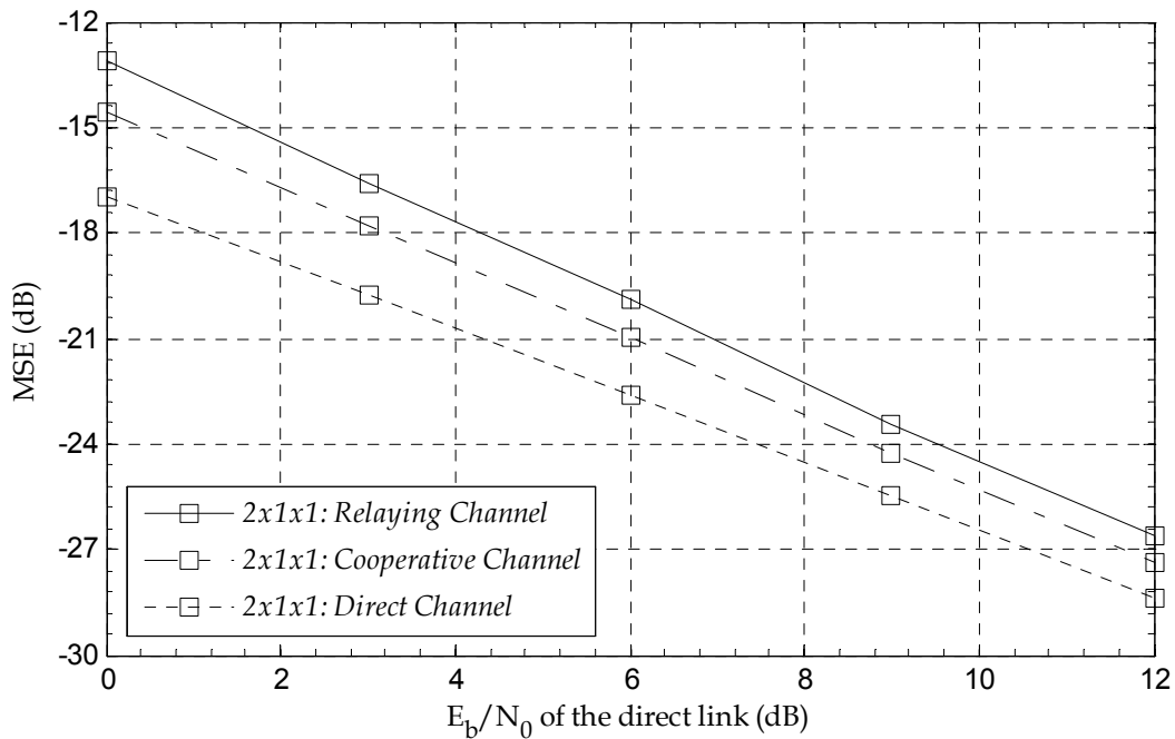
Fig. 12. Channel estimation MSE performance: RA 2x1x1 scheme
