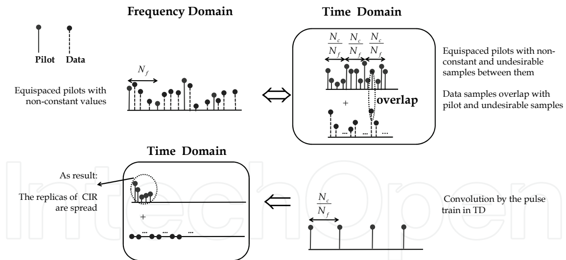
Fig. 4. Pilots with non-constant values result in the overlapped replicas of the CIR
