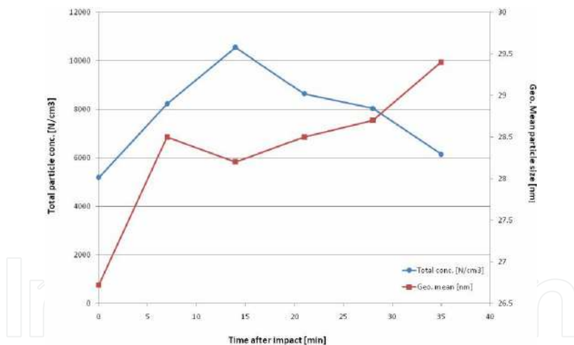
Fig. 9. Geometric mean particle size and total dependency of time after impact.
