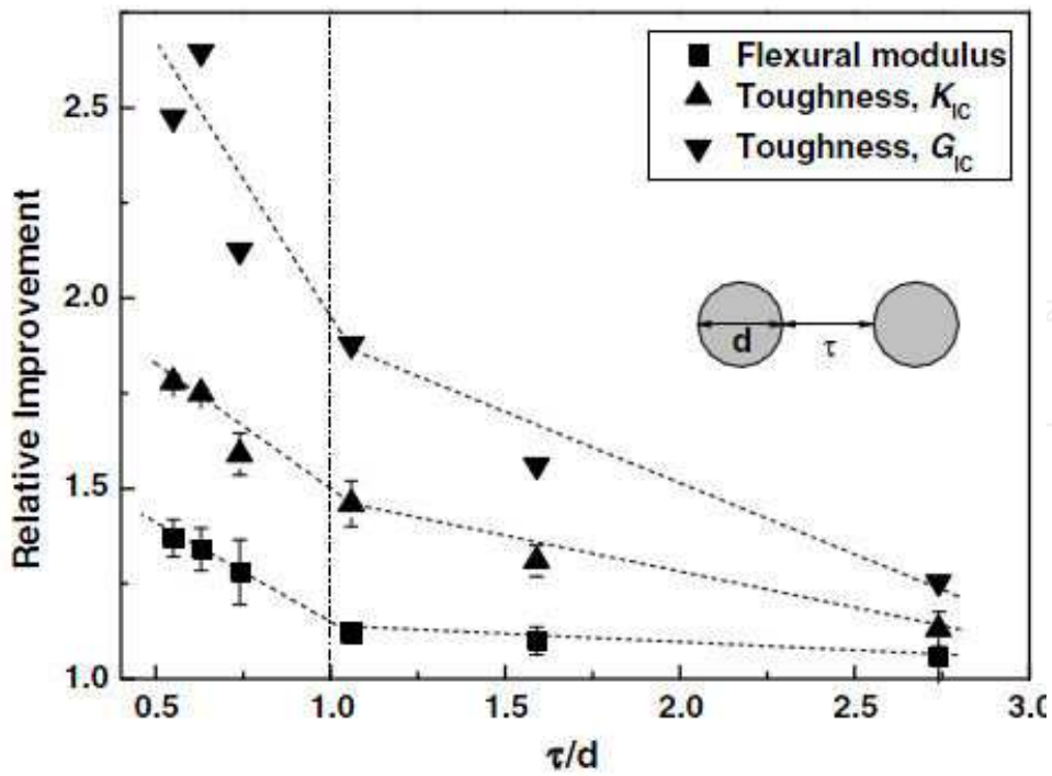
Fig. 1. Correlation between inter-particle distance and mechanical properties of SiO 2 / epoxy nanocomposites (Zhang et al., 2006).
