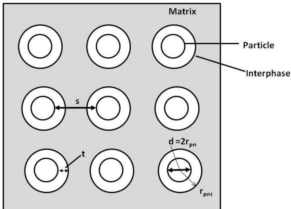
Fig. 5. Geometric parameters in nanoparticle-reinforced composites.
