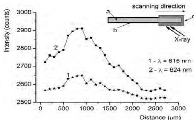
Fig. 17. The spatial responsivity of an extrinsic X-ray sensor for the two peak wavelengths. Insert: a - the POF; b - lightproof jacket; c - phosphorus tip. The focused X-ray beam is scanned along the length of the detecting tip and the profile of the X-ray generated luminescence, as collected by the POSF, is plotted against the distance (McCarthy et al., 2011).
