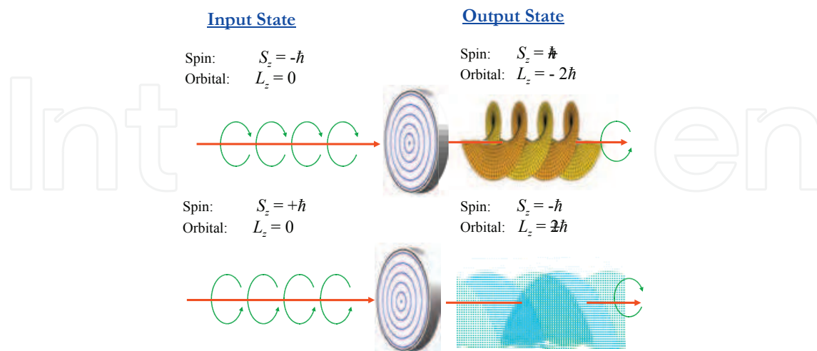
Fig. 9. Schematic representation of the action of a q-plate device with \delta = \pi and q = 1 , like the ones adopted in our experiments (Marrucci et al. (2011)).
