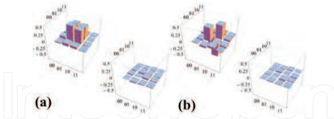
Fig. 10. Experimental density matrices (real and imaginary parts) for the single photon entangled state (Nagali et al. (2009)). The computational values \{0, 1\} are associated to the \{|R\rangle, |L\rangle\} polarization states, and to \{|+2\rangle, |-2\rangle\} for the orbital angular momentum m for the first and the second qubit, respectively. The incoming state on the QP is (a) |H\rangle_{\pi}|0\rangle_m , and (b) |V\rangle_{\pi}|0\rangle_m .
