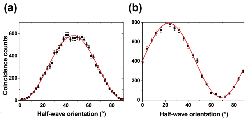
Fig. 14. Coincidence rate [D_A, D_B] measured as a function of the angle \theta of the half wave plate on the arm k_A for OAM detected state (a) |+2\rangle and (b) |h\rangle_{o_2} (Nagali & Sciarrino (2005)).
