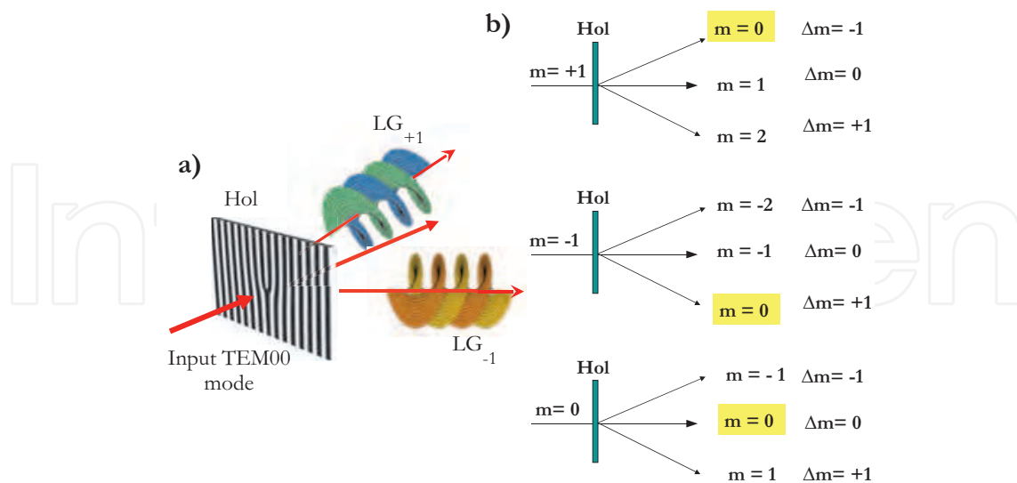
Fig. 3. a) Schematic representation of a hologram and its action on an optical field. b) Action of a single-fork hologram on different input states. In the yellow box have been enlightened the modes that can be coupled to single mode fiber for analysis.
