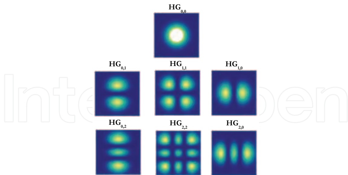
Fig. 2. Intensity profiles for different HG modes. As can be observed, the zero order of HG coincides with the one of LG modes that is, the gaussian mode.
