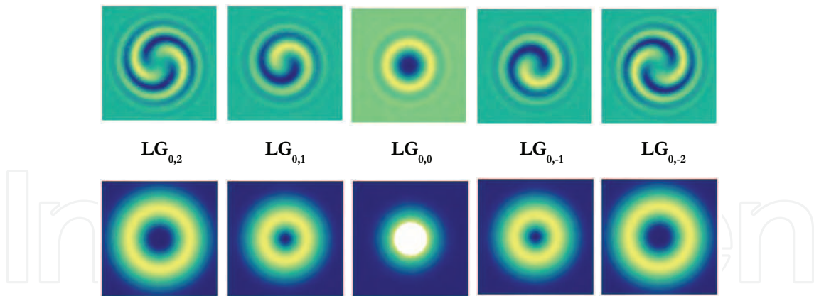
Fig. 1. Examples of LG modes. Top: phase profiles for different LG modes and Bottom: intensity profiles of the same modes.
