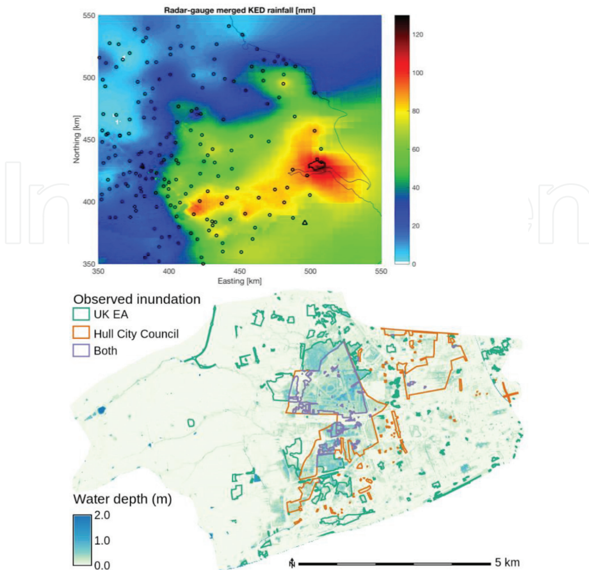
Figure 6. Merged radar-rain gauge rainfall product (top) used to simulate a flood (bottom) in Hull, England [26].
