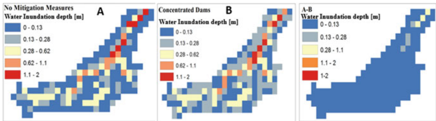
Fig. 13.20 Flood depths with concentrated dams; A-B represents the difference between the flood depths under the situation in which mitigation measures are taken and the situation in which no mitigation measures are taken in the Sume Basin based on the March 2014 flood event
