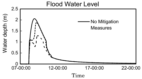
Fig. 13.18 Flood depth during the Gonu Cyclone in the Sume basin measured at a point downstream
