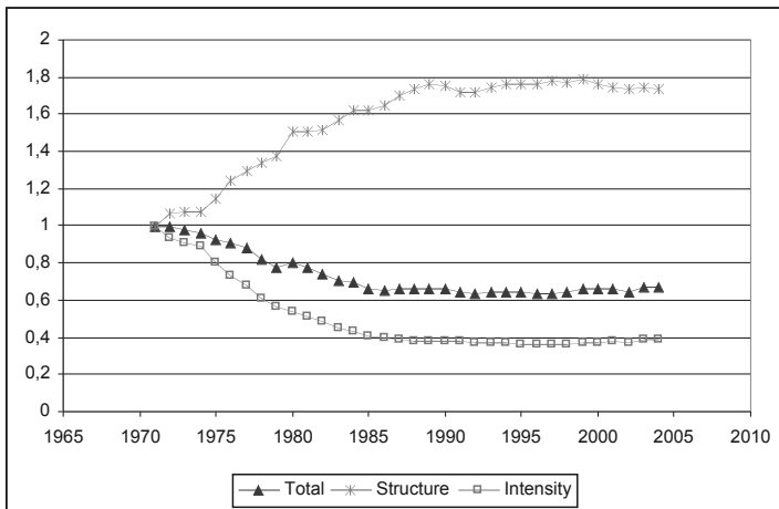
Figure 12. Sato-Vartia (1971=1)
