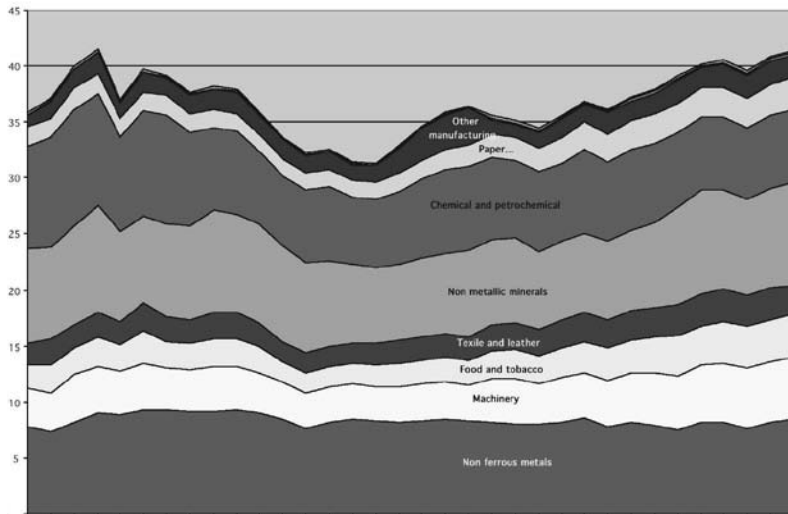
Figure 6. Italian industry energy consumption per sector (mtoes): 1971-2005
