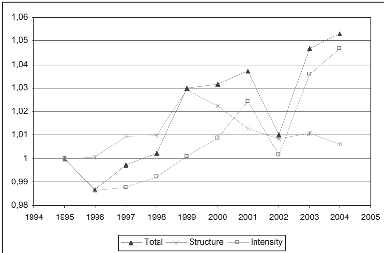
Figure 14. Sato-Vartia (1995=1)
