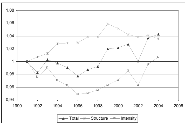
Figure 13. Sato-Vartia (1991=1)
