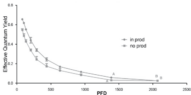
Figure 31. Effective Quantum Yield . PFD= Photon Flux Density ( \mu\text{mol photons m}^{-2} \text{ s}^{-1} ). The curves obtained for the two conditions are significantly different from each other, except for the last two points. t-test was performed for each PFD.
