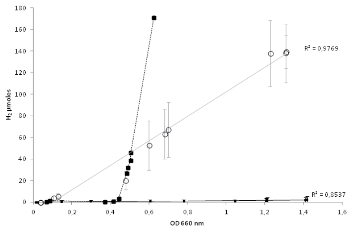
Figure 19. H_2 accumulated in the headspace versus cellular growth expressed as optical density at 660nm. Data for all NH_4^+ concentrations (2.5-10.0 mM) are included for Rp. palustris CGA009 wild type (■) and CGA676 mutant strain (○), except for the two wild-type replicates that eventually produced H_2 with 2.5mM NH_4^+ (dotted line). Error bars indicate SD.
