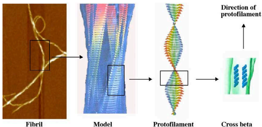
Figure 1. Close-up view of the structural organization of an amyloid fibril. The four protofilaments are wound around each other and their core structure is a row of \beta -sheets where each strand runs perpendicular to the fibril axis. From (Stefani, 2004).
