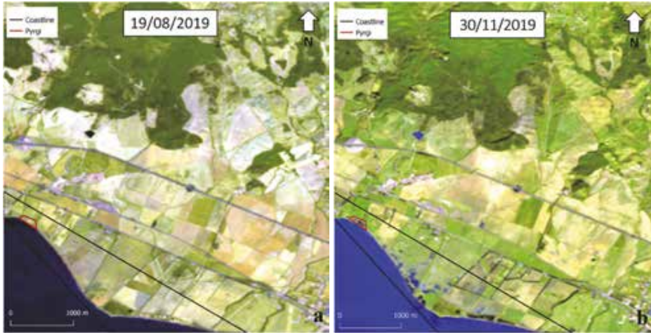
Figure 3 - Comparison of images captured by Sentinel 2-A and processed with Google Earth Engine of the same area in summer, image captured on 19 August 2019 (a), and in autumn, image captured on 30 November 2019 (b).
