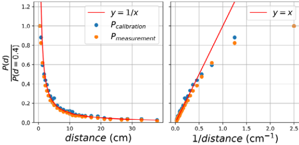
Figure 4 – Normalized RMS pressure levels at 2.4 kHz with distance (left) and with inverse of distance (right).
