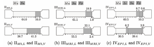
Fig. 4: Serial stacked specimens based on M5, MRI and EPI replicas with layer lengths l_i (mm): muscle-Mu, ligament-Li, superficial-Su, epithelium-Ep.
