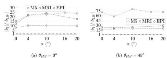
Fig. 2: Normalised non-oscillation mode ( j=1 ) amplitude magnitude: a) top view ( \theta_{HS}=0^\circ ), b) diagonal ( \theta_{HS}=45^\circ ) view.
