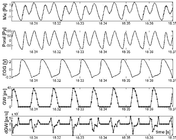
Fig. 5 – Samples of analyzed signals for vowel phonation, where GW and dGW are shown for VFs.
