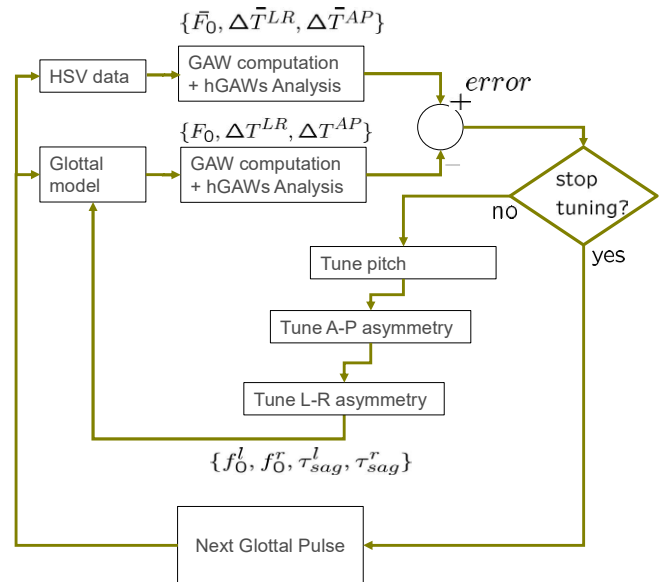
Fig. 3. Automatic pitch-synchronous parametric tuning
