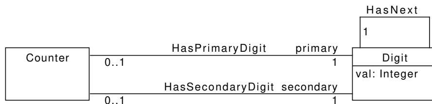
Figure 23.1: A metamodel for a simple counter with two digits
