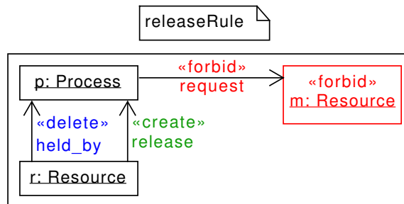
Figure 20.2: A transformation rule with combined LHS and RHS in a visual notation
