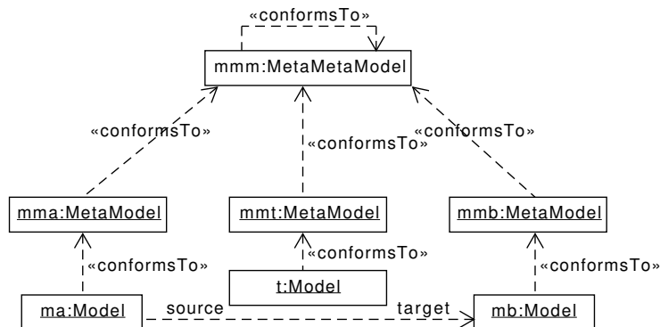
Figure 25.1: The classical out-place transformation scenario
