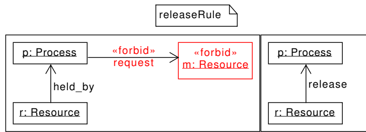
Figure 20.1: A transformation rule with separated LHS and RHS in a visual notation
