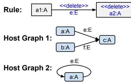
Figure 20.3: Illustration of differences between DPO and SPO
