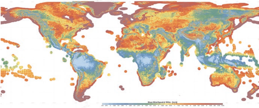
Fig. 10.2 The global wind energy potential shown as mean wind speeds 100 m above ground. (Source: Global Wind Energy Atlas 2019)
