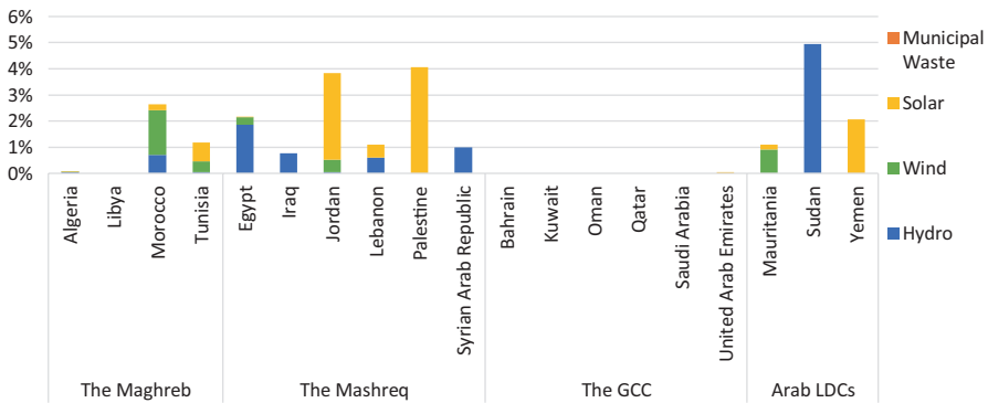
Fig. 33.12 Renewable energy share in TFE (excluding solid biofuel), 2016. (Source: IEA (2018), World Energy Balances; Energy Balances, UN Statistics Division (2018))
