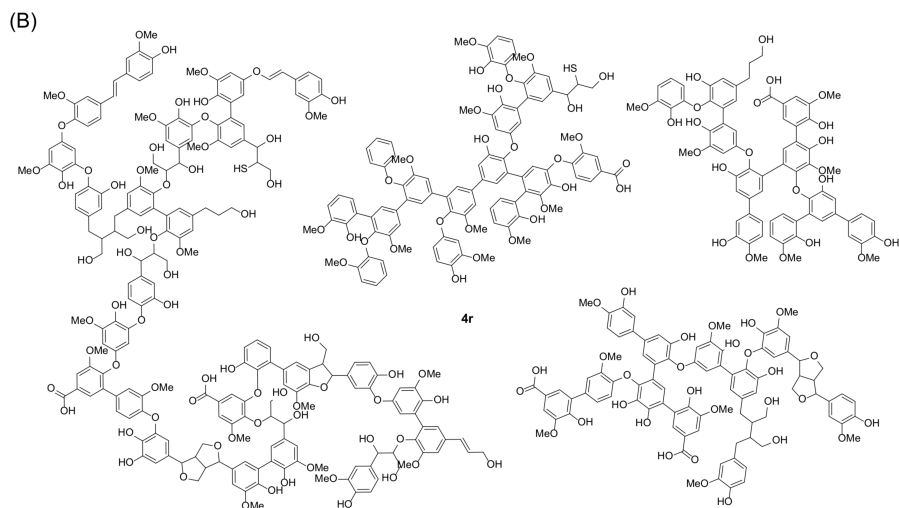
Figure 4. Lignin structures showing characteristic interunit bonding motifs and functional groups for different types of lignin (continued): (A) kraft lignin (outdated view); (B) kraft lignin (proposed revised structure composed of polymeric and oligomeric units); (C) lignosulfonate.
