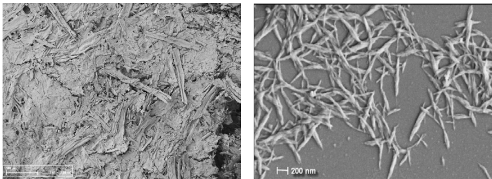
Figure 5. Scanning electron microscopy (SEM) micrograph of wood residue after the liquefaction process ( left ). SEM micrograph of nanocrystalline cellulose isolated form wood meal ( right ).
