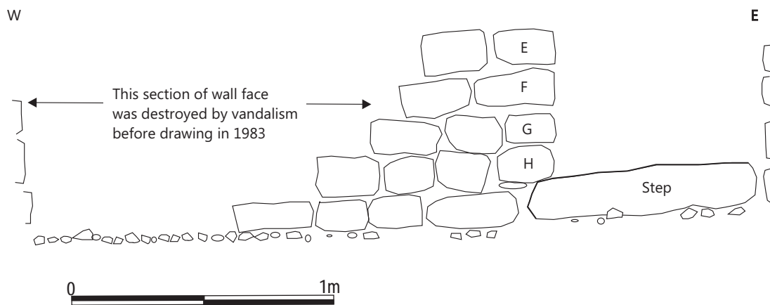
Fig re 8 Elevation of the north wall of the strong room, as depicted at 8
