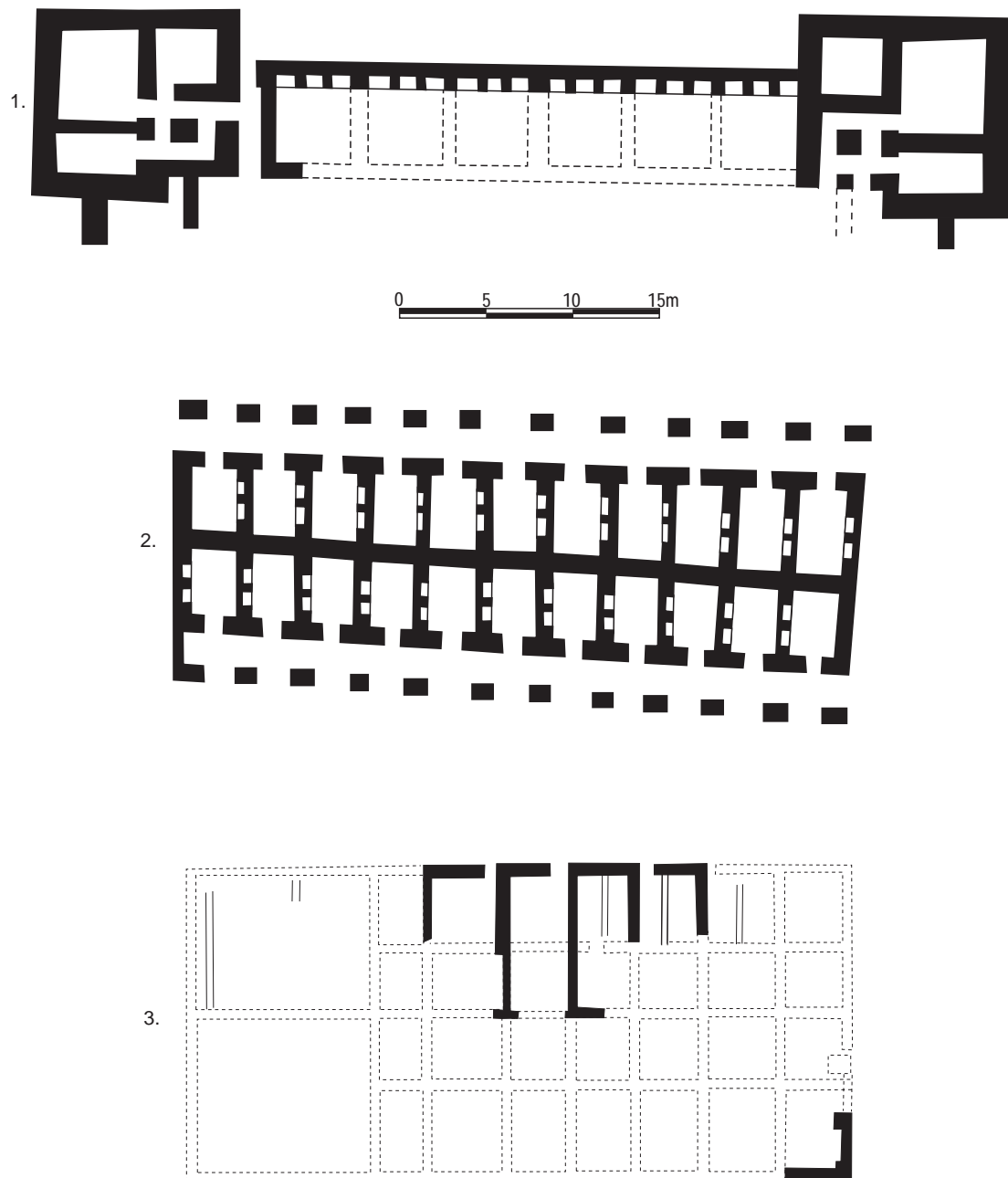
Figure 4 Late Roman cavalry barracks 1 Qasr Bsh r 2 B B – two storey barrack range against the north curtain, 2 Tim d B B back to back, two storey barracks, 3 Haltonchester's single storey back to back barracks. Scale 0
