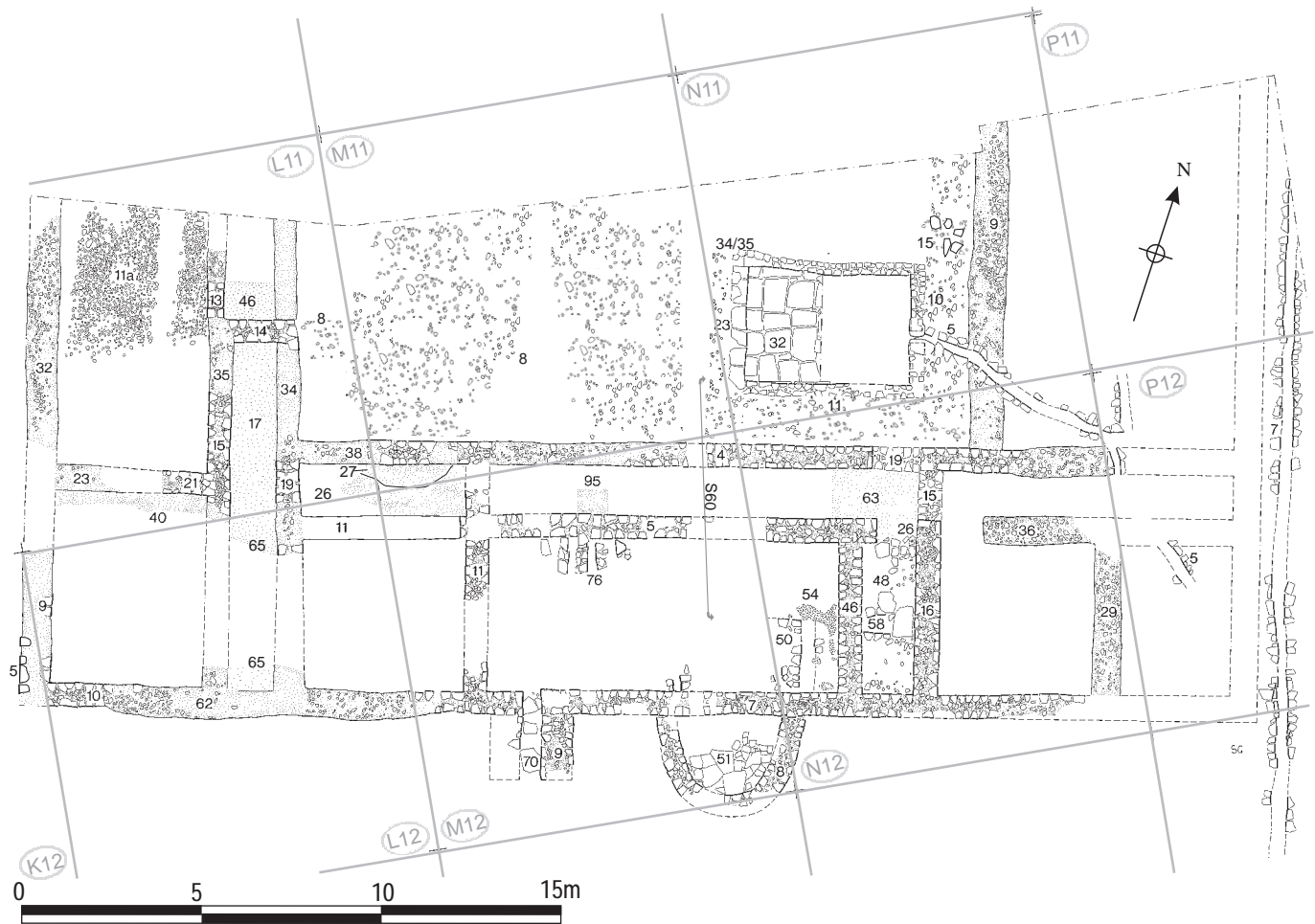
Figure 9.11: Building 13 Phase 3iv at 0
