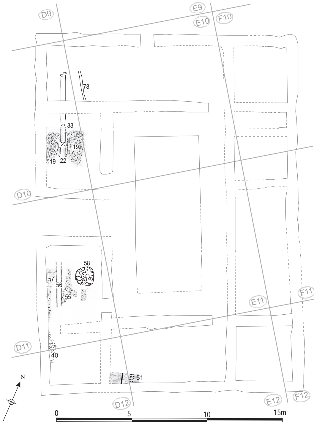
Figure 5.03 Evidence for the timber hospital (Building 21) (at 1:10 scale) with the outline of Building 8 shown for reference.
