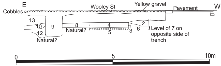
Figure 9 Section across the east defences in grid square R5 at Seg
