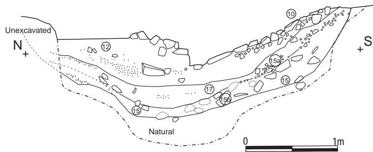
Figure 13 Section (S16) across pit Q04:10 in the north intervallum. Scale 1:10
