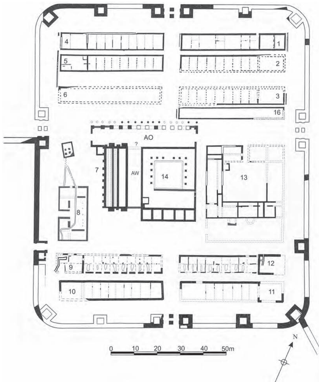
Fig. 2. Period 3. The fort in the late second/early third century.
