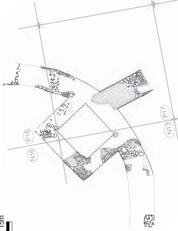
The south-east angle tower, at 1:200
