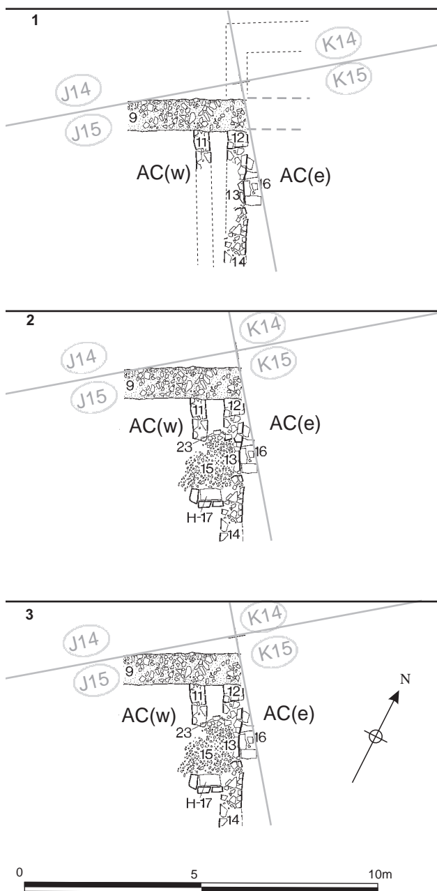
Figure 16 2 Plan showing successive phases in the area of the doorway between AC (w) and AC (e). Scale 1:100
