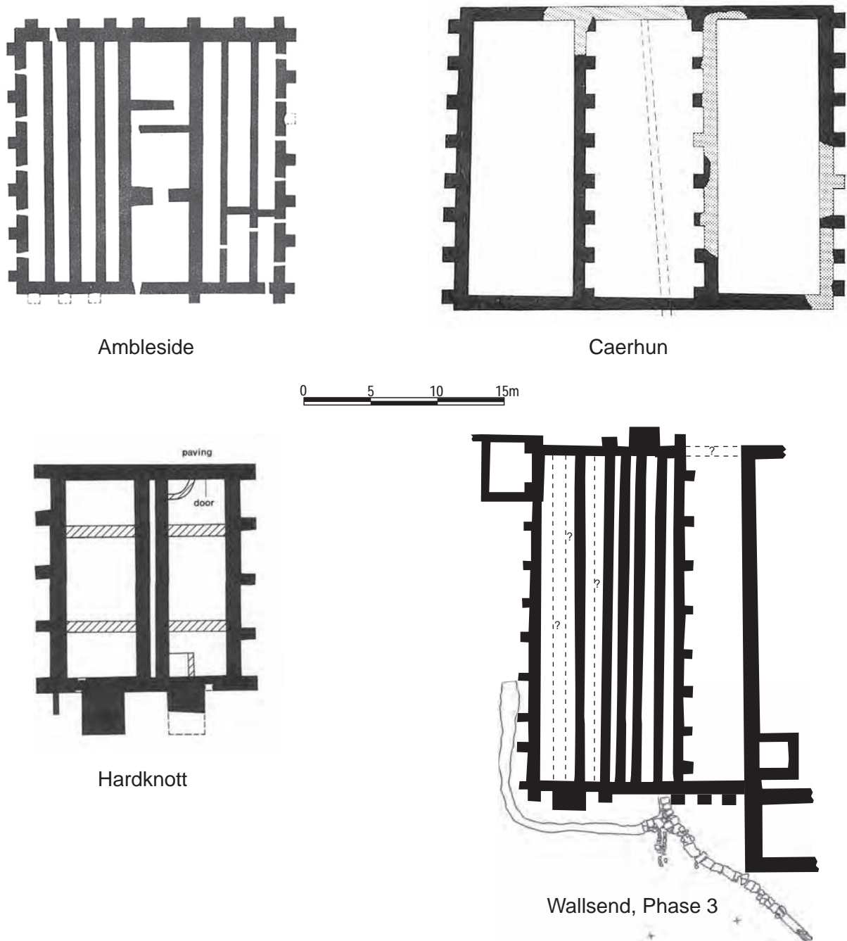
Fig. 4.24 Granary comparison plan, showing examples of granaries with enclosed yards or covered extensions, ④
