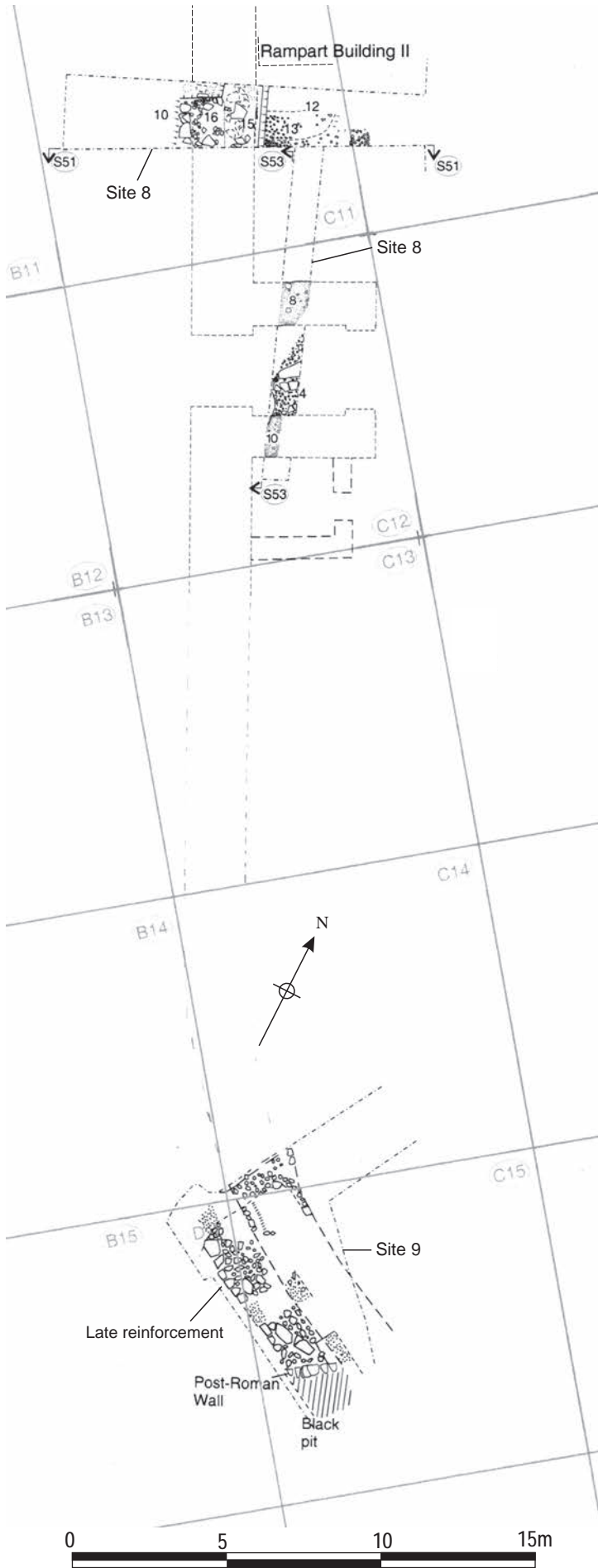
Fig. 1. Plan showing the trench locations (Sites 8–10) in the western defences, examining the porta quintana, curtain wall and rampart, and the SW angle. Scale 0
