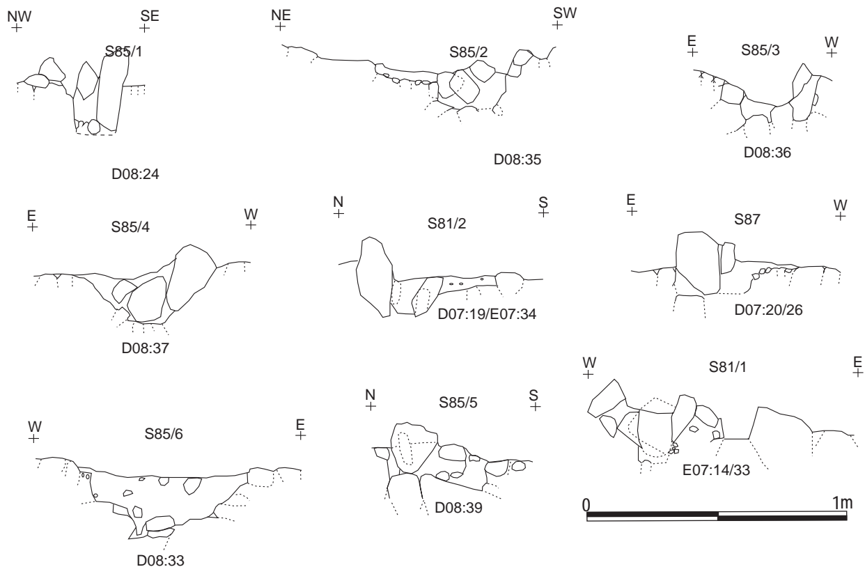
Figure 8 Section drawings of postholes associated with Building AS, at D
