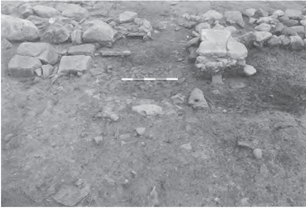
Figure 8 Pivots tone P05:21 associated with the Phase 1 Sub-Phase 1 doorway into the side passage of Contubernium 1 from the north.
