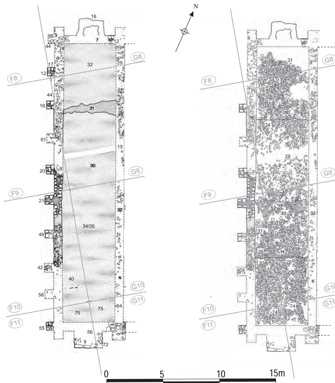
Figure 4.04: Clay base and cobble and flag makeup layers of the west granary at 1:200.
