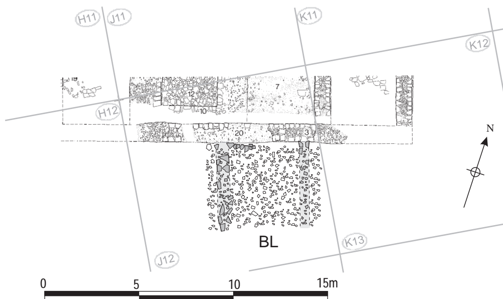
Fig. 8 Building BL south of Building 4 at 0
