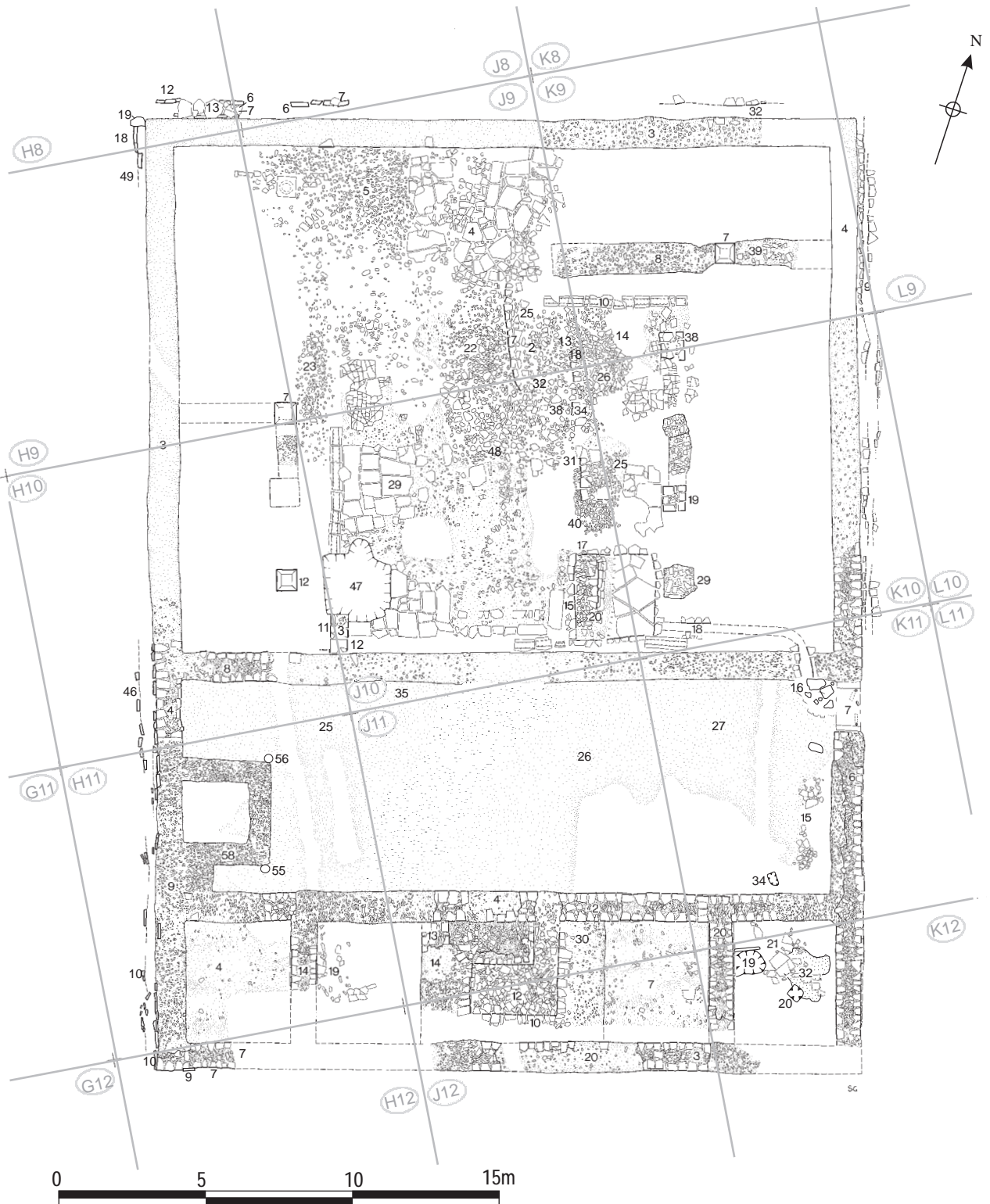
Fig re 8 Building 4 showing the Phase 4 courtyard and the latest recorded Phase 3 activity in the cross hall and south range where the Phase 4 levels were truncated, plus the rubble demolition fill in the strong room. Scale 1:200.
