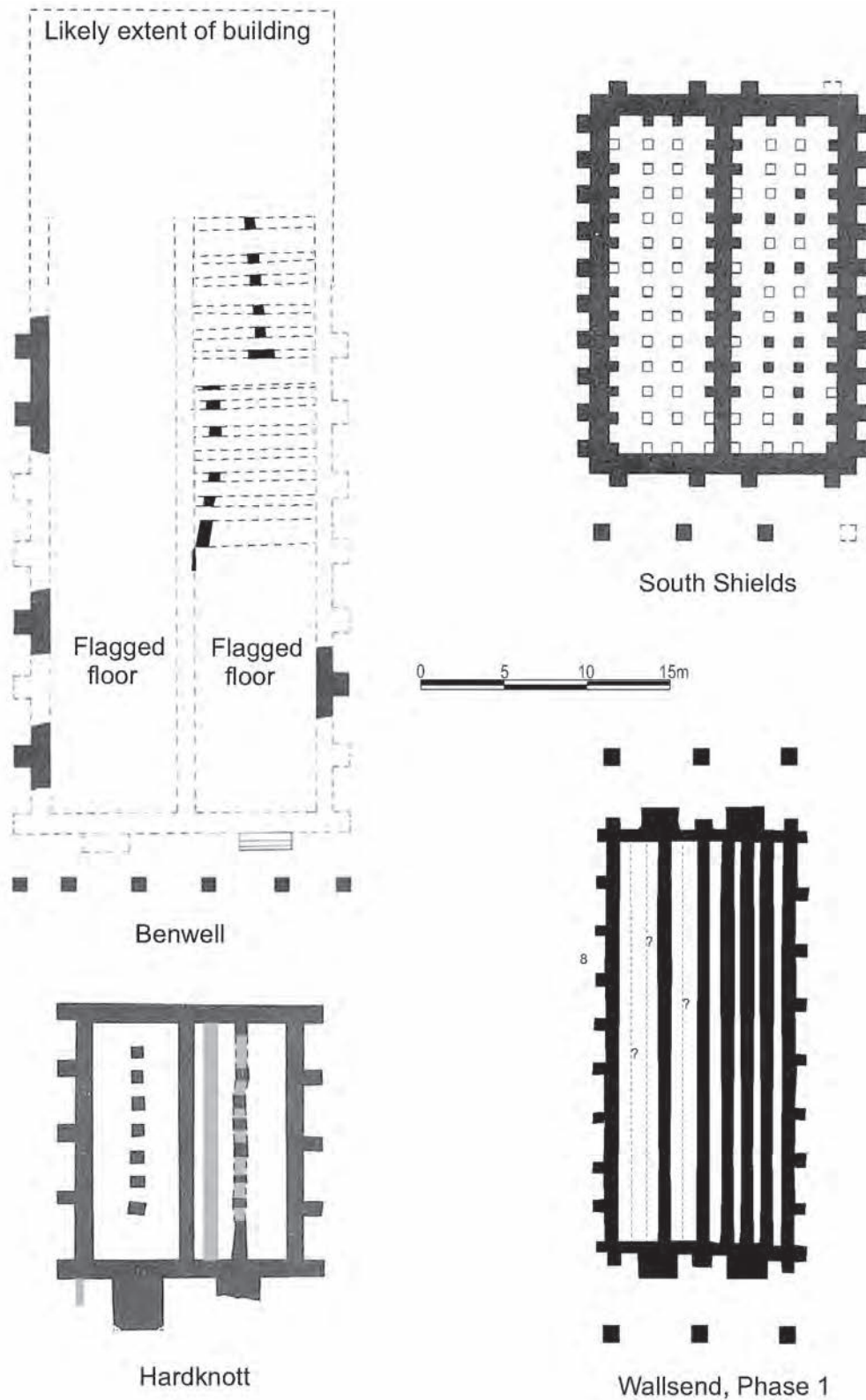
Figure 2 Granary comparison plan, showing examples of double granaries, 1
