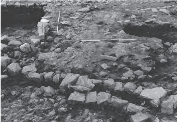
Figure 7.14: Drain E08:35 feeding into the north east corner of the cistern, from the east.
