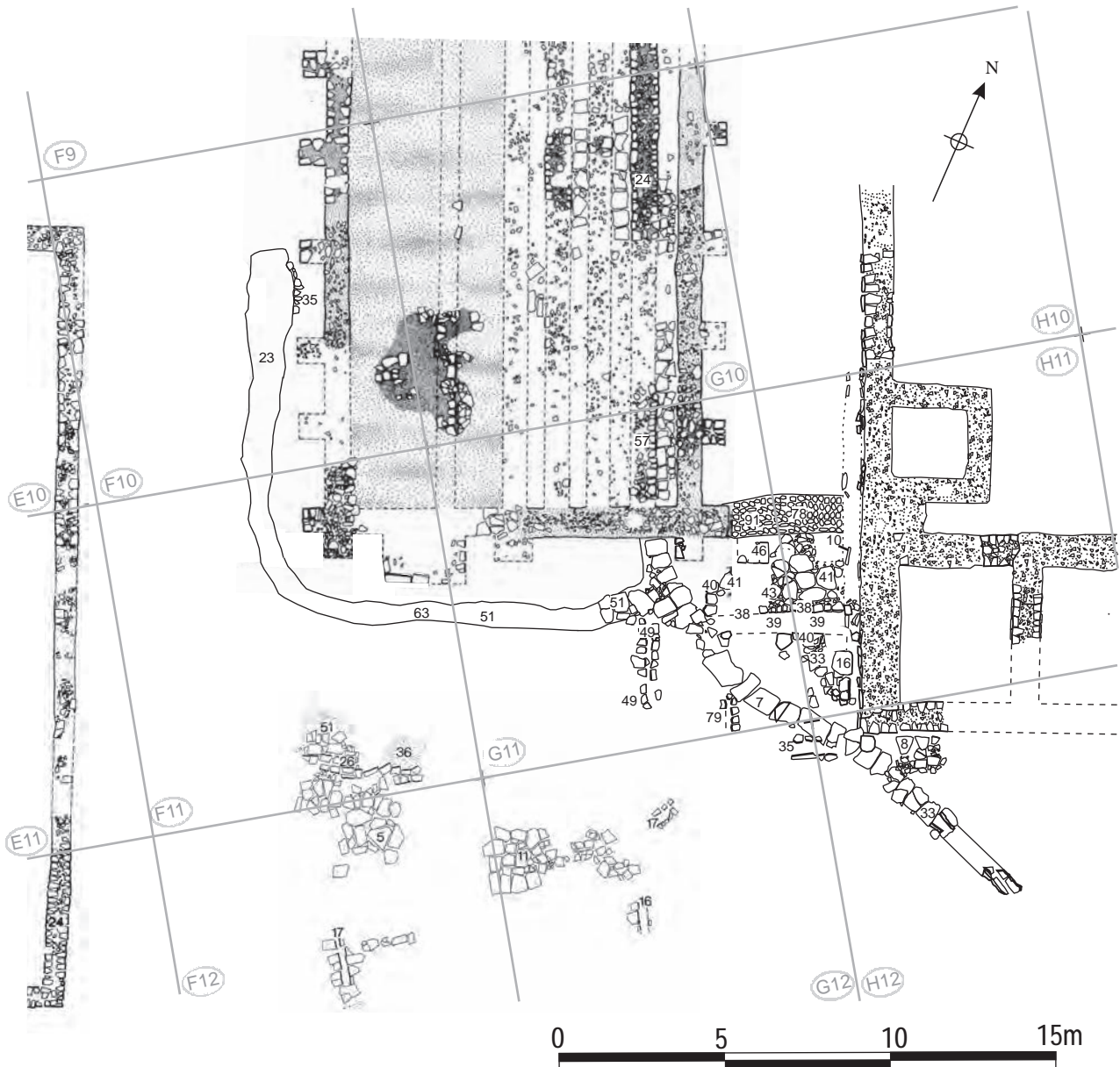
Figure 4.9 The south end of the granary (Phases 3 and 4) showing the south wall of AW and the surrounding storm drains F10:23/F11:63/G11:51 and G11:07/H12:33, at 1:200. Also shown for reference are the flagged floors of the third-century timber building in this area.
