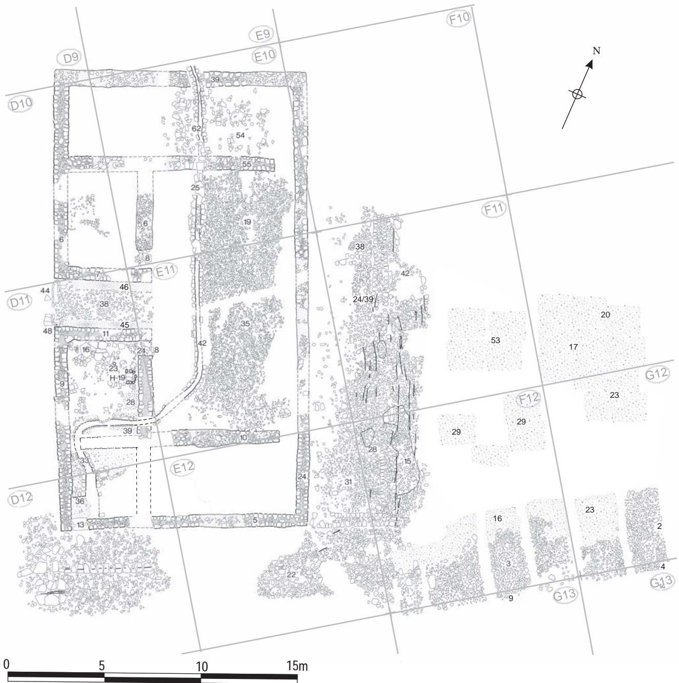
Fig re 3 Building 8 and adjacent road surfaces, Phase 2 Scale 0
