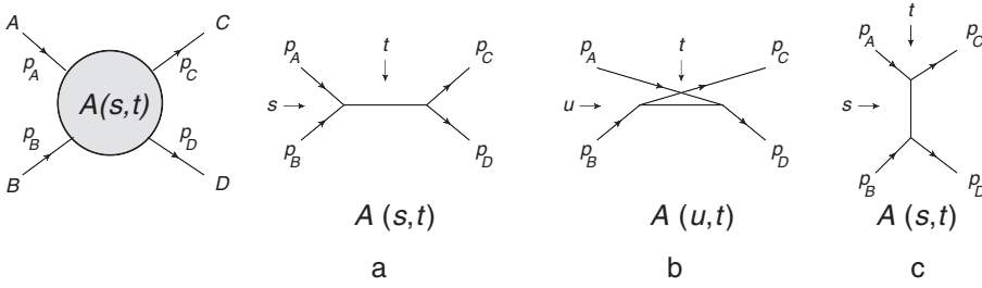
Fig. B.1. Scattering amplitude for a 2 \rightarrow 2 process and tree-level diagrams for the process in the \phi^3 theory in three different channels, s , u , and t , corresponding respectively to parts a, b, and c of the figure.
