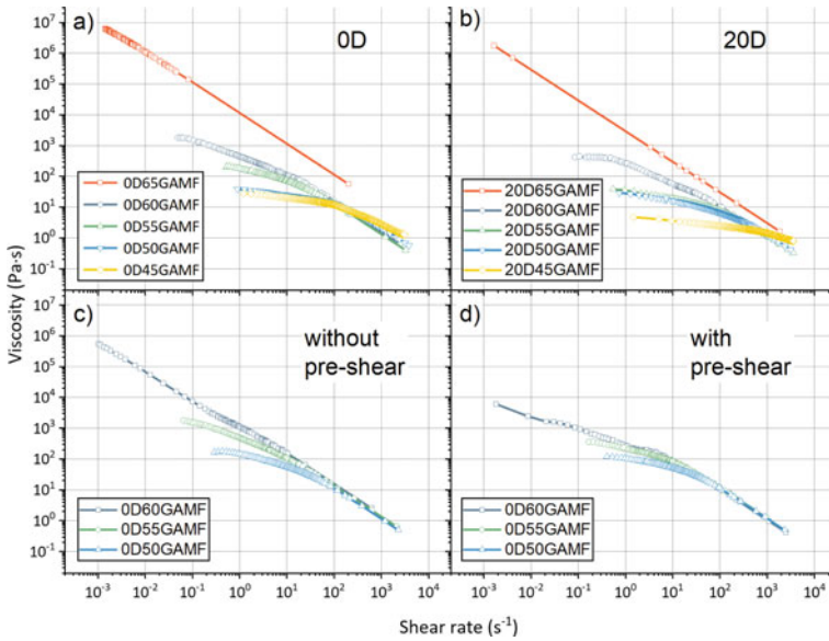
Fig. 9 Flow ramp test for GAMF recycle inks: a tests on GAMF ink without reactive diluent, b tests on GAMF ink containing 20 wt% of reactive diluent, c tests on GAMF ink performed without the pre-shear step, d tests on GAMF ink performed with the pre-shear step
