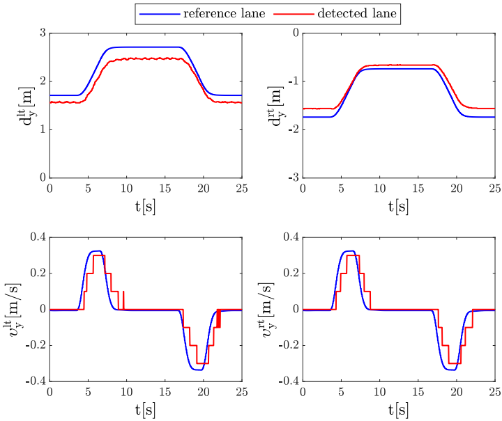
Figure 3.2: Verification process with the closed-loop HiL test bench using the example of the detection of left lane markings (left) and right lane markings (right) on the basis of a monocular camera sensor [ESW + 16].
