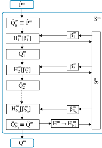
Figure 4.9: Modular architecture of the phenomenological sensor simulation [ESFG19b].
