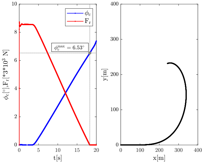
Figure 4.3: Driving around a tight curve at lateral acceleration of 6 [ \text{m}/\text{s}^2 ] and longitudinal velocity of 80 [km/h] including roll movement compared to weight force on the rear axle (left) and Ego-vehicle trajectory (right).
