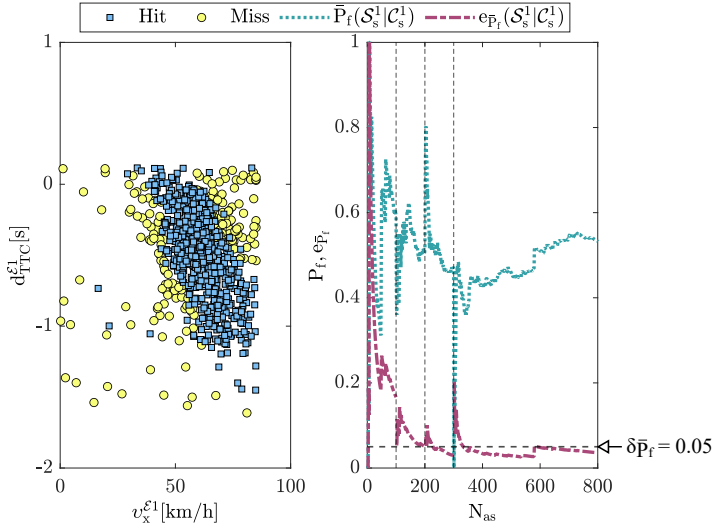
Figure 7.8: Estimation of failure probability for the severity level \mathcal{S}_s^1 using the AIS method. For comparative purposes, these calculations in MCS are shown in figure 7.4.
