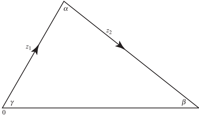
Figure 18.2 The unitarity triangle.
