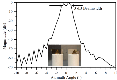
Figure 3.15: Measured radiation pattern from the experiment with two identical TCRs with the size of 7.9 cm, which are located in the radial range of 9 m from the radar. The TCRs are detected in azimuth angles of 0.5^\circ and -0.5^\circ . The setup of the measurement in the test environment is shown in the inset.
