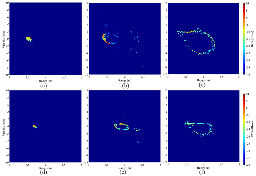
Figure 5.12: Extracted range, velocity, and RCS data along the left leg ( \varphi = -1^\circ ) of a human jogging (1.94 m/s) and walking (0.69 m/s); (a) jogging ( \theta = 0^\circ ); (b) jogging ( \theta = -8^\circ ); (c) jogging ( \theta = -14^\circ ); (d) walking ( \theta = 0^\circ ); (e) walking ( \theta = -8^\circ ); (f) walking ( \theta = -14^\circ ). (Figure based on [2], ©IEEE.)
