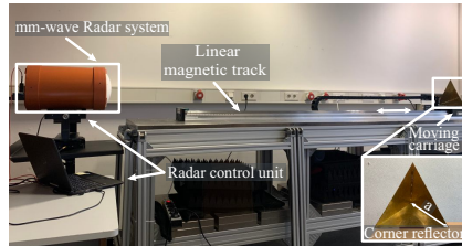
Figure 5.1: Setup for extracting the range-velocity information using a TCR, which can move on the linear magnetic track to verify the EFE algorithm. The TCR is aligned to the main beam of the Radar system. (Figure based on [2], ©IEEE).
