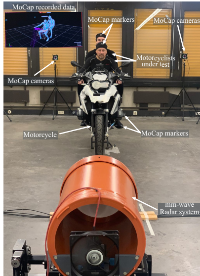
Figure 5.16: Setup for monostatic high-resolution RCS measurement to extract the range, velocity, and RCS information of different body parts of two motorcyclists in motion.
