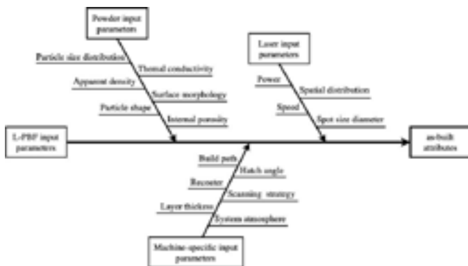
Figure 3. A schematic diagram showing a summary of L-PBF input parameters.
