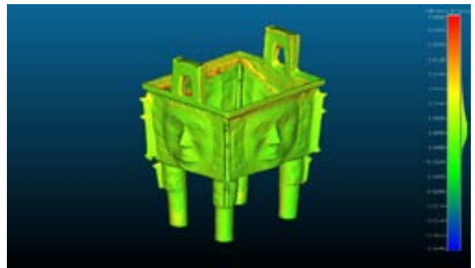
Figure 4. The mesh distance between the model obtained from the phone and the camera in the museum.
