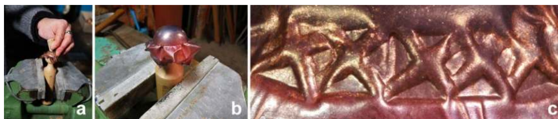
Figure 10. Experiments for embossing bowl-shaped objects; a-b – modern ball-shaped punch as an anvil for the embossing procedure; c – embossed ornamentation on the experimentally produced bowl-shaped object, with overlapping parts, visible outlines of the punch and crinkles of the material displacement.
