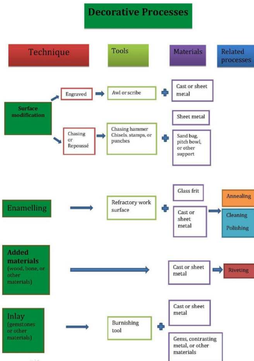
Figure 7. Flow chart of Decorative Processes
