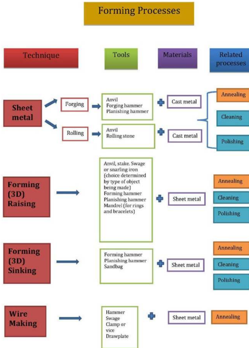
Figure 5. Flow chart of Forming Processes
