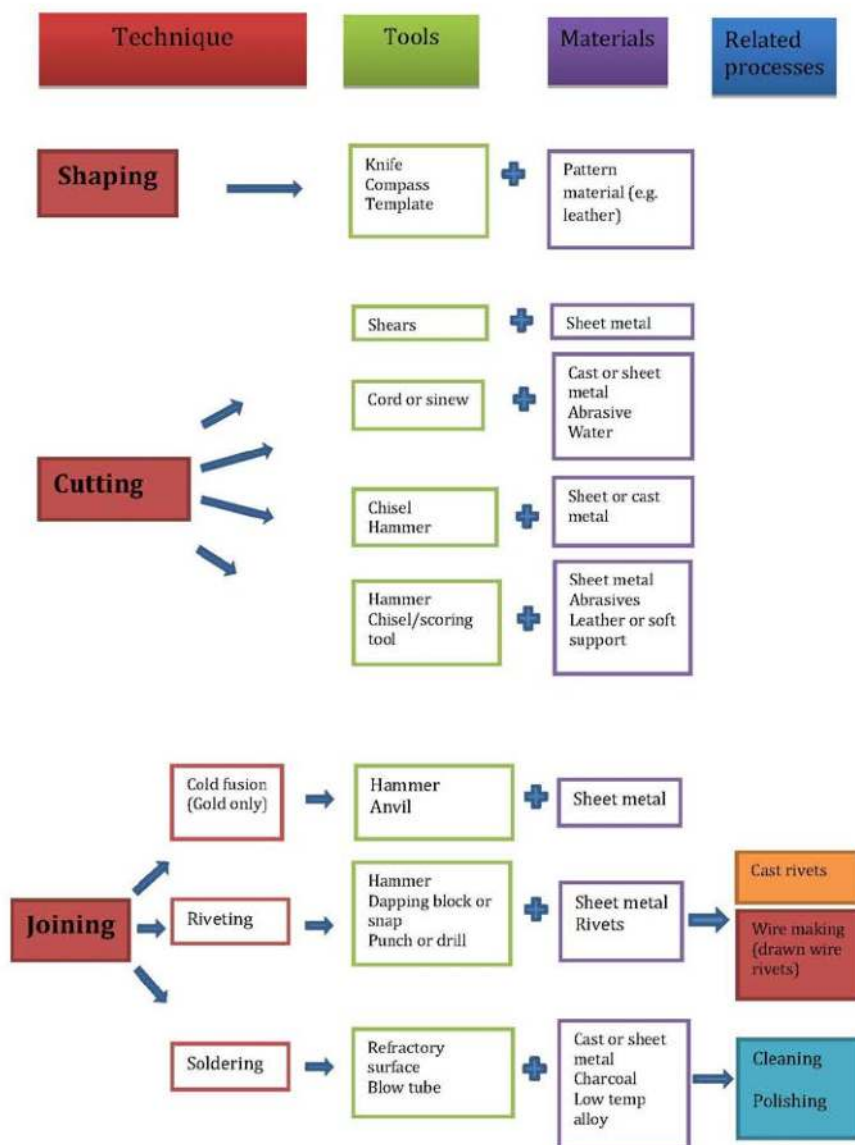
Figure 6. Flow chart of Joining Techniques
