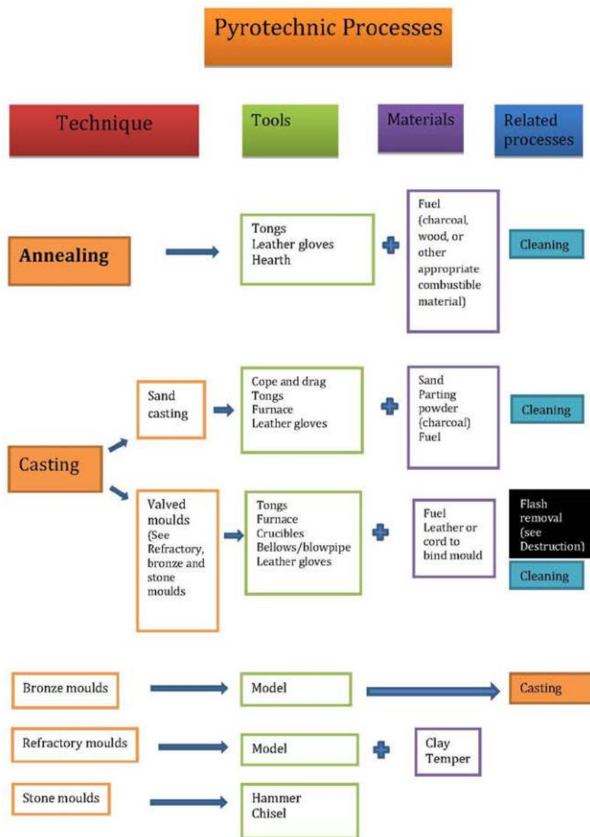
Figure 4. Flow chart of Pyrotechnic Processes
