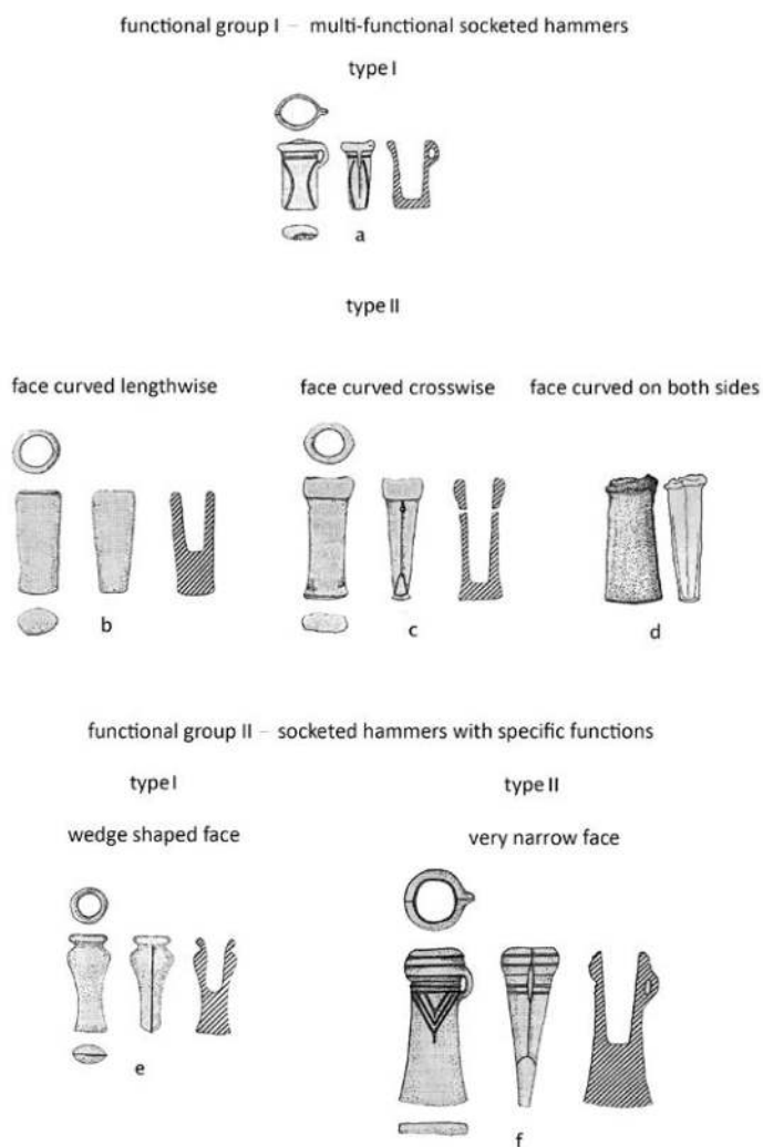
Figure 3. Multi-functional and special equipment hammers based on their functional attributes: a Jibou, b Sâmbriaș, c Gușterița, d Brvniste, e Corund, f Arad II (adapted from Nessel 2008).
