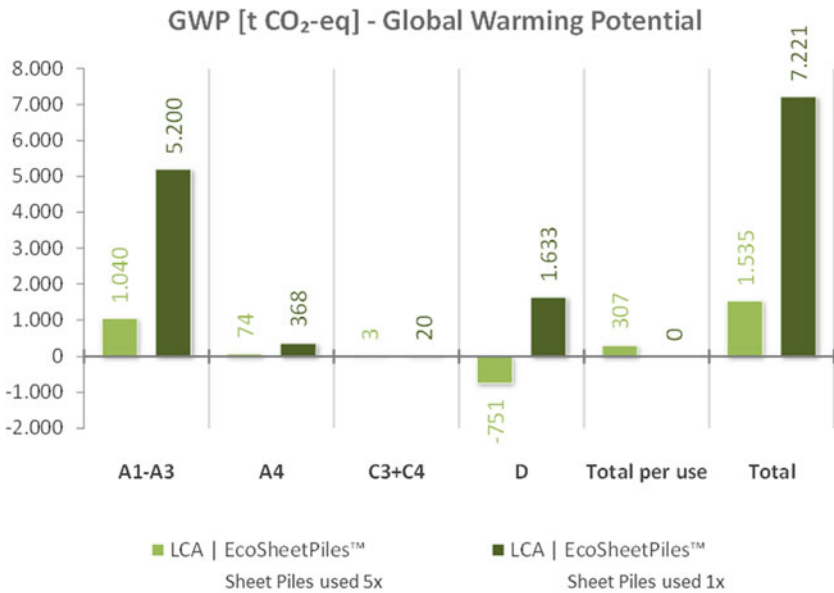
Fig. 3.6 GWP based on EPD EcoSheetPiles—Influence of reuse
