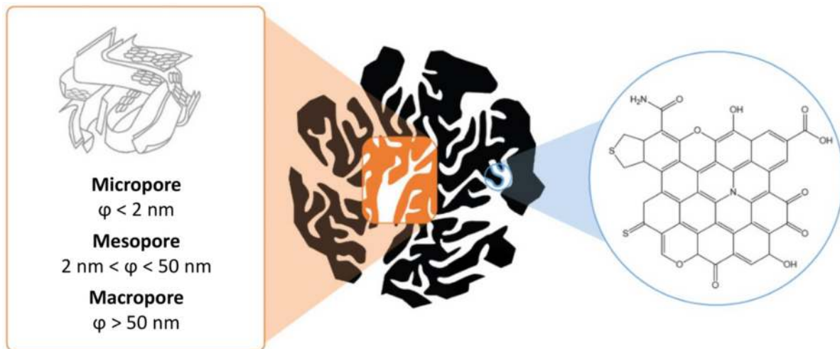
Figure 8.6 Representation of nanoporous structure and surface chemistry groups on AC. Source: From Mestre et al. (2022a) .
