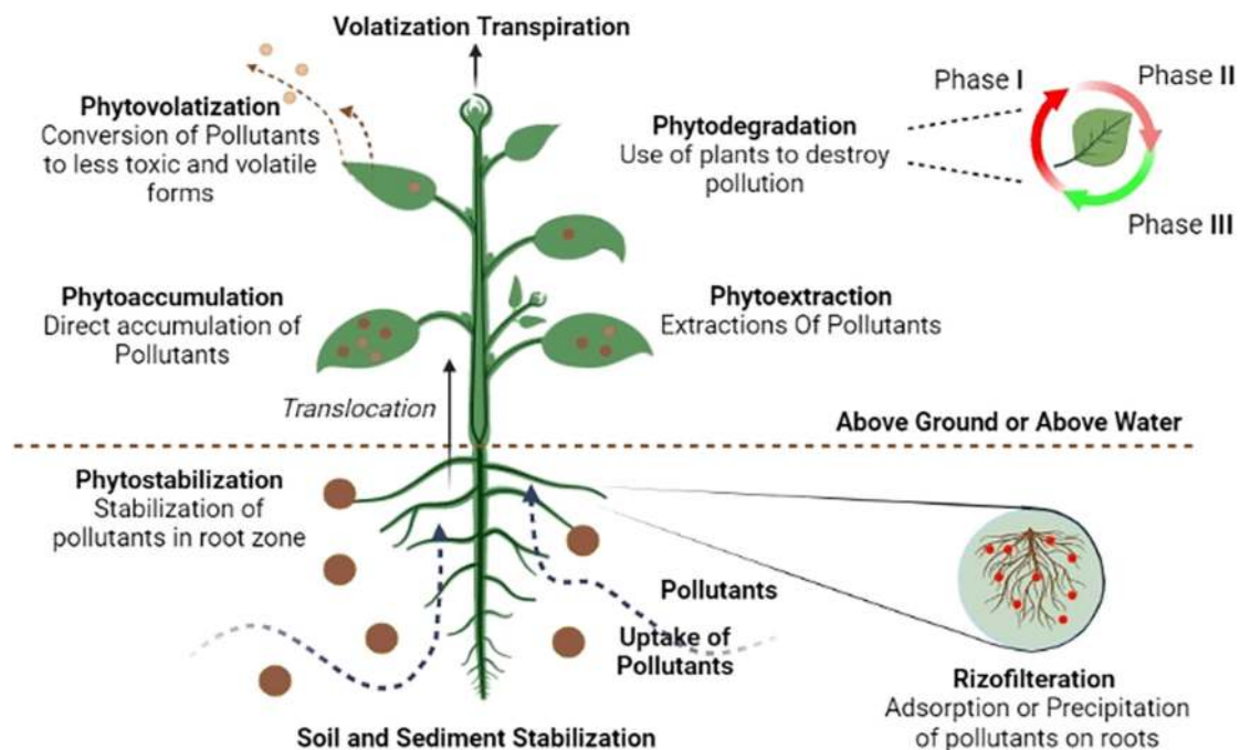
Figure 9.1 Mechanisms of phytoremediation.
