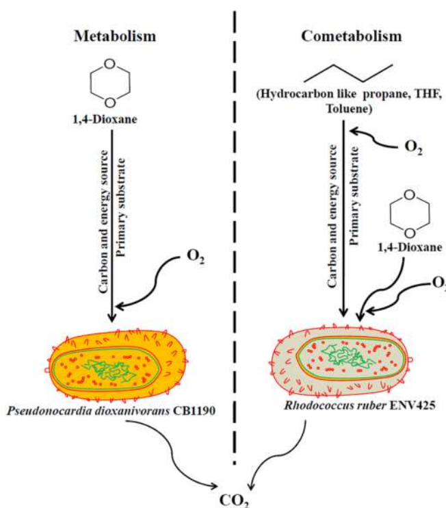
Figure 12.3 Simple illustration of microbial metabolism and co-metabolism of 1,4-dioxane.
