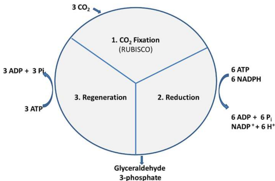
Figure 4.3 CB cycle-mediated biological CO 2 fixation.
