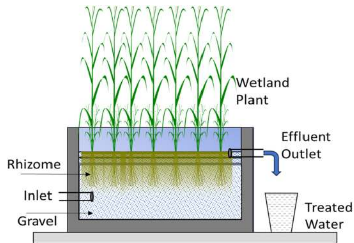
Figure 16.5 Schematic representation of constructed wetland system for wastewater treatment.
