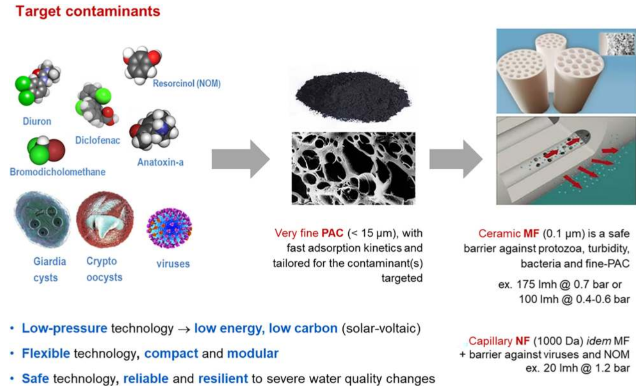
Figure 8.12 Hybrid adsorption/membrane process.
