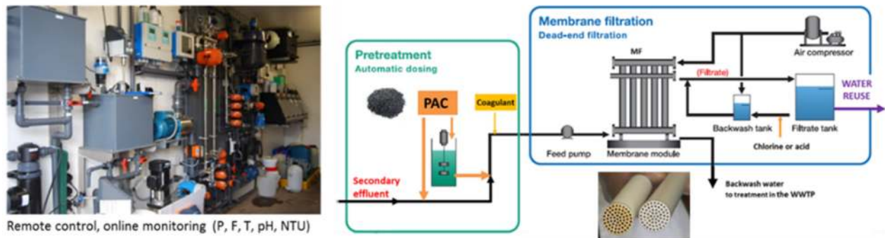
Pilot. PAC / (C)/MF, ceramic 0.8 m 2 , 0.1 μm, dead-end constant flux at BEI WWTP (Viegas et al. 2020a)
