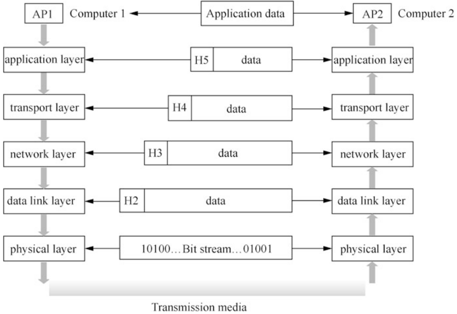
Fig. 4.7 Data transfer process between various layers of the network
