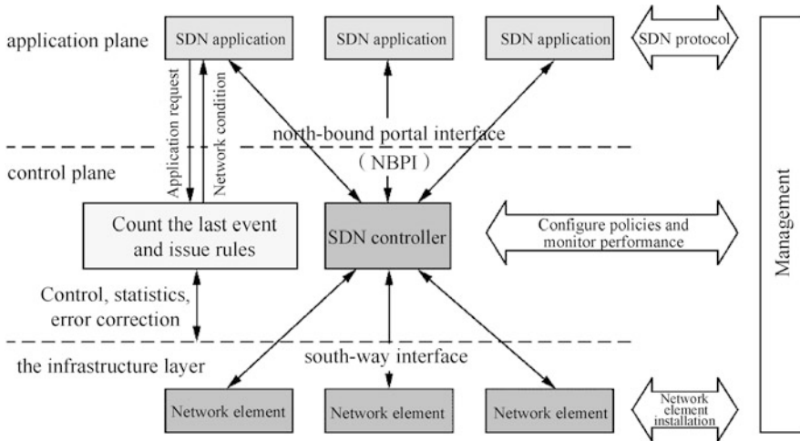
Fig. 4.23 SDN architecture
