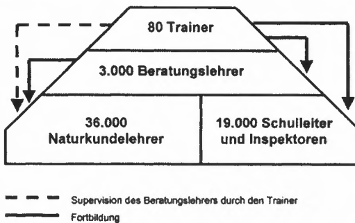
Abb. 2: SEQIP-Trainingskaskade
