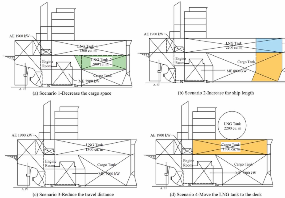
Figure 11. Design scenario layouts Adapted from the reference design in MEPC (2018)
