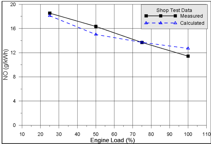
Figure 7. Calculated and measured NO_x specific emissions comparison, reference measurements
