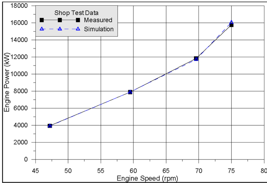
Figure 5. Calculated and measured power comparison, reference measurements
