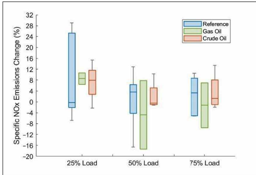
Figure 11. Specific NO_x emissions comparison, B30: Reference, gas oil, crude oil
