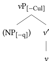
Figure 2: Non-culminative vP
