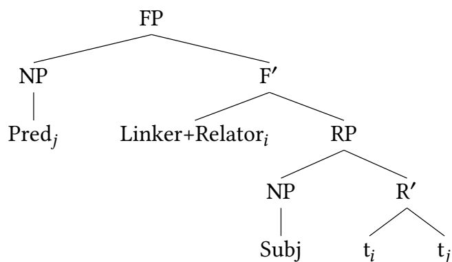
Figure 2: Comparative QBNPs
