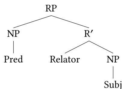
Figure 1: Attributive QBNPs
