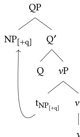
Figure 3: QP
