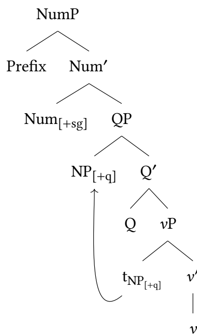
Figure 6: Singular NumP
