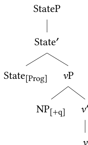
Figure 5: StateP
