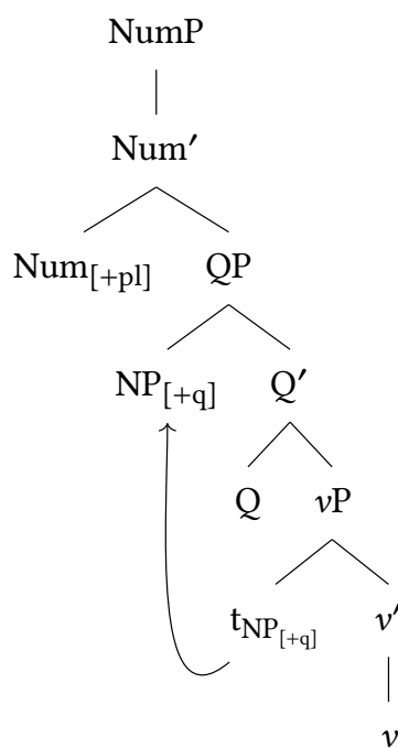
Figure 4: Plural NumP
