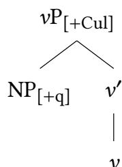
Figure 1: Culminative vP
