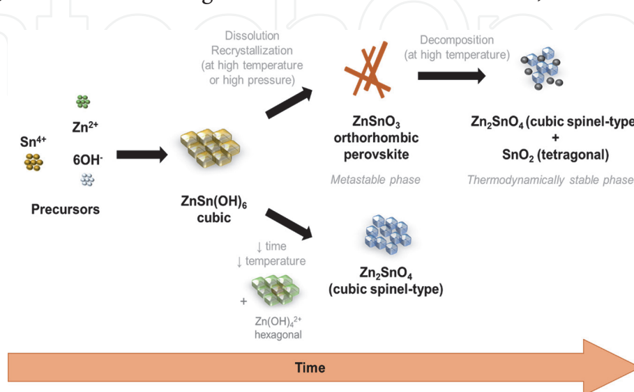
Figure 3. Schematic of the growth mechanism of ZTO nanostructures ( \text{ZnSnO}_3 nanowires and \text{Zn}_2\text{SnO}_4 nanoparticles) on a hydrothermal synthesis as a function of the energy available and the duration of the synthesis. From reference [43].
