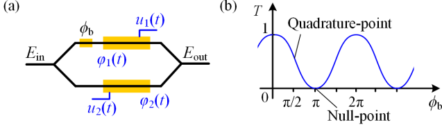
Figure 2.1: Schematic and characteristics of an electro-optic Mach-Zehnder modulator (MZM). (a) Schematic of a MZM where the incoming light E_{\text{in}} is split in two arms, each of which contains a phase modulator. The top MZM arm has an additional bias phase \phi_b that defines the operating point of the MZM by adjusting the relative phase difference between the two MZM arms. Two RF modulating signals u_1(t) and u_2(t) in the upper and lower arm of the MZM result in a modulation of \phi_1(t) and \phi_2(t) , respectively. After modulation, the light from the two arms is coherently combined at the output E_{\text{out}} of the MZM. (b) Intensity transfer function T of a push-pull MZM as a function of the relative bias phase \phi_b between the phase modulating arms. A relative phase difference \phi_b = \pi/2 results in a quadrature operating point of the MZM, where the intensity modulation varies linearly for a small RF modulation signal. For \phi_b = \pi , the MZM is said to be operating at its null-point where the optical carrier is suppressed.
