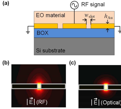
Figure 2.7: Plasmonic-organic hybrid modulator. (a) Cross-section of POH Mach-Zehnder modulator (MZM) on the SOI platform. Each MZM arm consists of a plasmonic slot waveguide of width w_{\text{slot}} formed by the gold strips. The slots are filled with an organic EO material and the chromophores are aligned in a poling process, see Sec 2.2.1. An RF signal applied to the gold electrodes drops in the slot and modulates the plasmonic mode propagating through it. (b) Plot of the electric field profile of the RF modulation field tightly confined to the plasmonic slot. (c) Plot of the field profile of the symmetric optical mode that propagates through plasmonic slot waveguide. A high overlap between the optical and the RF fields results in a high efficiency of the POH modulators.
