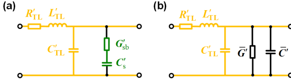
Figure 2.4: Equivalent-circuit models for estimation of EO bandwidth of RC-SOH MZM. All elements represent lumped differential quantities. (a) Equivalent-circuit of an infinitesimally short element of the transmission line formed by RC-SOH MZM. The differential elements R'_{TL} , L'_{TL} and C'_{TL} (yellow) correspond to the metal transmission line. The differential elements G'_{sb} and C'_s (green) represent the RC shunt load formed by the doped-Si slab and the Si slot waveguide respectively. (b) Telegrapher-type equivalent-circuit representation of an MZM transmission-line element. The equivalent-circuit of RC-SOH MZM shown in (a) is transformed into a telegrapher-type model using a frequency-dependent differential shunt conductance \bar{G}' and a frequency-dependent differential shunt capacitance \bar{C}' .
