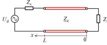
Figure B.6: Equivalent-circuit model for a traveling-wave modulator having a length L and a complex line impedance \underline{Z}_c . The device is driven by an RF source with an internal impedance Z_s and a voltage amplitude U_d . Z_t denotes the termination impedance.
