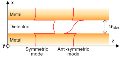
Figure 2.6: Schematic showing a plasmonic slot waveguide with the dielectric and the metal electrodes infinitely extending in z - and y - direction. The plot shows the electric E_x -field of the symmetric and anti-symmetric modes that can propagate in the metal-insulator-metal (MIM) slot waveguide.
