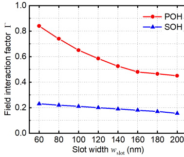
Figure 2.8: Field interaction factor \Gamma of the optical mode with the EO cladding material in the slot region as a function of slot width w_{\text{slot}} for both POH and SOH waveguides at a wavelength of 1550 nm. For the SOH modulator, a slot waveguide having a height of 220 nm, a Si rail width of 240 nm and a Si slab of 70 nm are chosen for the calculations. The POH devices considered for the calculations have a gold thickness of 150 nm. In general, POH devices feature a 2.5 – 3.5 times larger field interaction factor than SOH devices due to the tight confinement of the plasmonic mode to the slot region and due to a reduced group velocity of the plasmonic slot mode. Figure and caption adapted from [36].
