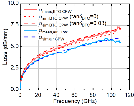
Figure B.4: Measured (solid lines) and simulated (dashed lines) microwave propagation loss \alpha_{\text{air CPW}} ( \alpha_{\text{BTO CPW}} ) of the air-filled (BTO-filled) CPW. The measured and simulated loss assuming a loss tangent \tan \delta_{\text{BTO}} = 0 and \tan \delta_{\text{BTO}} = 0.03 for the 150-nm-thick amorphous BTO film. We determine an upper limit for the BTO loss tangent to be 0.03.
