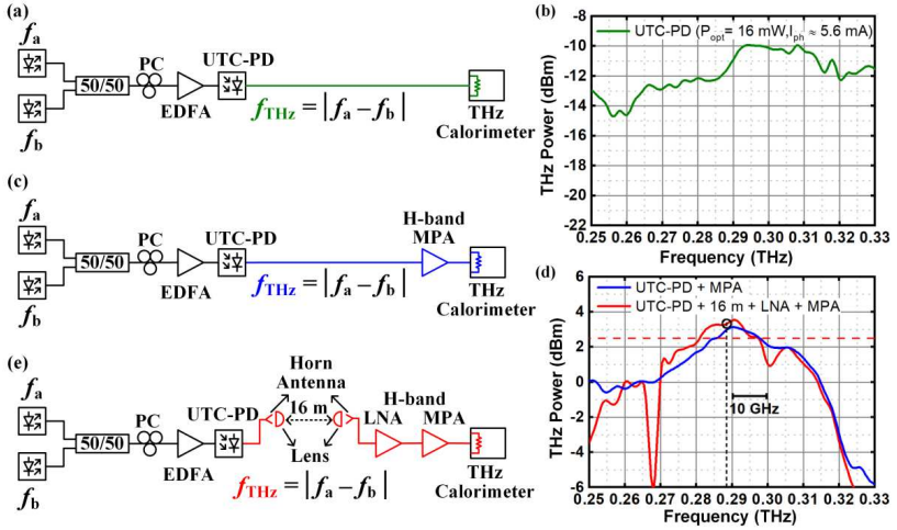
Figure A.6: Setup for characterizing various THz components used in the data transmission experiment. For all the measurements, the optical input power to the uni-travelling-carrier photodiode (UTC-PD) is set to P_{\text{opt}} = 16 \text{ mW} which corresponds to a direct photocurrent of I_{\text{ph}} = 5.6 \text{ mA} . (a) Setup for measuring the THz output power of the UTC-PD (b) Frequency-dependent THz power of UTC-PD as measured by calorimeter (c) Setup for measuring the available THz power after amplification by H-band medium-power amplifier (MPA). (d) Frequency-dependent THz power for the combination of UTC-PD and MPA (blue curve). (e) Setup for measuring the THz power available after a free-space transmission distance of 16 m and a cascaded amplification stage, comprising a low-noise amplifier (LNA) and the MPA. The available THz power as a function of frequency is shown as the red curve in (d). The kinks in the red curve are attributed to imperfect waveguide connector flanges. A horizontal red dashed line indicates a minimum THz power of 2.5 dBm that was needed at 20 Gbd to achieve a BER of 4.5 \times 10^{-3} , corresponding to the threshold for forward-error correction (FEC) with 7% coding overhead, see Fig. 3.2(d) in the Chapter 3. The operating frequency of the THz communication link for the data transmission experiments is marked with a circle and a vertical line.
