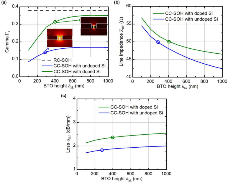
Figure B.10: Impact of BTO slab height h_{hk} on the field interaction factor \Gamma_s , line impedance Z_{RF} and RF loss \alpha_{RF} for CC-SOH modulator with pure dielectric Si rails and doped ( \rho = 5.5 \times 10^{-4} \Omega\text{m} ) Si rails having w_{hk} = 1 \mu\text{m} , w_{sig} = 4 \mu\text{m} , and a metal thickness of 600 nm. (a) Field interaction factor \Gamma_s of CC-SOH modulator as a function of BTO slab height h_{hk} . As a comparison, the field interaction factor of RC-SOH modulator, \Gamma_{RC-SOH} \approx 0.38 is shown in black trace. Inset shows RF field profiles of CC-SOH devices with undoped and slightly doped Si rails at positions marked by the respectively colored circles. (b) Line impedance Z_{RF} of CC-SOH modulator for different slab heights. (c) RF propagation loss \alpha_{RF} of CC-SOH modulator with and without doped Si rails for different BTO slab heights. The respective designs with doped and undoped Si rails having a good match to 50 \Omega source impedance are marked in colored circles.
