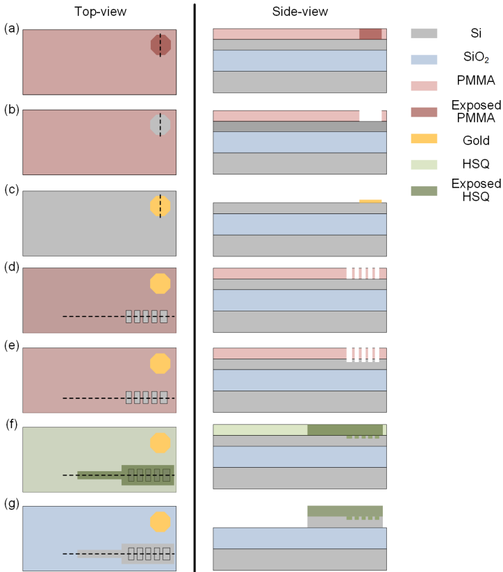
Figure 2.12: Fabrication process flow for passive silicon structures on SOI substrates. The cross-section shown in the side-view corresponds to the dashed line shown in the top-view. (a) Patterning of octagonal marker into the PMMA resist. (b) Development of PMMA resist to reveal the silicon device layer in the exposed regions. (c) Evaporation of gold onto the PMMA mask followed by the stripping of the resist. The steps from (a) – (c) form the so-called ‘lift-off’ process. (d) Patterning and development of PMMA resist to create a mask for shallow-etch of silicon, e.g., for shallow-etched grating couplers. (e) Reactive-ion-etching of silicon to fabricate shallow-etch structures followed by stripping of the PMMA resist. (f) Patterning and development of the HSQ resist for fully-etched structures in silicon. (g) Reactive-ion-etching of silicon to realize fully etched structures.
