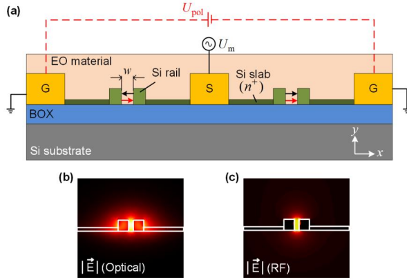
Figure 2.3: Resistively-coupled silicon-organic hybrid (RC-SOH) modulator. (a) Cross-section of RC-SOH Mach-Zehnder modulator (MZM) on the silicon-on-insulator platform. The slot waveguide consists of two silicon rails separated by a slot of width w . The slot waveguide is electrically connected to the RF transmission line arranged in ground-signal-ground (GSG) configuration via thin lightly doped silicon slabs. The upper cladding is formed by the organic electro-optic (EO) material which also fills the slot. The chromophores of the EO material are aligned (depicted along the red arrows) in a poling process, where a poling voltage U_{pol} (in red) is applied across the floating ground terminals at elevated temperatures. After cooling down and removing the voltage, the chromophores are locked in this orientation. An RF modulating signal U_m applied to the GSG terminals of the RC-SOH MZM drops predominantly in the slot. The modulating electric field (depicted along the black arrows) is oriented parallel to orientation of the EO chromophores in one arm, and is anti-parallel in the other arm, thus resulting in a push-pull operation of the MZM. (b) Plot of the field profile of the quasi-TE optical mode that is confined to the silicon slot waveguide. The discontinuity at the interface between silicon and the organic material leads to an enhancement of the electric field in the slot. (c) Plot of the field profile of the RF modulation signal. An RF voltage applied across the transmission line drops predominantly in the slot region leading to a large overlap between the optical and the RF fields.
