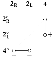
Fig. 13.1 The Krajewski diagram for the finite real spectral triple (A^{\text{ev}} = \mathbb{H}_R \oplus \mathbb{H}_L \oplus M_4(\mathbb{C}), H_F, D_F; J_F, \gamma_F) . The dashed line corresponds to an ‘off-diagonal’ component of the Dirac operator, thus failing on the first-order condition. The labels + and – represent the value of the grading \gamma_F on the corresponding summands of H_F
