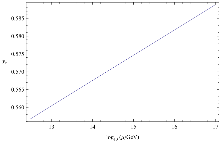
Fig. 14.4 The running of the tau-neutrino Yukawa coupling y_\nu for \Lambda_{GUT} = 9.92 \times 10^{16} GeV, \rho = 1.2 , and m_R = 3 \times 10^{12} GeV
