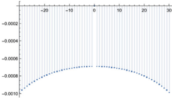
(c) Summands in (16.2.7) for (\lambda_i, \lambda_j) = (0, 0)
