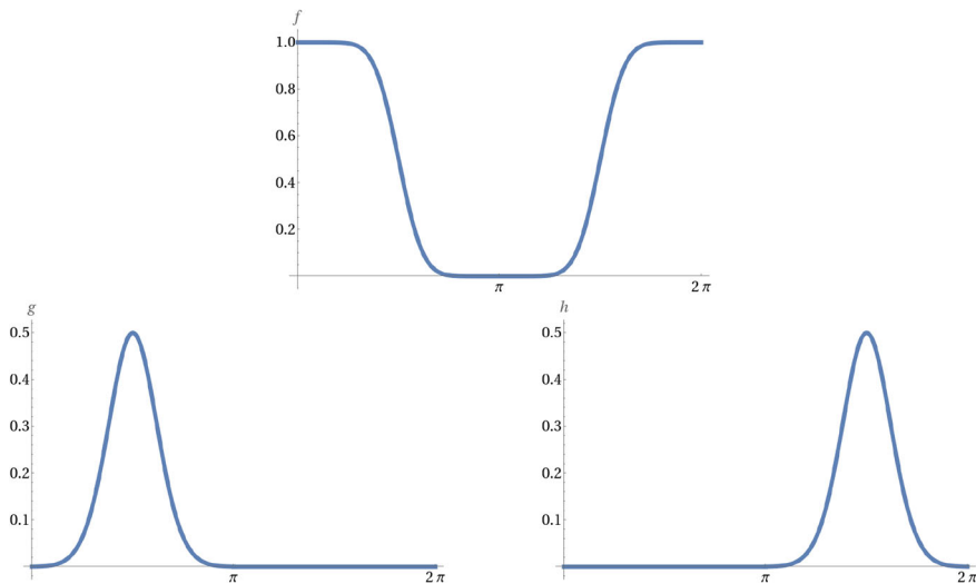
Fig. 6.2 Functions f, g, h that ensure that p in (6.1.1) is a projection
