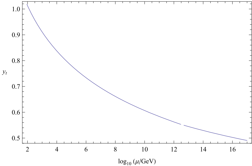
Fig. 14.3 The running of the top-quark Yukawa coupling y_{\text{top}} for \Lambda_{GUT} = 9.92 \times 10^{16} GeV, \rho = 1.2 , and m_R = 3 \times 10^{12} GeV
