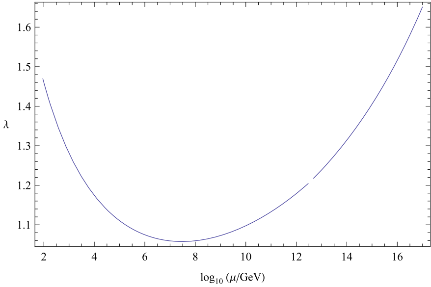
Fig. 14.2 The running of the quartic Higgs coupling \lambda for \Lambda_{GUT} = 9.92 \times 10^{16} GeV, \rho = 1.2 , and m_R = 3 \times 10^{12} GeV
