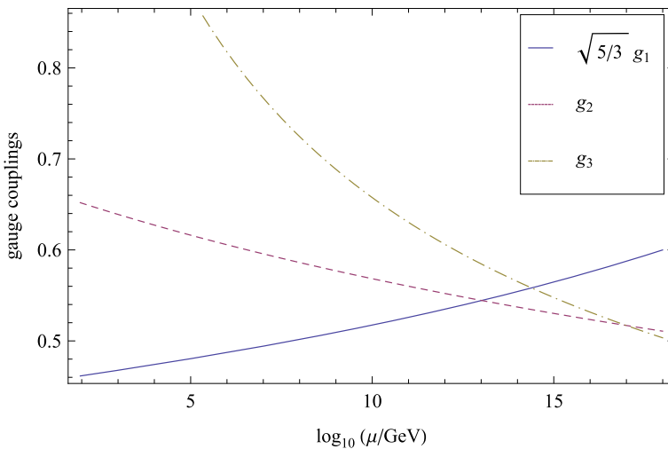
Fig. 14.1 The running of the gauge coupling constants
