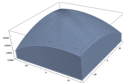
(b) The divided difference f'[\lambda_k, \lambda_l] for this function f .
