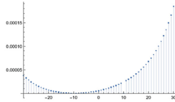
(b) Summands in (16.2.6) for (\lambda_i, \lambda_j) = (10, 0)
