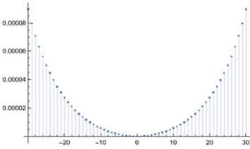
(a) Summands in (16.2.6) for (\lambda_i, \lambda_j) = (0, 0)
