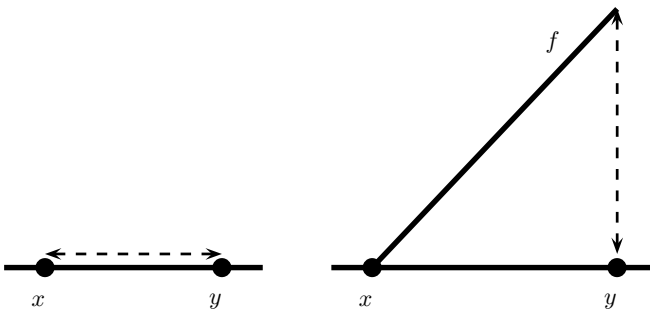
Fig. 5.1 The translation of the distance between points x, y in M to a formulation in terms of functions of slope \leq 1
