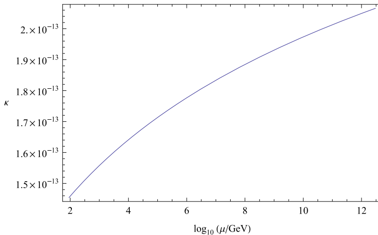
Fig. 14.5 The running of the effective coupling \kappa for \Lambda_{GUT} = 9.92 \times 10^{16} GeV, \rho = 1.2 , and m_R = 3 \times 10^{12} GeV
