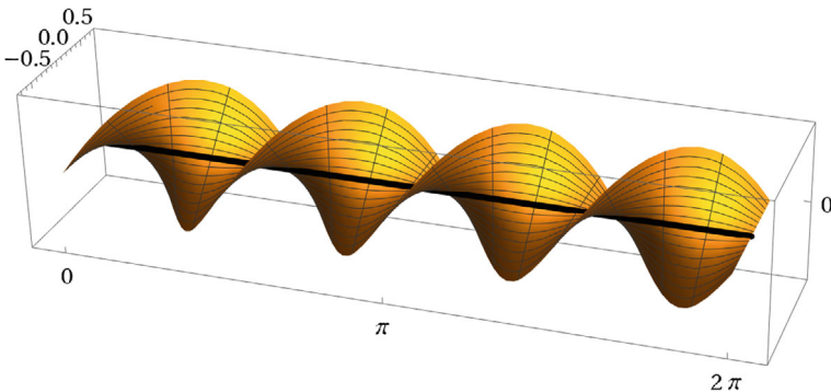
Fig. 6.3 Winding twice around one of the circle directions on the torus. Let the range of the projection p be v(t_1, t_2)s with s \in \mathbb{C} and v(t_1, t_2) \in \mathbb{C}^2 varies with (t_1, t_2) \in \mathbb{T}^2 . We have drawn the real and imaginary parts of the first component v_1(t_1 = 3\pi/4, t_2)s with 0 \leq t_2 \leq 2\pi and -1 \leq s \leq 1 . The other component v_2(t_1 = 3\pi/4, t_2) is constant
