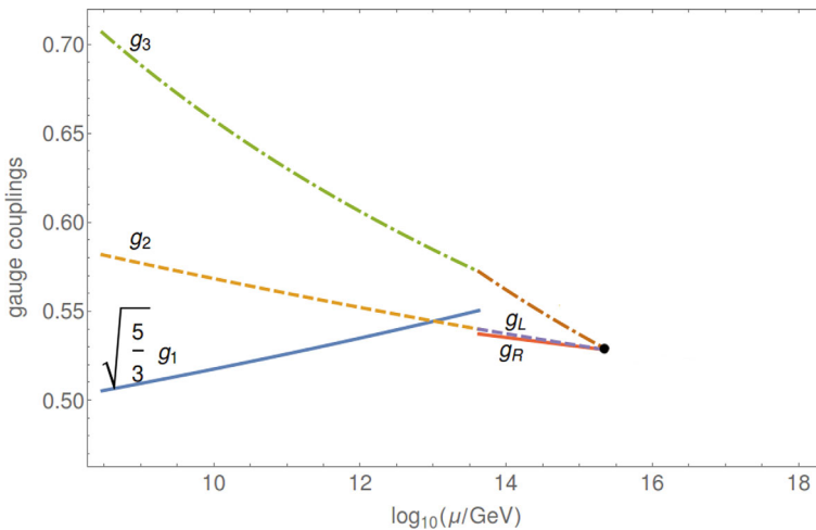
Fig. 15.1 Running of coupling constants for the spectral Pati-Salam model with composite Higgs fields: g_1, g_2, g_3 for \mu < m_R and g_R, g_L, g for \mu > m_R with unification scale \Lambda \approx 2.5 \times 10^{15} GeV for m_R = 4.25 \times 10^{13} GeV
