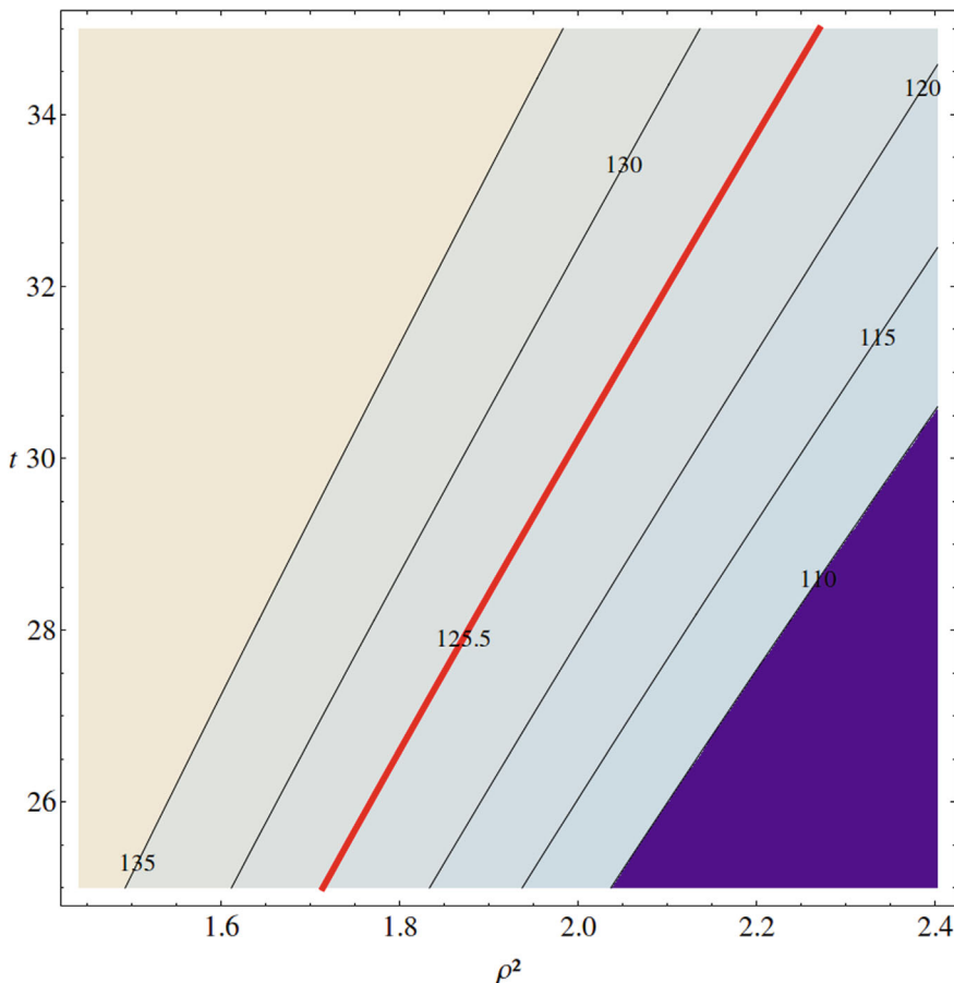
Fig. 15.2 A contour plot of the Higgs mass m_h as a function of \rho^2 and t = \log(\Lambda_{GUT}/M_Z) . The red line corresponds to m_h = 125.5 GeV
