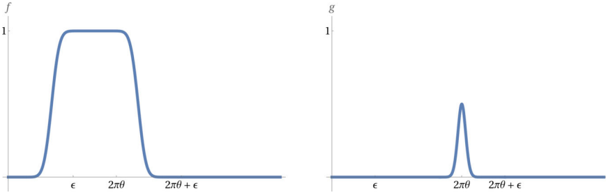
Fig. 6.4 Functions f and g = h^* that ensure that p defined in (6.2.1) is a projection in \mathcal{A}_\theta
