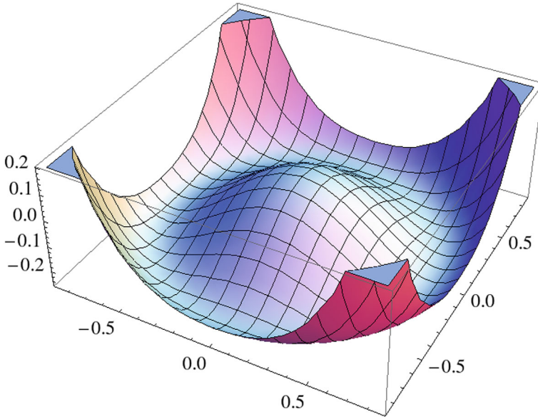
Fig. 13.3 The potential \mathcal{L}_{\text{pot}}(H) of (13.3.8) with 2af_2\Lambda^2 > ef(0)
