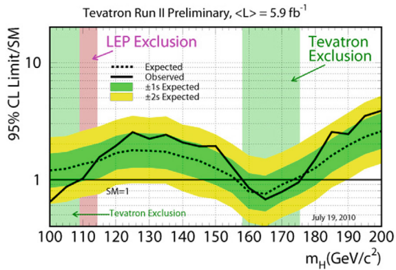
Fig. 14.6 Observed and expected exclusion limits for a Standard Model Higgs boson at the 95-percent confidence level for the combined CDF and DZero analyses. (Fermilab)
