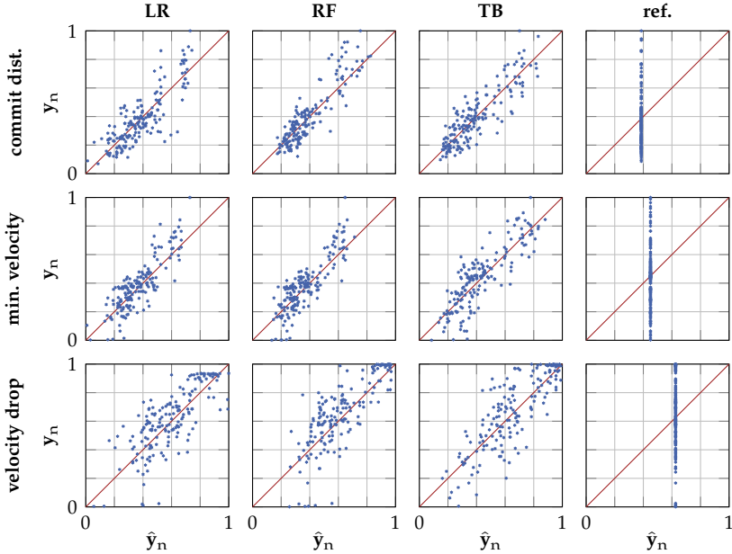
Figure 2.4 Scatter plots of the behavior prediction at the X-intersections with the full feature set. All three behavior features are used as labels and LR, RF and TB are used for regression. For comparison, the regression with the naive reference is also given. The true labels y_n and estimated labels \hat{y}_n are normalized to the maximum value of each individual regression.
