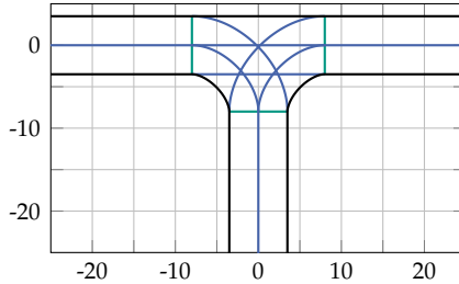
Figure 4.2 Generic map of a T-intersection that is used for simulation. The map is made up of lanelets, the inner borders of those are marked in blue and green. All dimensions are in meters. For simulation purposes the parts of the streets leading into the intersection are extended further out as a straight street, which is only shown in part here.
