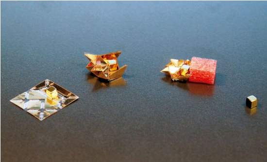
Self folding origami robots, Photo credit: CSAIL. Reference: https://danielarus.csail.mit.edu/index.php/2015/09/lorem-ipsum-2/
