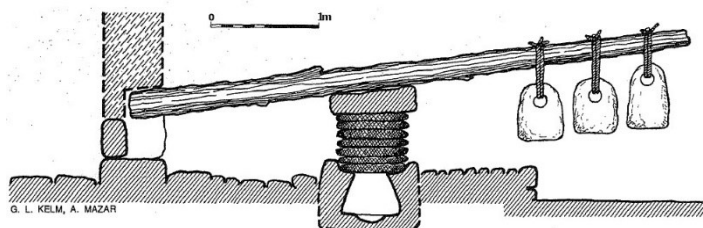
Figure 2: Simple lever-and-screw weights olive press, used in Tel Baṭaṣh (biblical Timna) during the Iron Age (Frankel 1994, 39)
