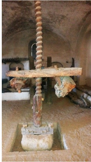
Figures 7a and 7b: Close-up photos of the screw weight-stone in MUSA, the Eretz Israel Museum, Tel-Aviv (images: Dr Etan Ayalon)
