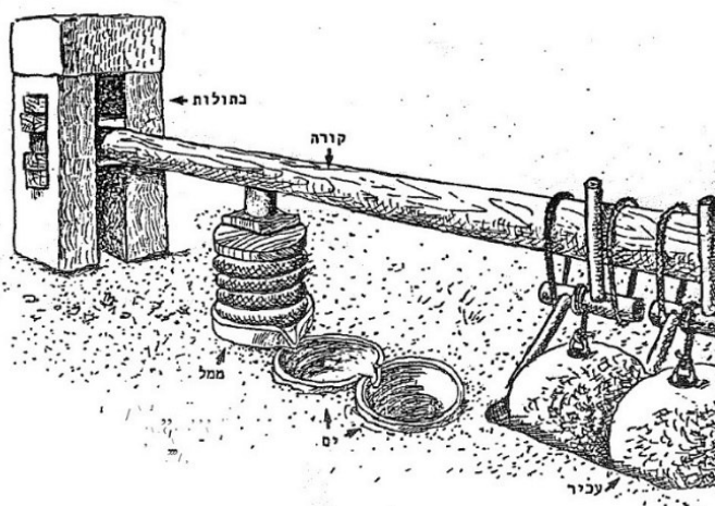
Figure 3: Parts of a press in m. Bava Batra 4.5, according to Frankel (1986, 59)
