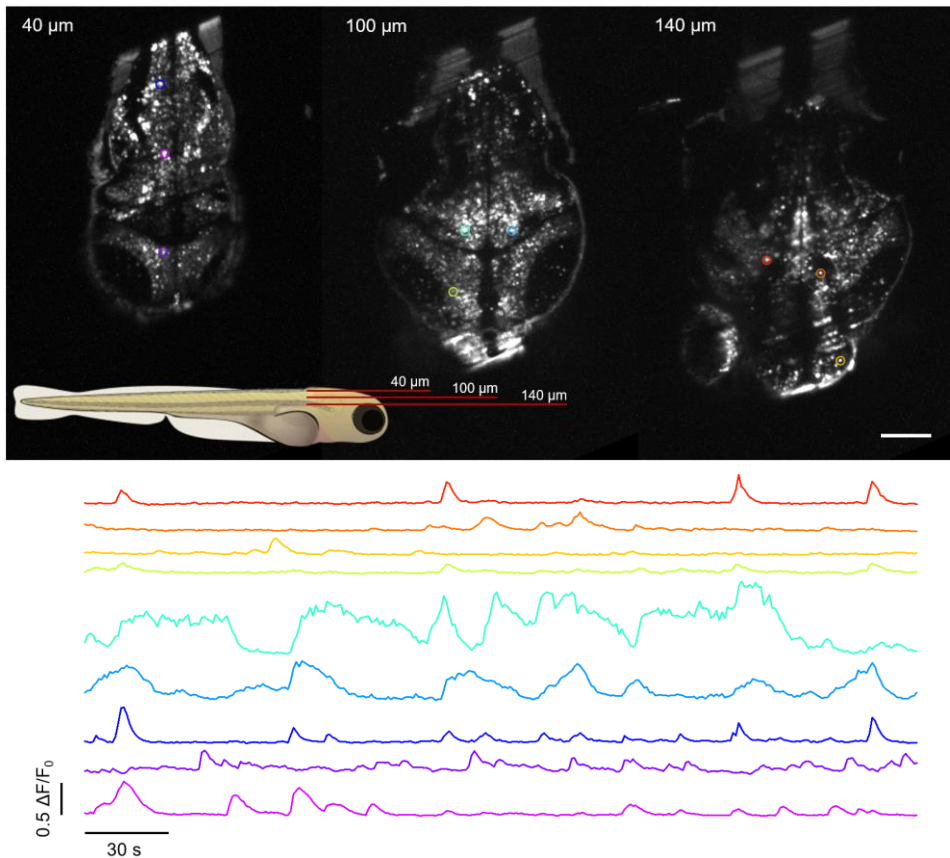
Figure 51. Real-time whole-brain neuronal activity recording by 2P-LSFM.
