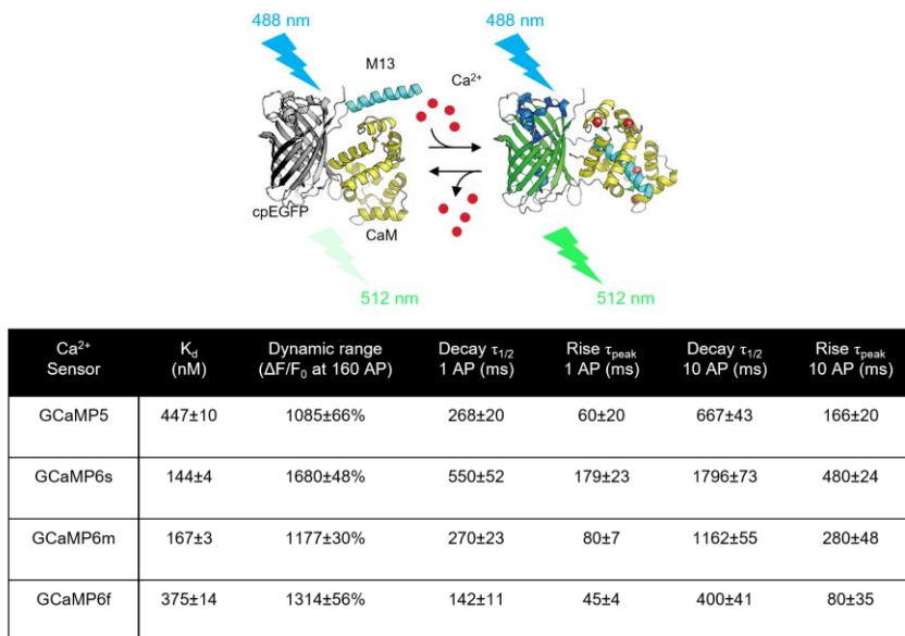
Figure 10. GCaMP structure and kinetic features.
