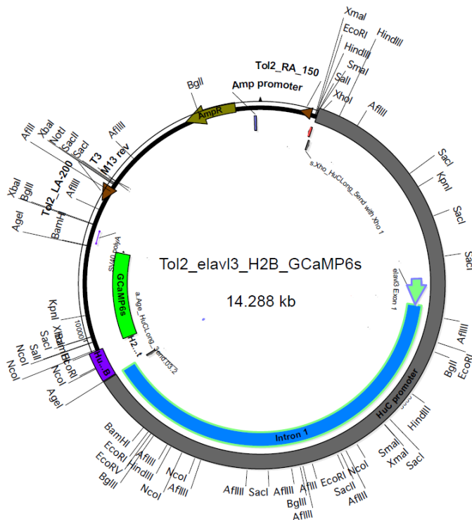
Figure 22. Map of the tol2-elavl3:H2B-GCaMP6s plasmid.
