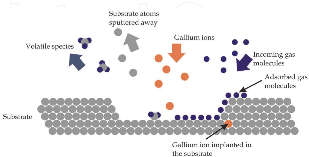
Fig. 5. Schematic describing atomic processes during ion beam-promoted sputtering.
