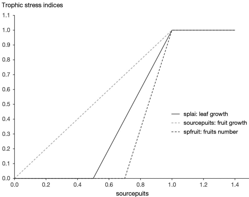
Figure 4.15. Trophic stress indices ( sourcepuits , splai , spfruit ) as a function of the source/sink ratio (sourcepuits). Parameters splaimin_p = 0.5 , splaimax_p = 1 , spfrmin_p = 0.7 and spfrmax_p = 1 .
