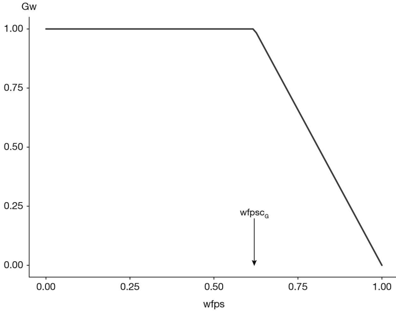
Figure 12.19. Effect of water-filled pore space on the proportion of N_2O emitted by denitrification. Parameter: wfpSC_a = 0.62 .
