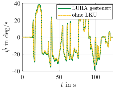
(c) Gierrate \dot{\psi} .
