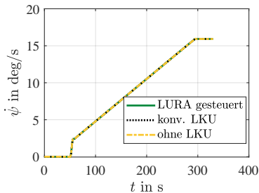
(c) Gierrate \psi .
