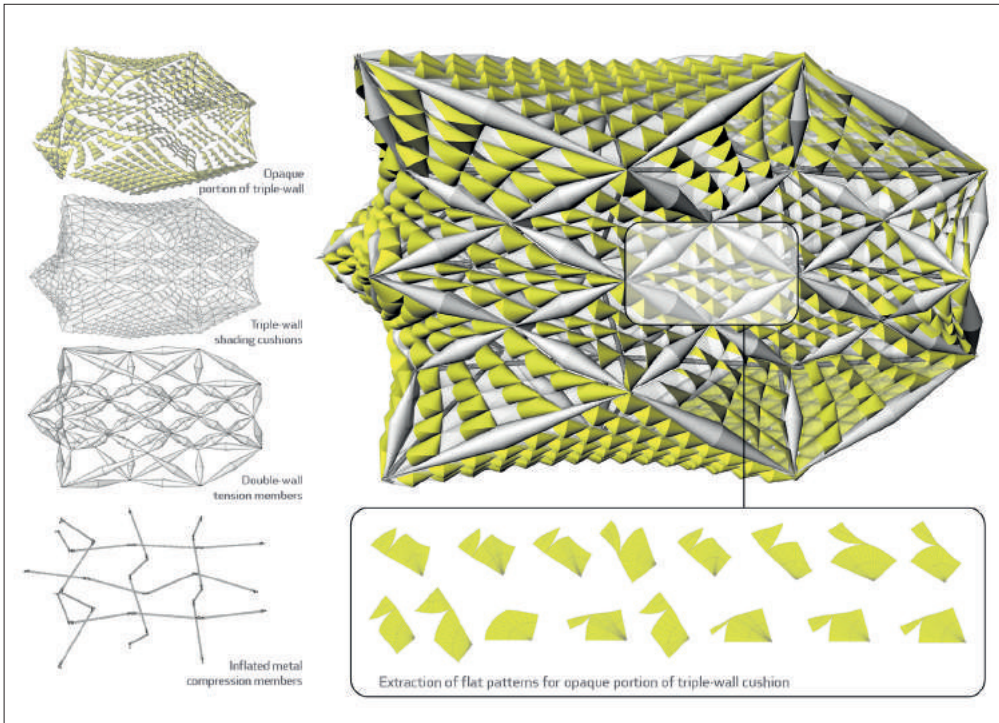
Fig. 12: Study of the proposed system elements and extracted flat-pattern data for the opaque portion of the triple-wall cushions.
