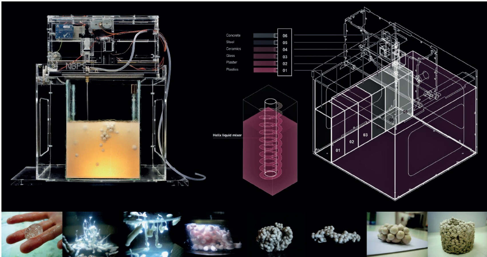
Fig. 7: NGPS Project, developed by Ali Basbous, Miquel Lloveras. FABbots 1.0, IaaC, 2010. Left: Machine prototype with filled tank. (Photo: Diaz Wichmann Photography.) Right: Machine diagram showing multi-material capabilities. (Image: NGPS team.) Bottom: Material spherification samples. (Photos: Miquel Lloveras.)
