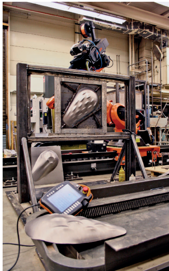
Fig. 4: (left) Forming a singular valley. (right) Multiple valleys in one panel.
