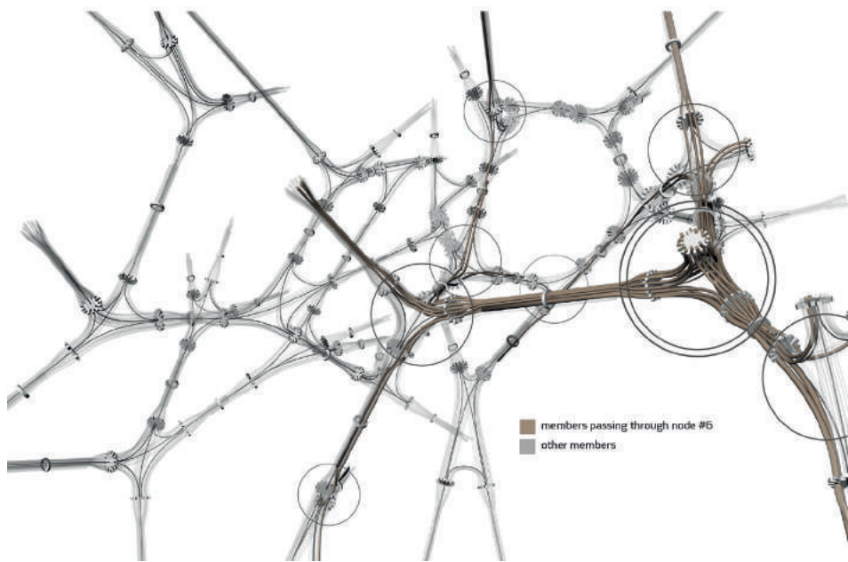
Fig. 14: Member continuity through multiple connection nodes, as demonstrated by identifying all the members that pass through node #6.
