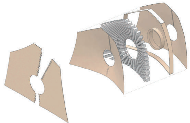
Fig. 6: Exploded axonometric view of the module layers.
