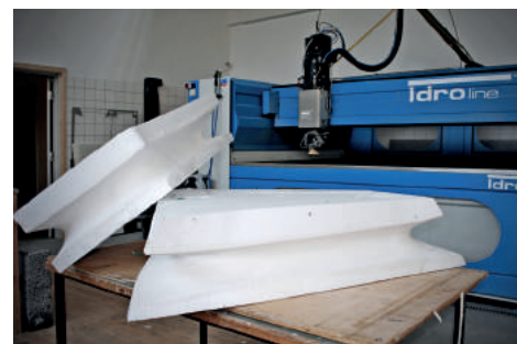
Fig. 8: Opticut sample moulds.
