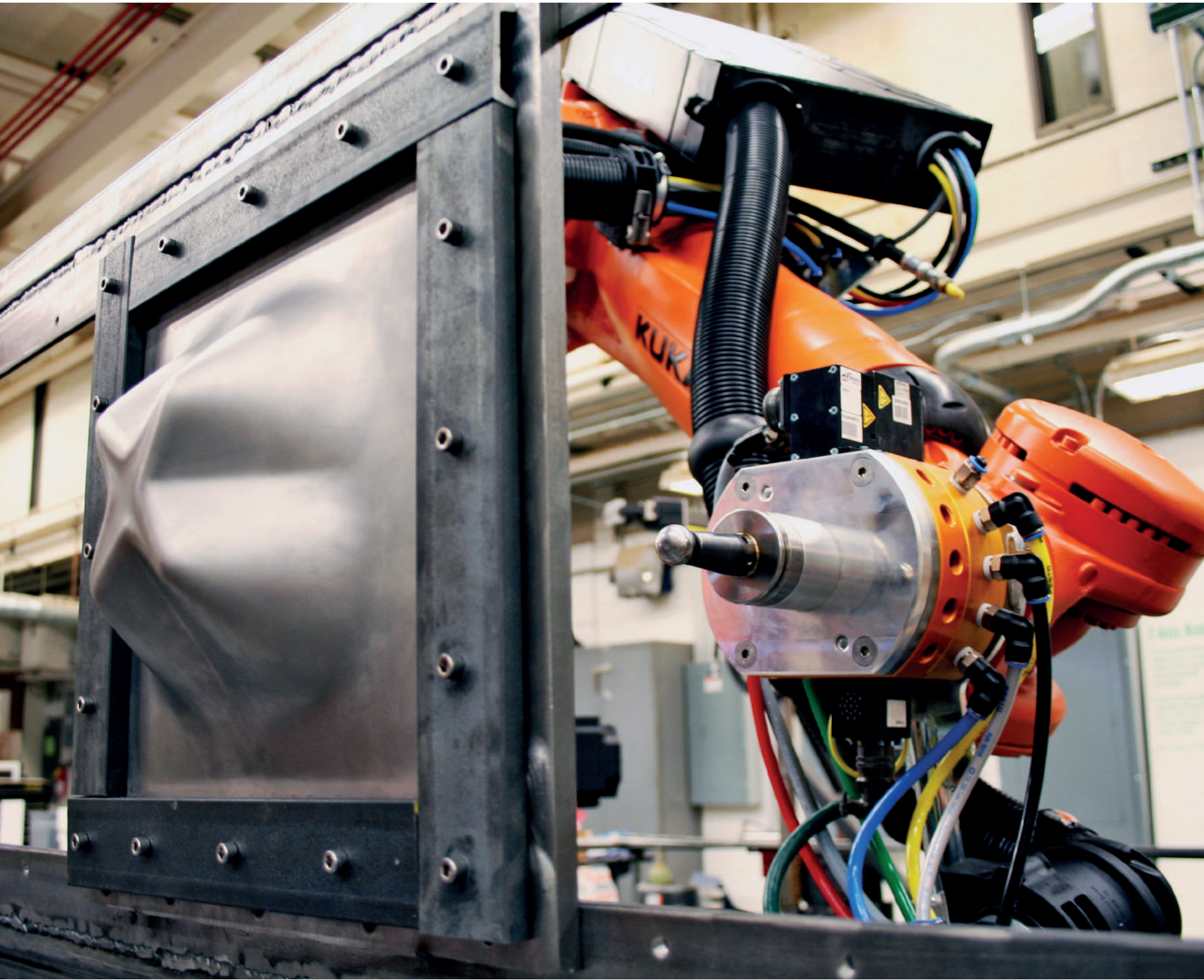
Fig.1: Custom forming tool mounted on the six-axis robotic arm.
