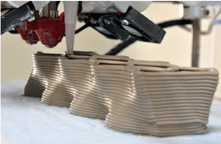
Fig. 3: 3D printing bricks with a liquid ceramic mixture on a modified desktop 3D printer.
