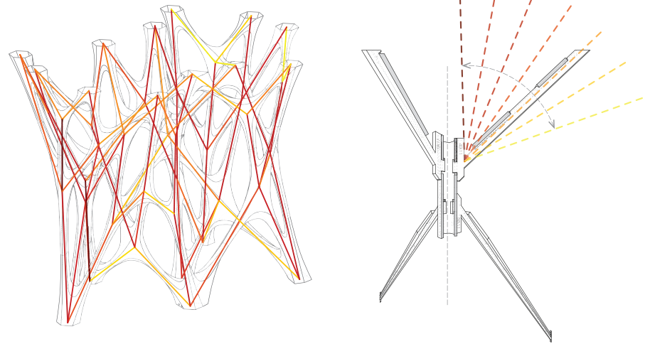
Fig. 5: Steel assembly diagrams: variety of vertical steel connection angles, range of vertical angles accommodated by steel pipe detail.
