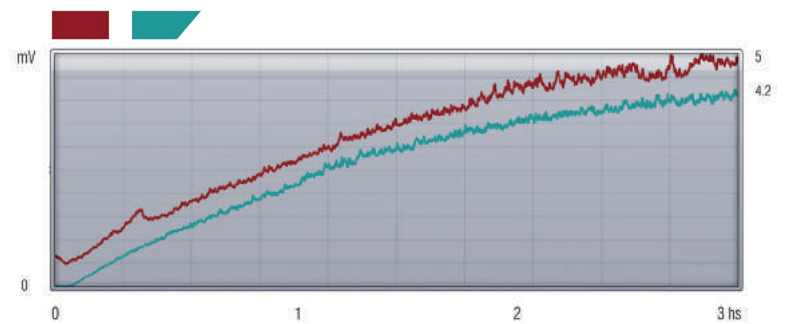
Fig. 10: Heat flux results from the physical test.
