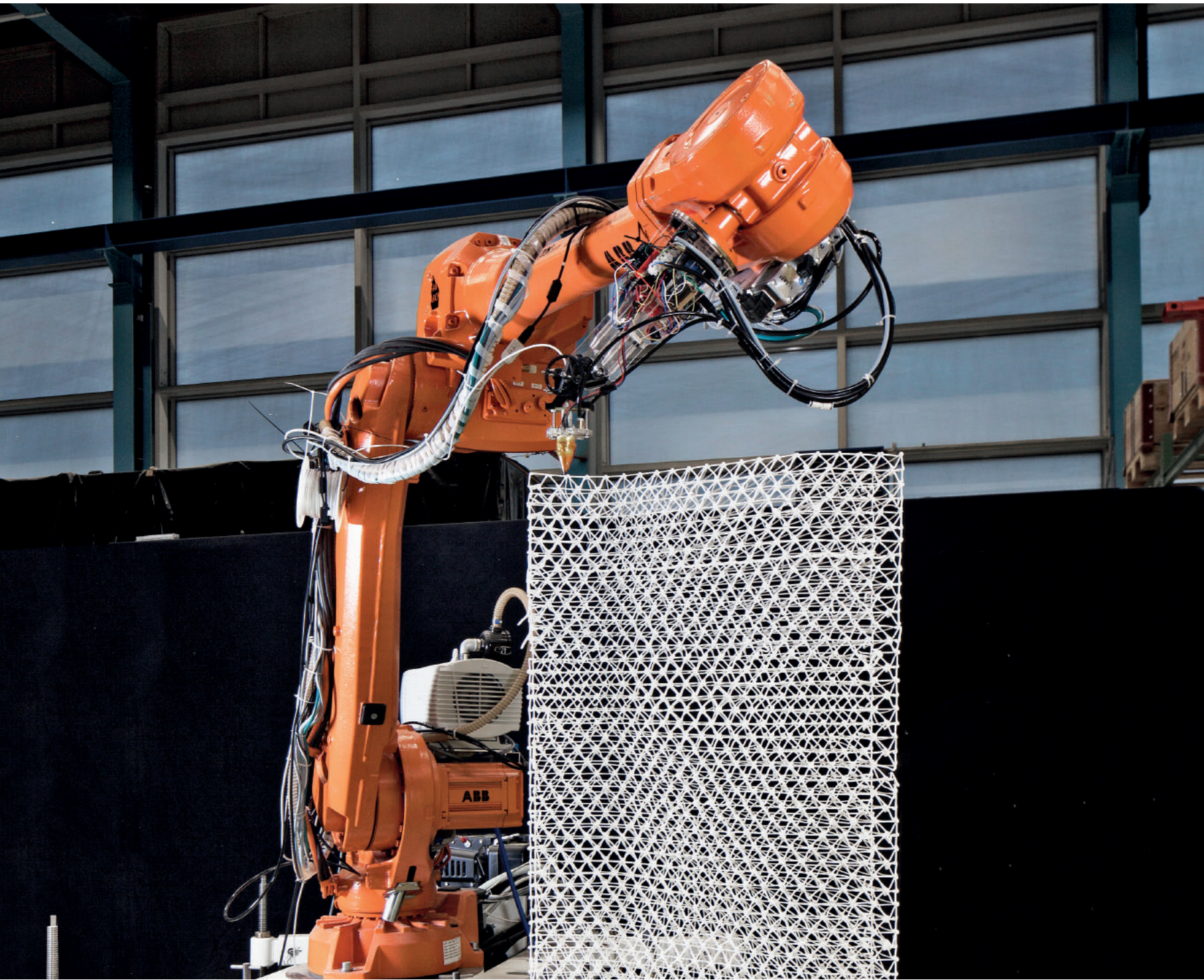
Fig.1: Large prototype extruded with the mobile robot.
