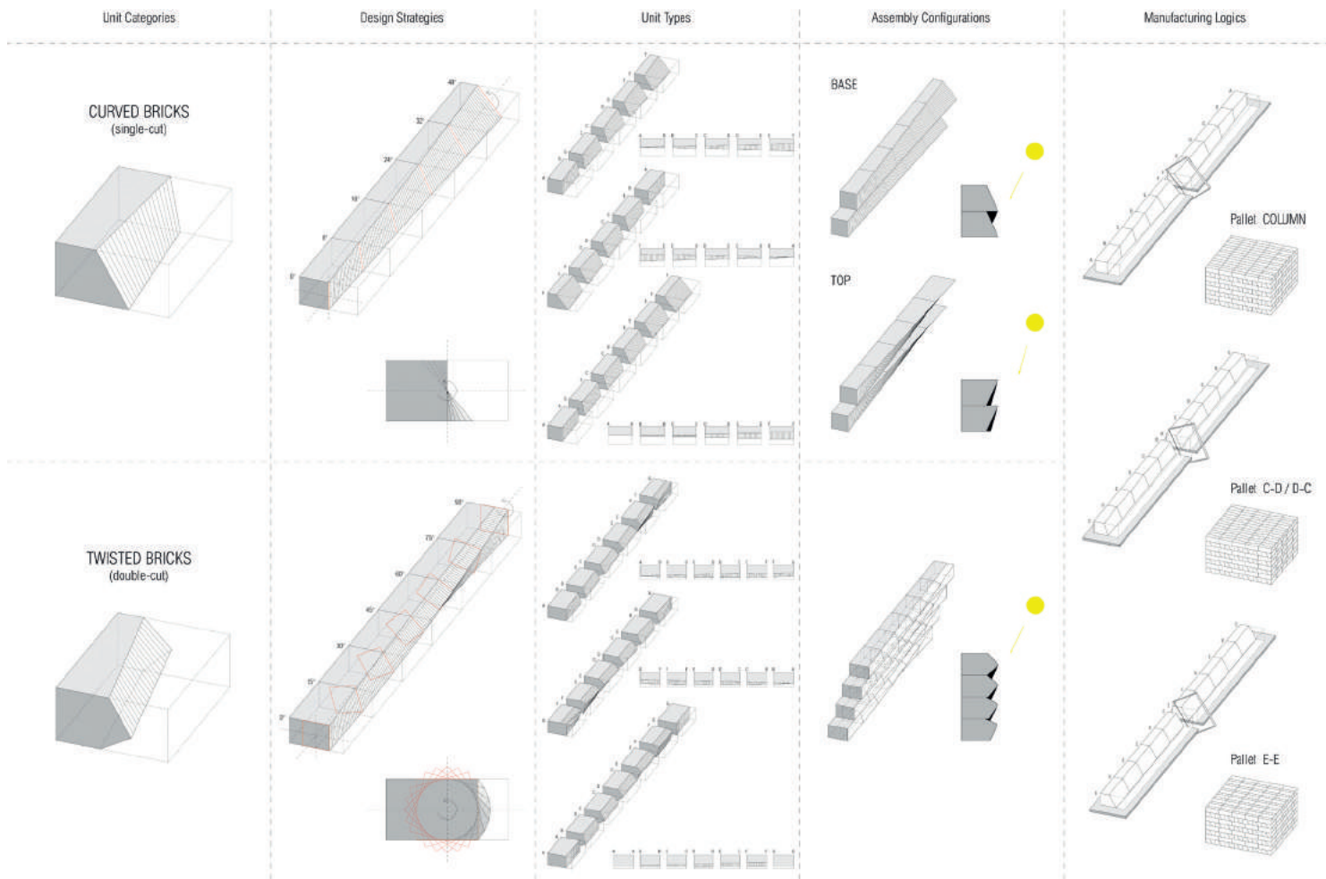
Fig. 5: Strategically customised ruled-surface unit typologies.
