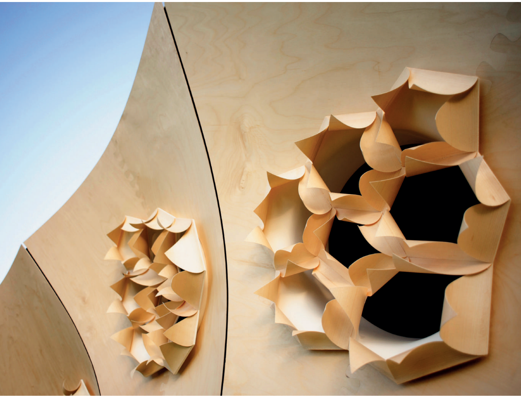
Fig. 1: Close-up photo of the HygroSkin – Meteorosensitive Pavilion (low relative humidity, 45%).
