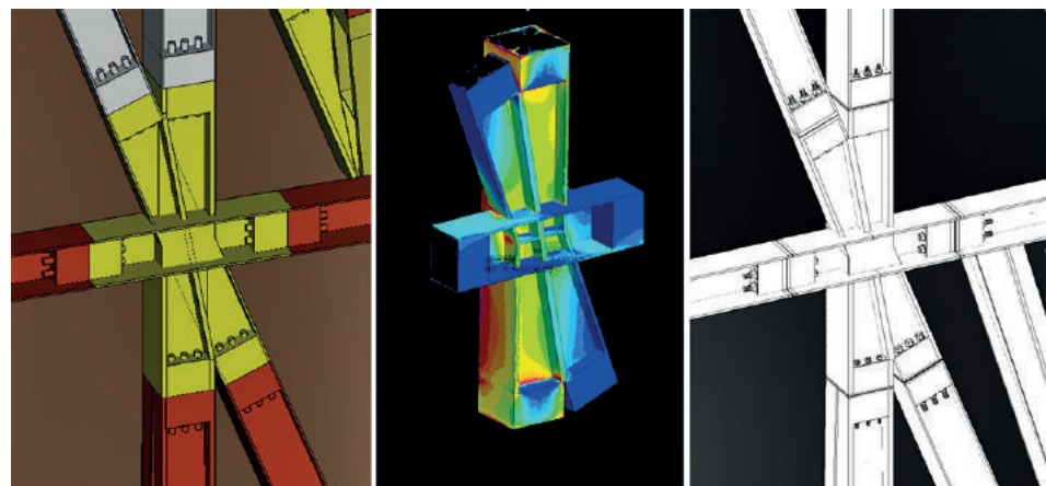
Fig. 13: Early architectural model, FE analysis model and final fabrication model of a flank node 5.
