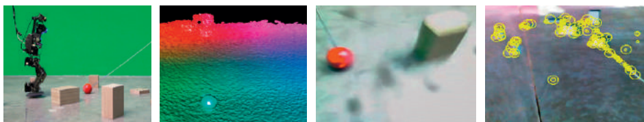
Fig. 4: Our team mounted a 3D scanner above the motion tracking video camera of a Darwin OP bipedal robot. This set-up allowed the machine to make accurate 3D terrain maps of its surroundings while tracking a tagged colour object. Darwin has a 32-bit processor and can be used as a software development platform for designing future navigation controls. Left to right: Robot following a moving ball, 3D mesh, video camera POV, and an edge detection system.
