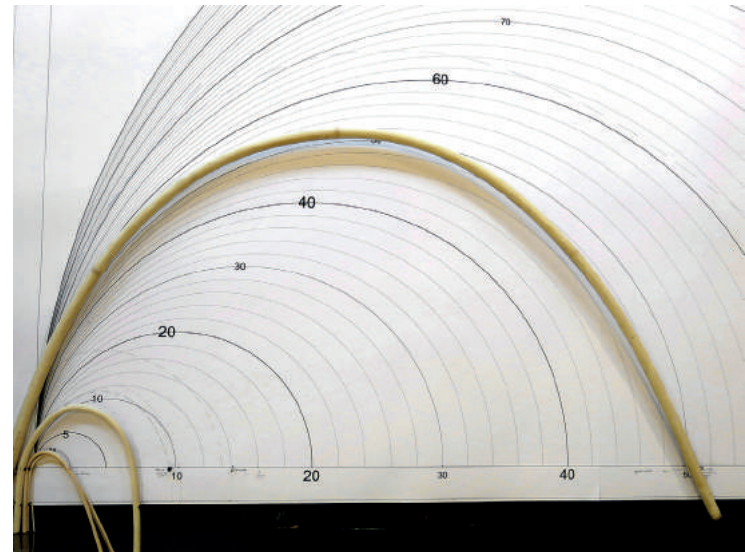
Fig. 8: Identification of minimum bending radius by rattan section.
