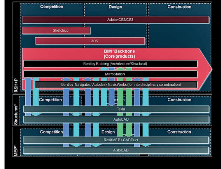
Fig. 10: An accurate map of the software technologies involved and their compatibility helps forecast workflow issues; this map is dynamic and changes throughout the design process.
