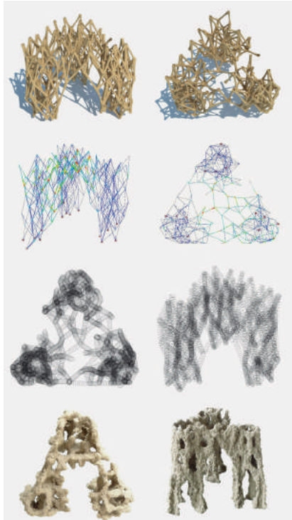
Fig. 5: STONE SPRAY Project, developed by Anna Kulik, Petr Novikov, Inder Parakash Singh. FABbots 3.0. IaaC, 2012. Left: Different phases of simulation culminating in a printed sample. (Photos: Stone Spray team.) Right: Small-scale material prototype of solidified sand and binder, which explores plausible structural topologies that can be achieved by a multidirectional deposition technique.
