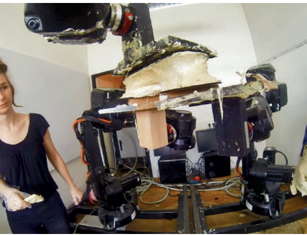
Fig. 8: The process of stretching the material mixture into a self-supporting filamentous foam structure completed with multi-directional manipulation. Event: Robotic Infiltrations, Architecture Challenge 2013. (Photos: REX|LAB.)
