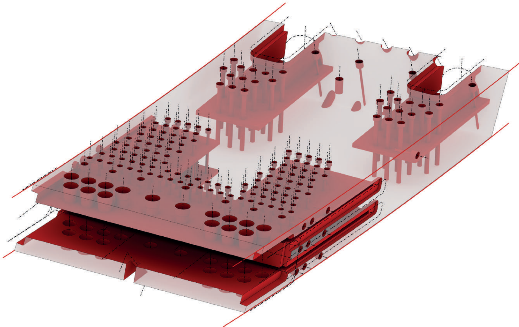
Fig. 1: A single, intricately detailed timber segment of the D1 canopies (see note 8 and fig. 11 ). More than 600 individual segments were parametrically modelled in Rhinoceros and brought into Lignocam for fabrication using a predecessor of Woodpecker. (designtoproduction.)
