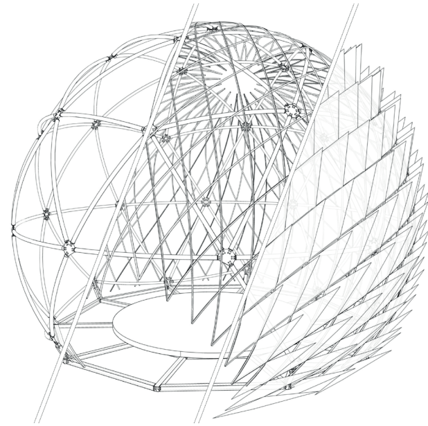
Fig. 2: Main components: 1) Steel geodesic dome, 2) Two kilometres of bent bamboo, 3) 475 stretch fabric flames.
