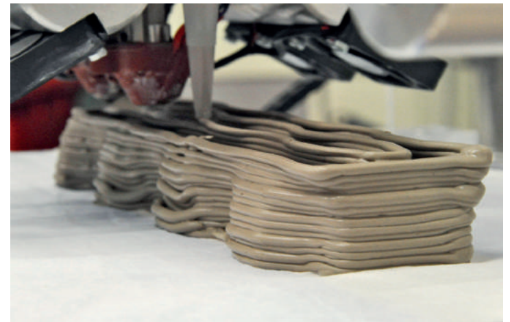
Fig. 7: Printing early honeycomb brick prototype.
