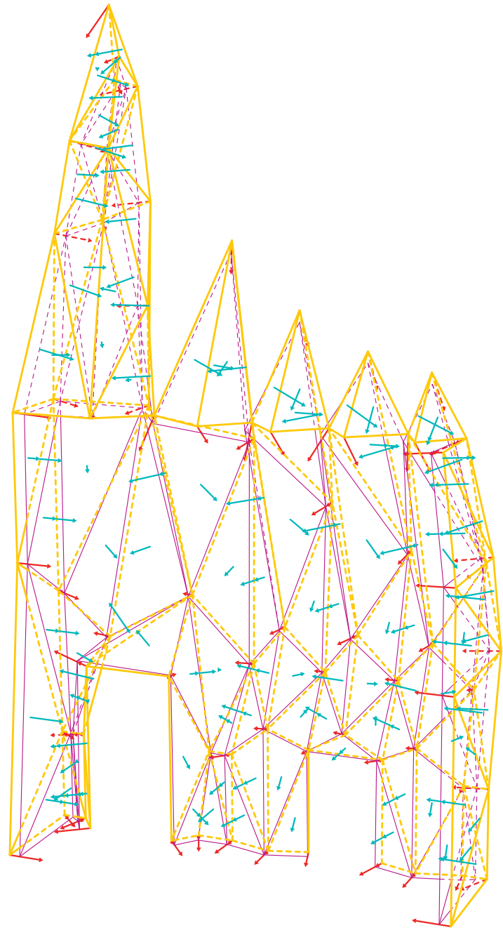
Fig. 5: The mesh topology used to define the façade.
