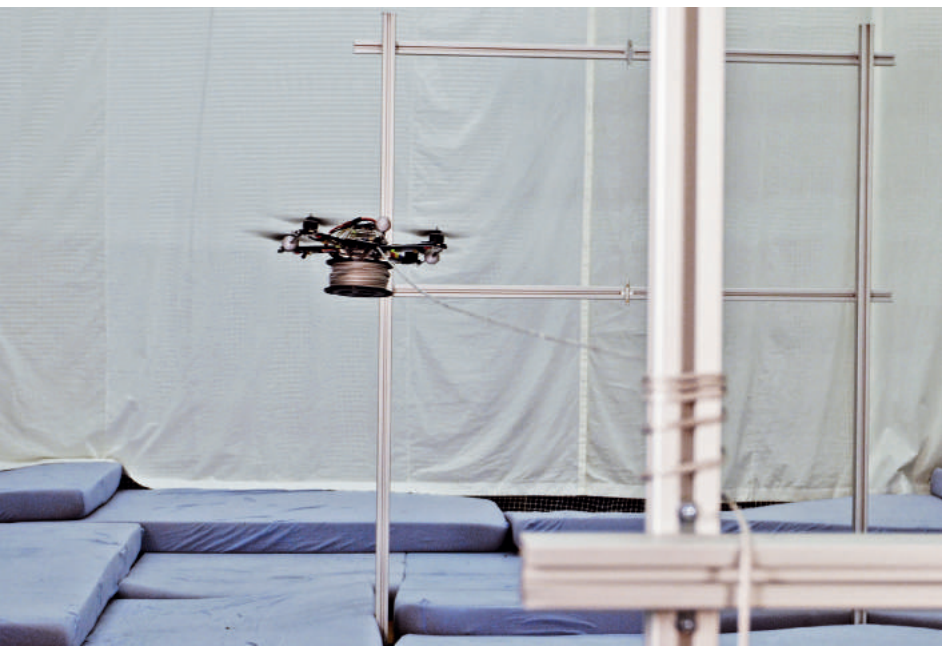
Fig. 4: Autonomous erection of a linear suspension structure.
