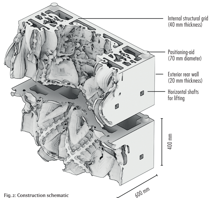
Fig. 2: Construction schematic of two grotto elements.
