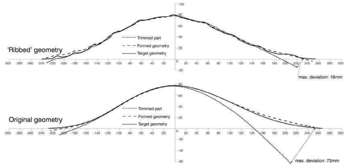
Fig. 6: Evaluation of the geometry before and after trimming.
