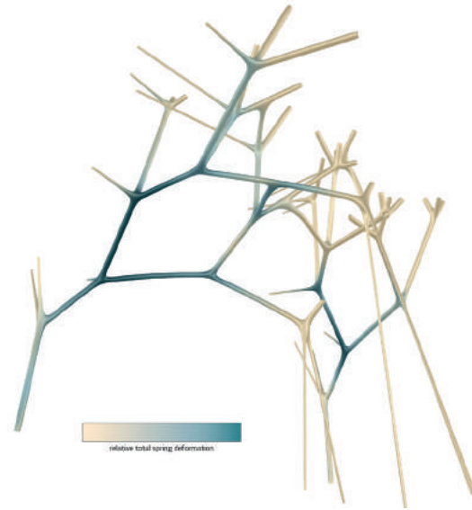
Fig. 10a: Localised spring deformation of morphogenetic model due to bending under self-weight during growth.
