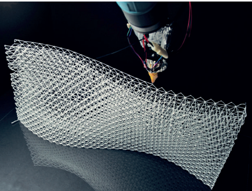
Fig. 4a–b: Robot extruding mesh and first prototype filled with concrete.
