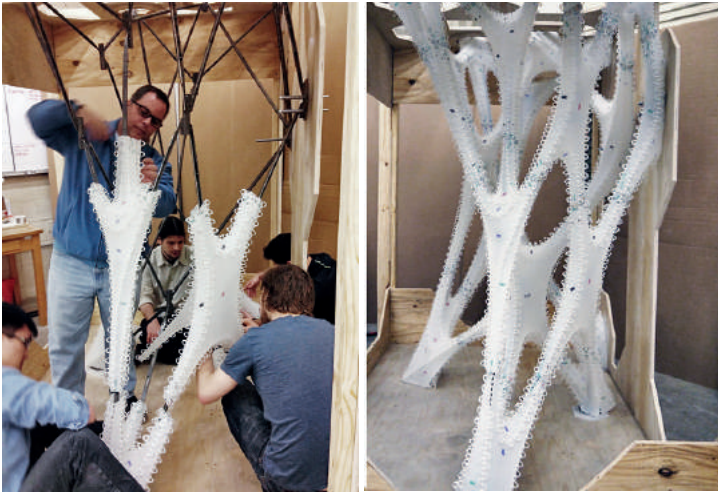
Fig. 10: Plastic formwork assembly process: assembled steel frame, plastic formwork being tied around steel frame, and fully assembled plastic formwork.
