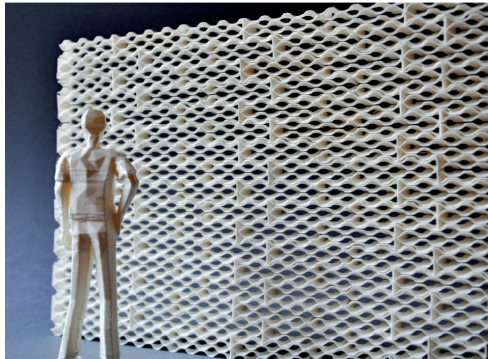
Fig. 10: Honeycomb brick: full-scale wall prototypes.
