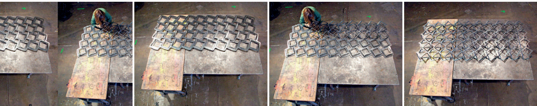
Fig. 7: Process of expanding a steel sheet employing Spin-Valence. (Photo: P.D. Rearick.)
