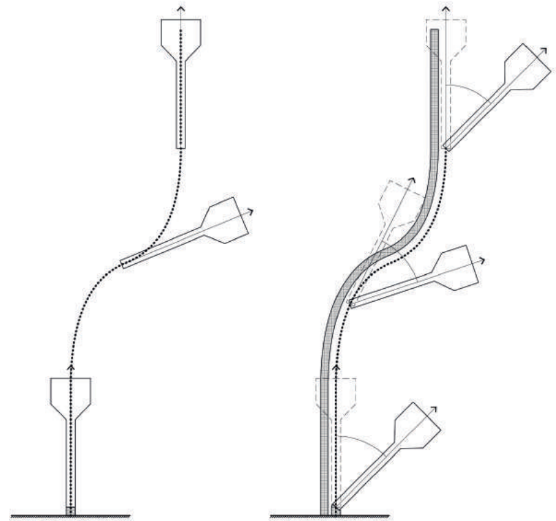
Fig. 5: Side view showing the process of forming a first curve with the orientation of the nozzle. (Image by courtesy of Joris Laarman Lab.)
