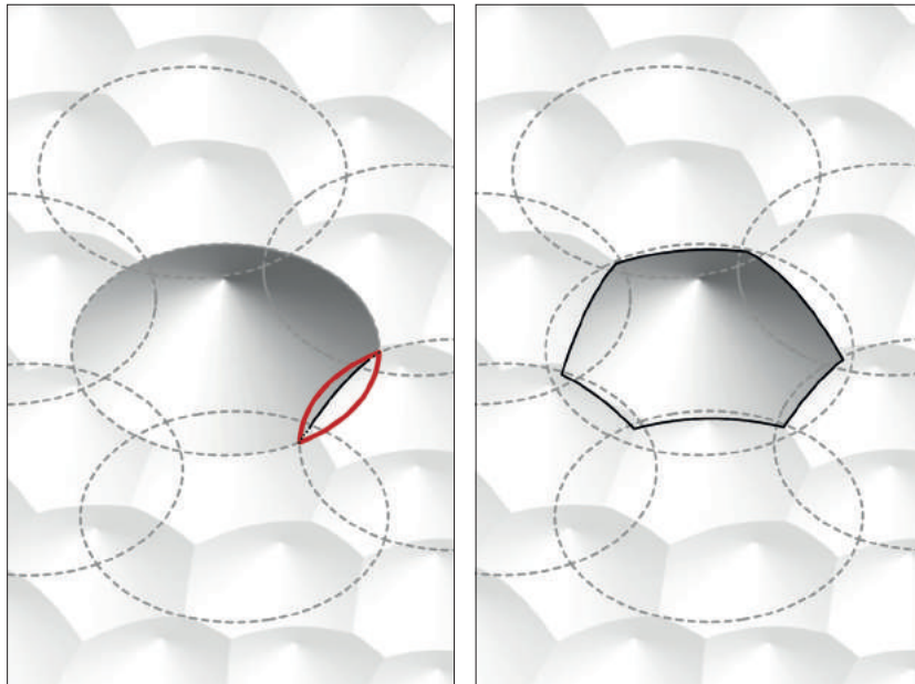
Fig. 4: Intersecting conical geometries. Intersection curves between the units and resulting module geometries after Boolean operations.
