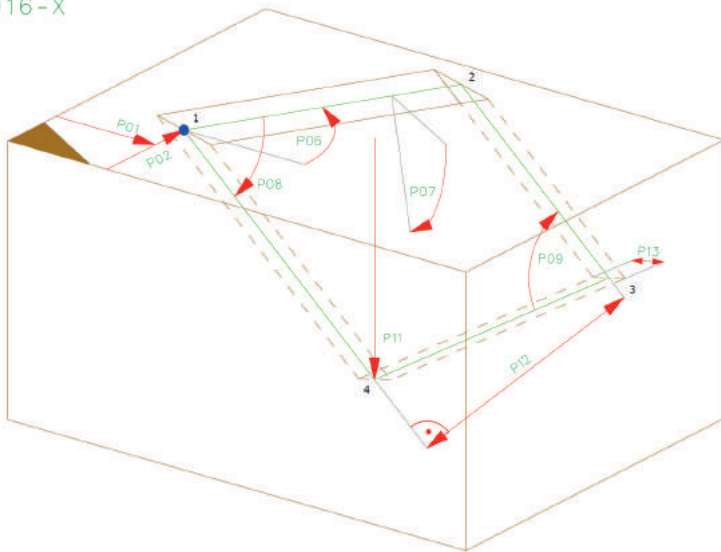
Fig. 7: BTL definition of a slot. While it is complete in terms of geometry, it is not machine-specific and does not contain information about which tool to use. (design2machine.)
