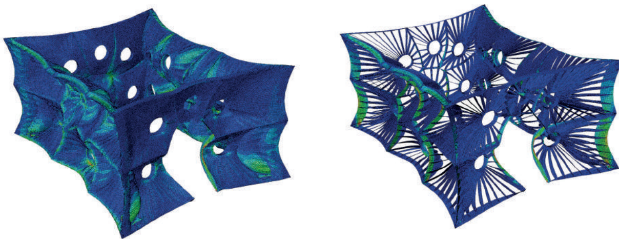
Fig. 11: Finite element analysis of the HygroSkin Pavilion. a) Von Mises stress results of the overall structure. b) Von Mises stress results of the structural frame.
