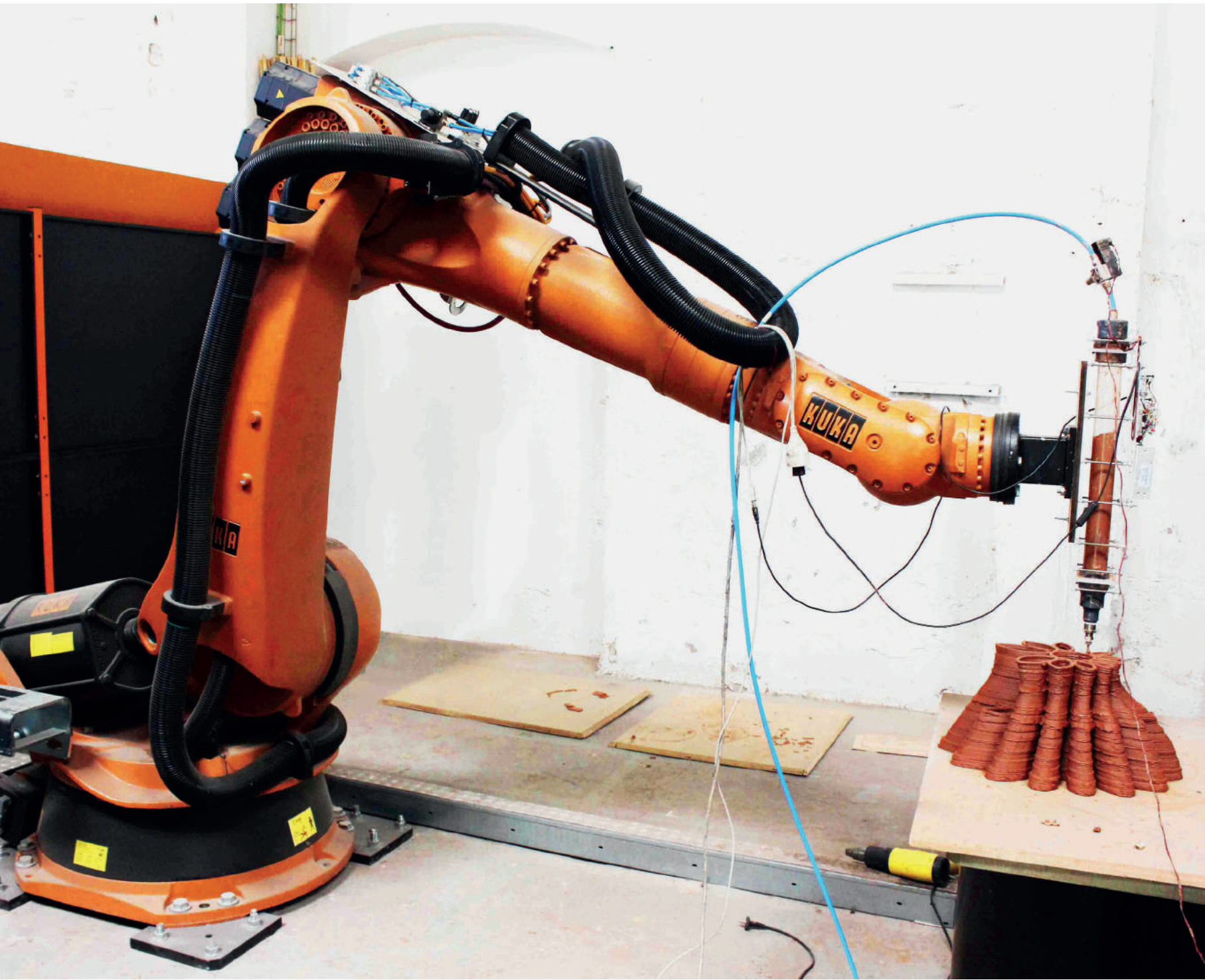
Fig. 1: FABCLAY Project, developed by Nasim Fashami, Saša Jokić, Starski Naya. FABBots 3.0, IaaC, 2012. Machine-material test running on a universal robot depositing clay. (Photo: Saša Jokić.)
