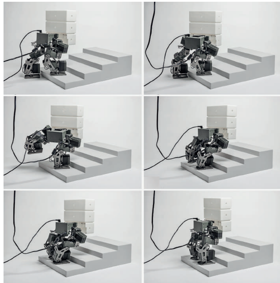
Fig. 3: Payloads ascending a staircase. This working prototype demonstrated the ability of a leg-based robot to carry three stacked components all at once. These horizontal units were conceived at multiple scales as either small building blocks or large modular housing units.
