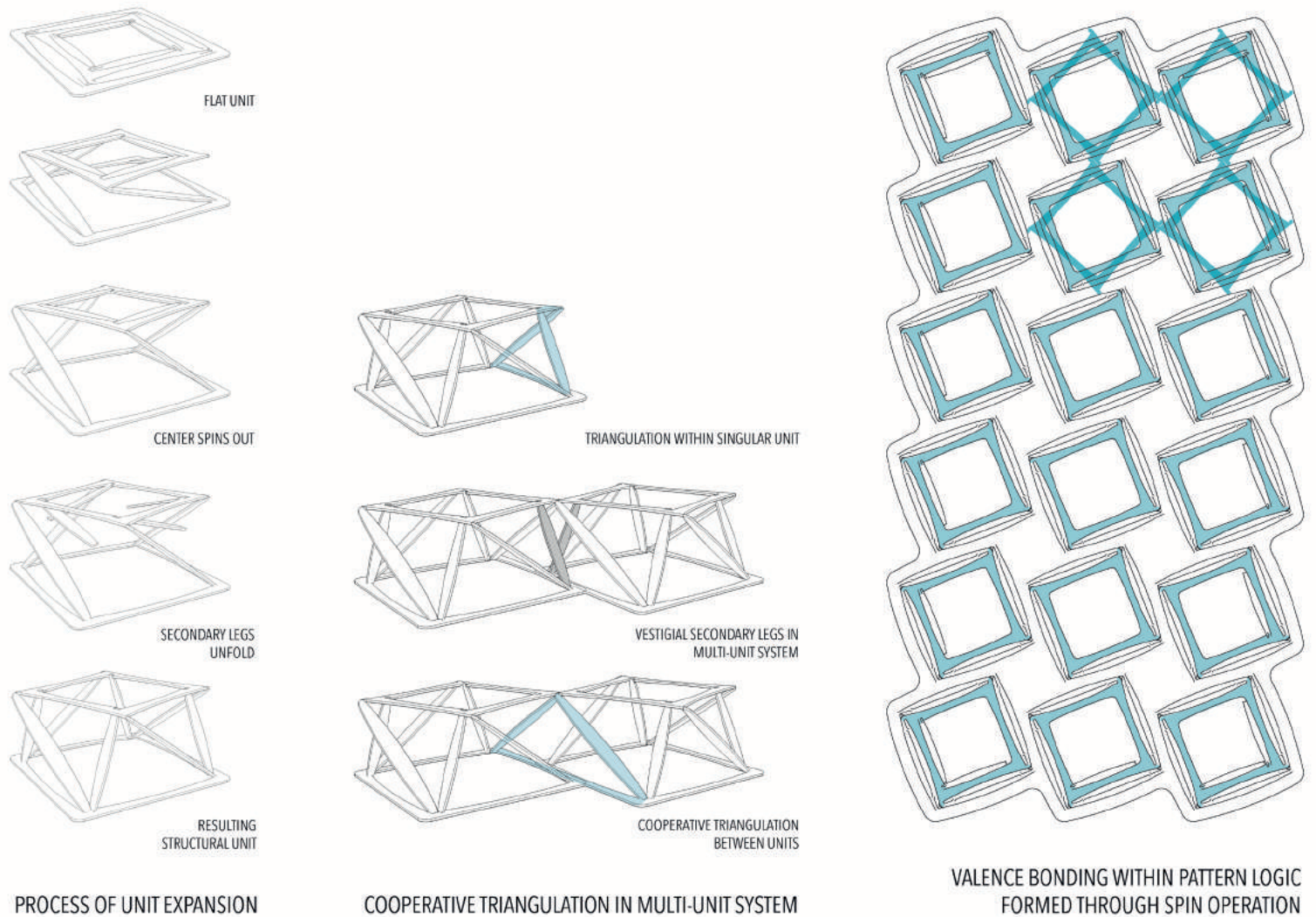
Fig. 8: Left: Process of unit expansion. Center: Triangulation in single unit and multi-unit system. Inner legs become vestigial as units cooperate to create triangulation. Right: Valence bonding formed through spin operation.
