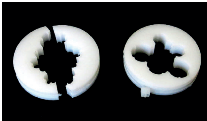
Fig. 13: Packing nodes for organising rattan bundles along structural struts.
