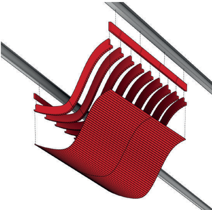
Fig. 5: The timber façade of the Kilden Performing Arts Centre comprises three different kinds of timber components. While feature recognition could be employed for the straight primary beams, the curved and extensively detailed secondary beams were transported as CAD models specifically conditioned for the timber fabricator. For the rather simple, but numerous oak cladding boards, machine code was directly exported from the CAD model, avoiding CAM software altogether. 1 (designtoproduction.)
