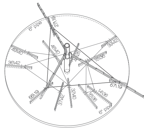
Fig. 6: Steel assembly process: precise horizontal angles registered by angle-finder welding jig. Radially-cut steel pipe, flat-cut steel struts, and plywood angle-finder jig.
