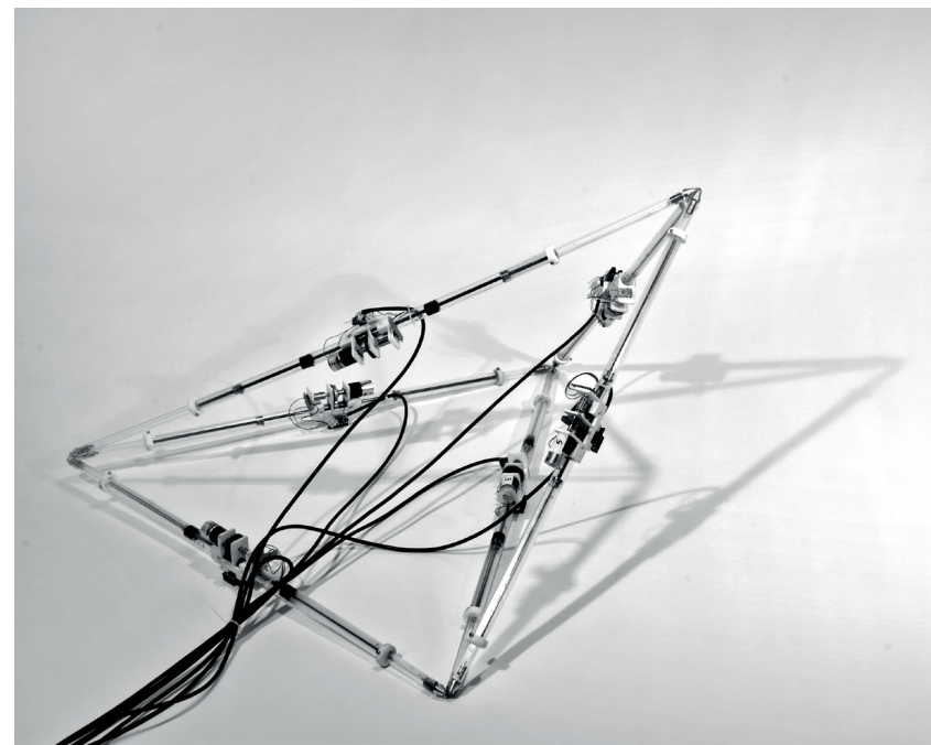
Fig. 6: Prototype for a tetrahedral adaptive truss: partially extended.
