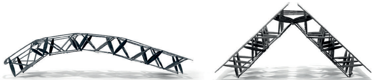
Fig. 9: Side views of curvilinear and angled space frame prototypes in steel. (Photo: P.D. Rearick.)
