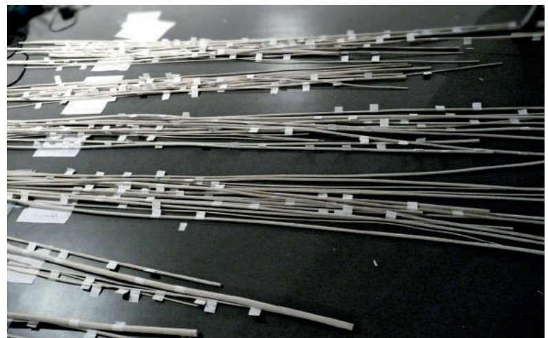
Fig. 20: Rattan elements laid out sequentially, according to installation order, with temporary tags showing locations of associated star nodes and packing nodes along the length of each member.
