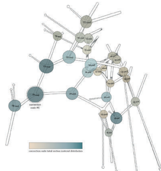
Fig. 10b: Translation of local deformations to assigned material thickness along each connection node.
