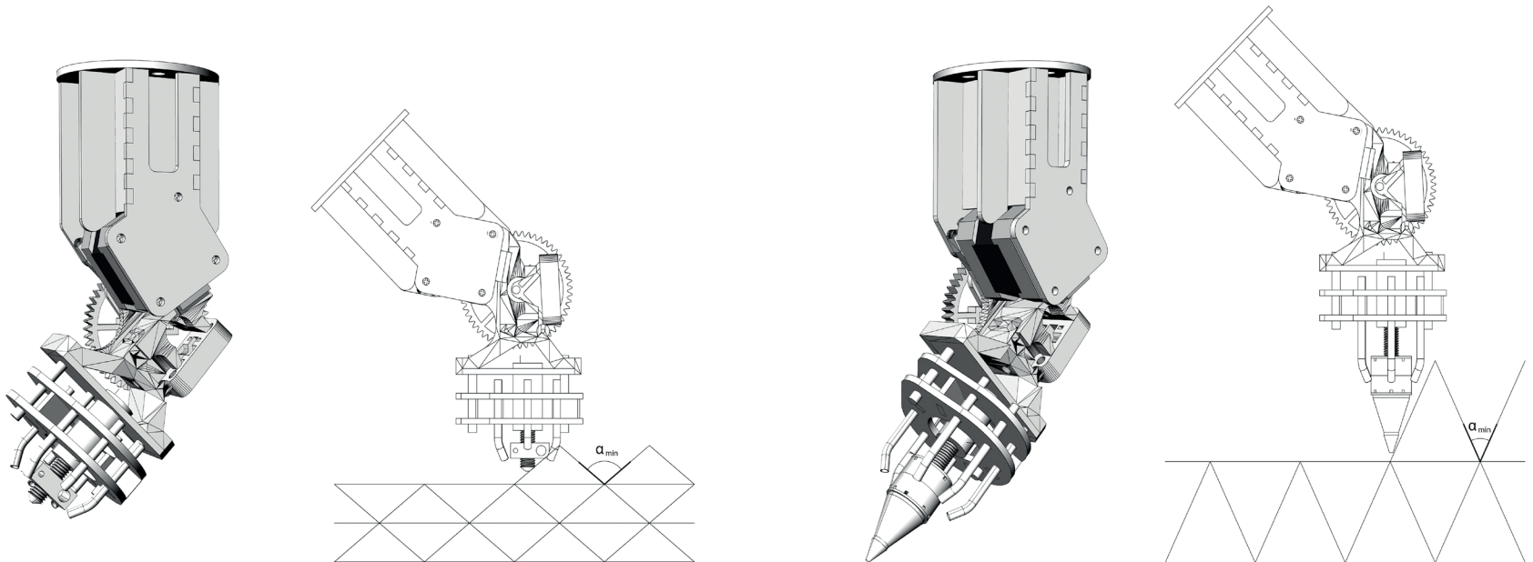
Fig. 5: Extruder head with air-cooling: based on standard components (left) and with custom extruder nozzle.
