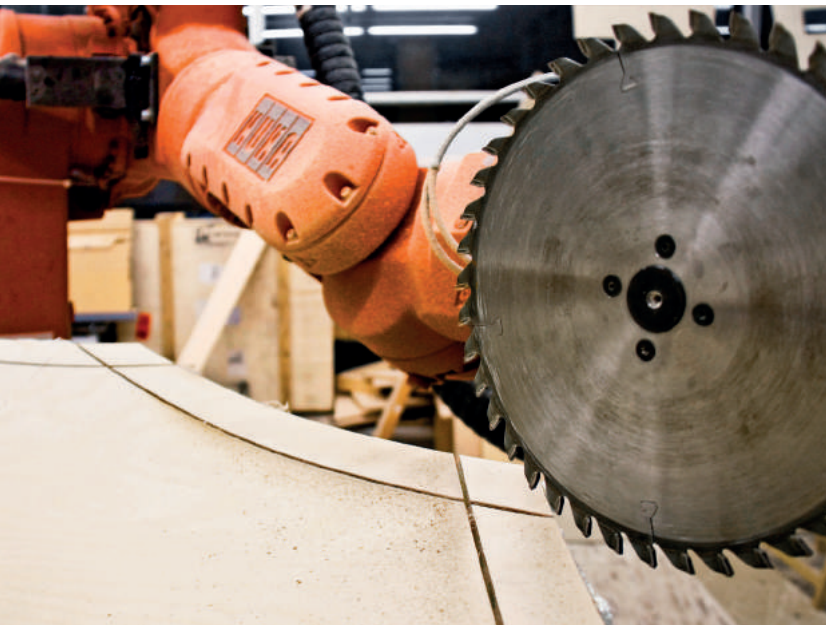
Fig. 8: Trimming the module's edges with a circular saw.
