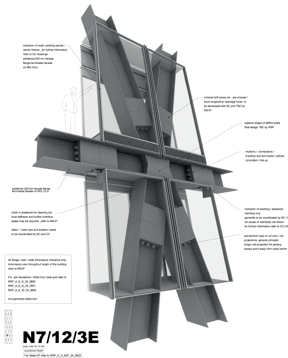
Fig. 4: Node type 7, which occurs on the inclined south façade; the complex façade interface had to be considered part of the architectural requirements.
