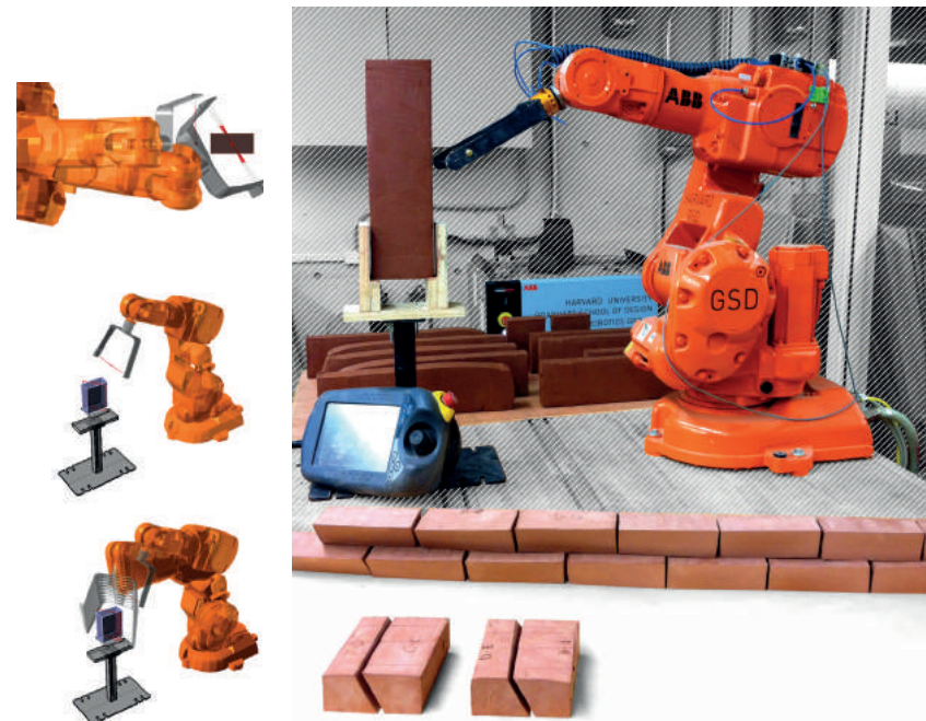
Fig. 11: Robotic wire cutting simulation and prototyping.
