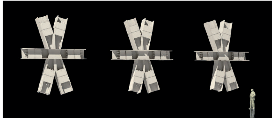
Fig. 5: All node types have sub-variants. The illustration shows the final fabrication models of node 7 types, which all incorporate varying plate thicknesses and bolt layout. Plate thicknesses typically decrease over the height of the building. This approach led to a large number of individually tailored components. The final model was used to automatically generate over 8000 drawings required for fabrication and assembly.
