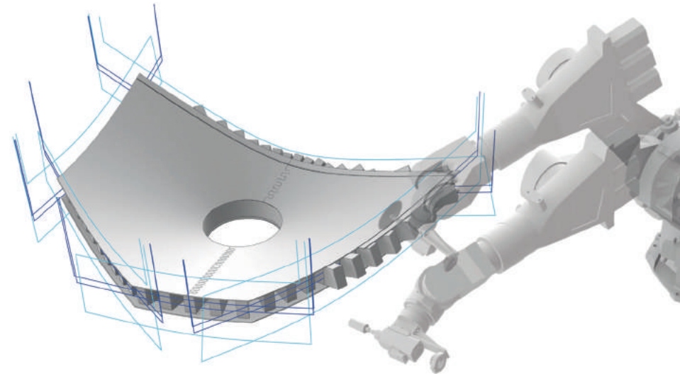
Fig. 9: Automated robot control code generation and simultaneous kinematics simulation.
