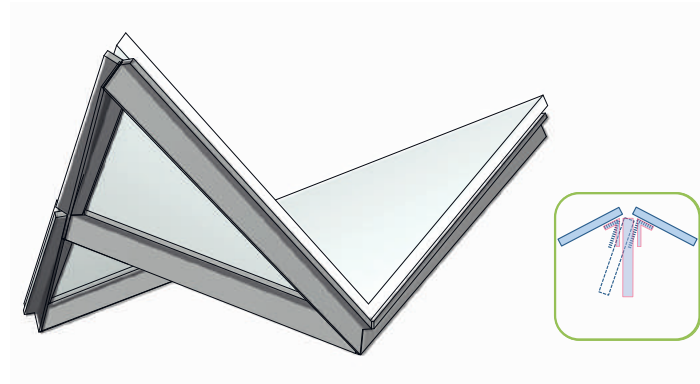
Fig. 7: Structural hypothesis 2 – carrier frame and Plate, with the plate twisted between the end points' non-coplanar vertex normals.
