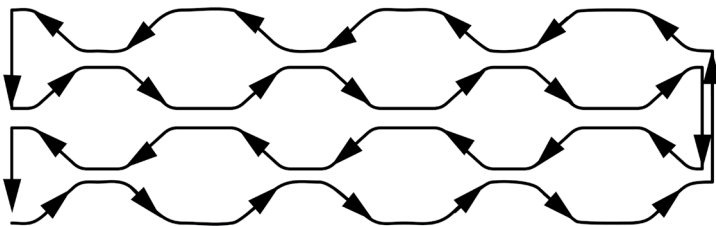
Fig. 4: Diagram of a honeycomb brick printing path.
