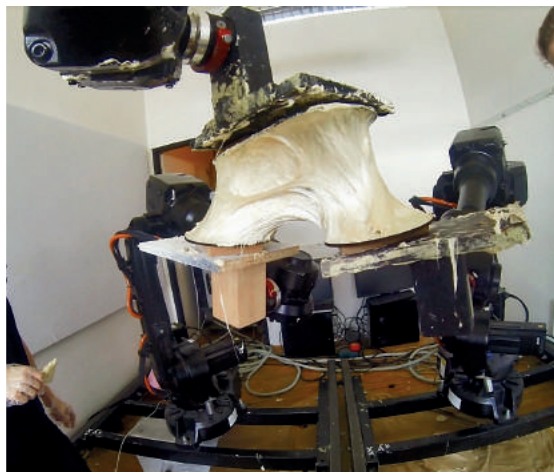
Fig. 8: The process of stretching the material mixture into a self-supporting filamentous foam structure completed with multi-directional manipulation. Event: Robotic Infiltrations, Architecture Challenge 2013. (Photos: REX|LAB.)
