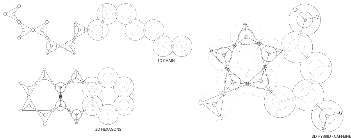
Fig. 3: Intermolecular structures, including 1-dimensional, 2-dimensional and 3-dimensional patterns.
