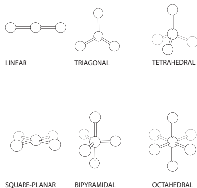
Fig. 2: Intramolecular geometries including: linear, trigonal, tetrahedral, square-planar, bipyramidal and octahedral.
