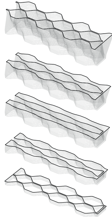
Fig. 5: Diagram of various printing paths that comprise the honeycomb brick.
