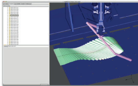
Fig. 13: PyRAPID coding of EPS mould cut with hot wire.
