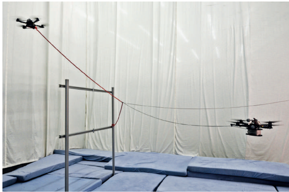
Fig. 5: Multi-vehicle cooperation in freely establishing a knot in space.
