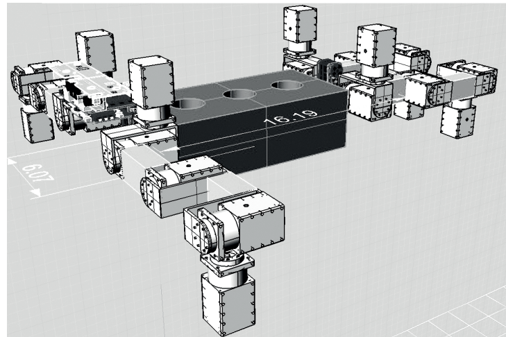
Fig. 8a–c: Sketch model of our proposed full-scale quadruped brick-stacking robot with high-powered servos motors.
