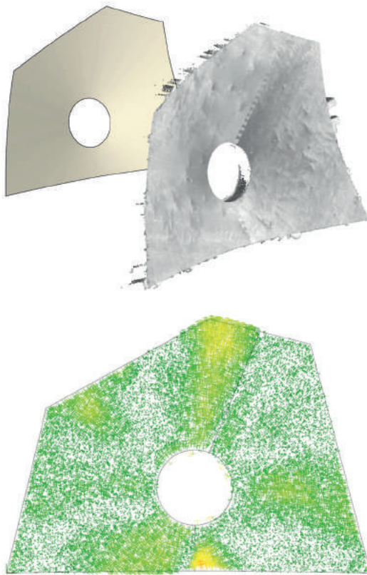
Fig. 10: Precision evaluation through 3D scanning. a) Comparison between the computational target geometry and the elastically self-formed wood panel. b) The evaluation shows a median deviation of less than 0.6 mm (units in mm).
