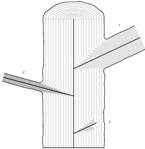
Fig. 3: A simplified section of a branch reveals its complex fibrous structure, which works in compression as well as in tension. (Diagram based on the publications of Dr Alex Shigo). 13
