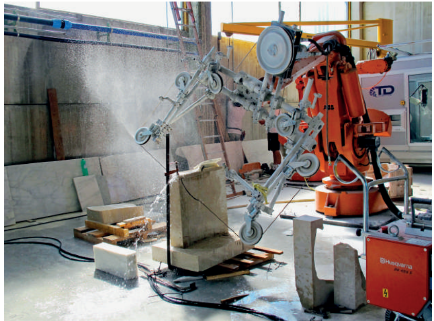
Fig. 4: Experimental diamond wire saw set-up.
