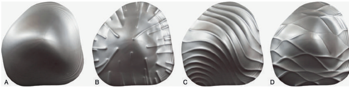
Fig. 5: a) Original geometry. b), c), and d) 'Ribbed' geometry.
