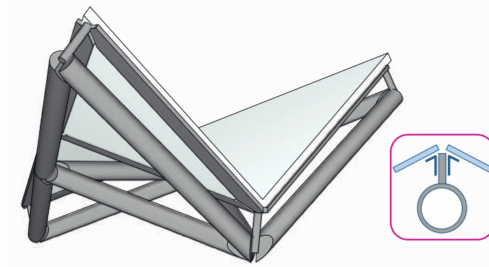
Fig. 9: Structural hypothesis 4 – offset structure and carrier frame, with the offset node connectors based on the average vertex normals.
