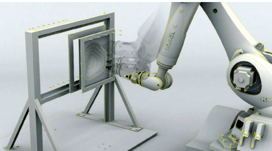
Fig. 2: Single point incremental forming set-up and process.
