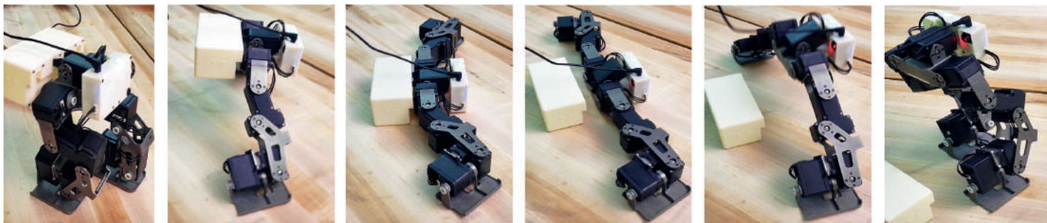
Fig. 6: Bipedal robot deploying an object. This working prototype uses its legs to both grab and transport individual payloads.
