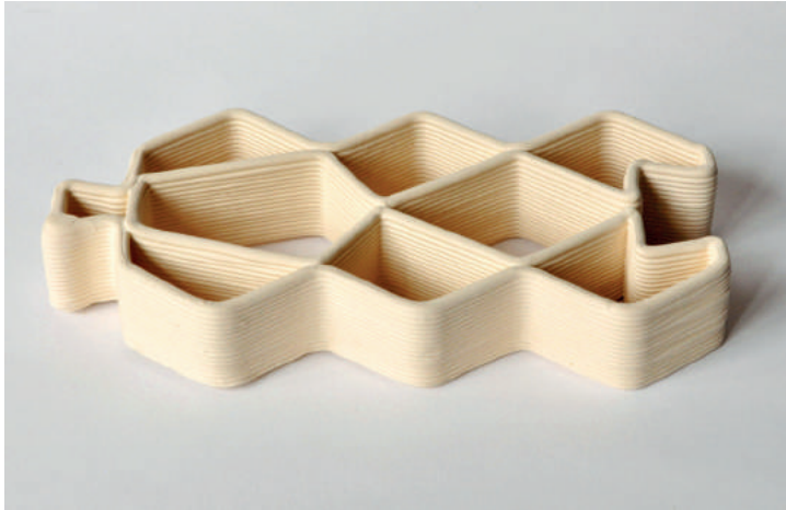
Fig. 11: Interlocking brick: prototype.
