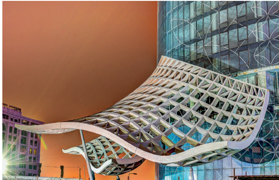
Fig. 11: The four timber canopies surrounding the D1 Tower 8 were modelled in Rhinoceros and brought into Lignocam for fabrication using a predecessor of Woodpecker. (Hess Timber, Rensteph Thompson.)
