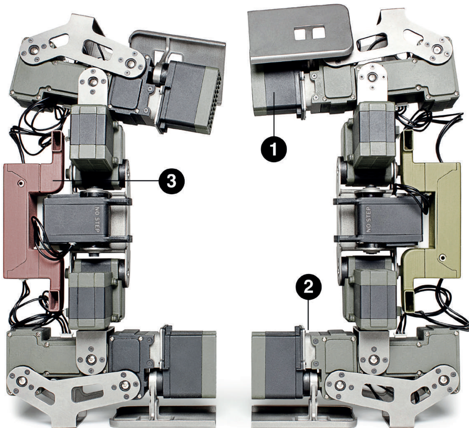
Fig. 1: Two fully functional ABS 3D-printed and titanium-sintered robots shown in the stowed position. Parts: (1) motors, (2) exoskeleton and (3) power plant and sensor package.
