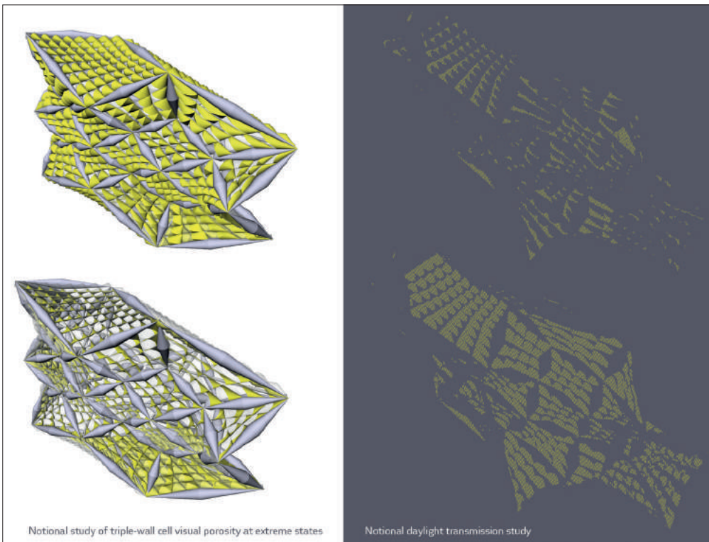
Fig. 13: The computation of material assignment, organisation and fabrication data is performed in relation to orientation and the performance envelope of desired porosity/transmission. A notional study is examined in its two extreme states.
