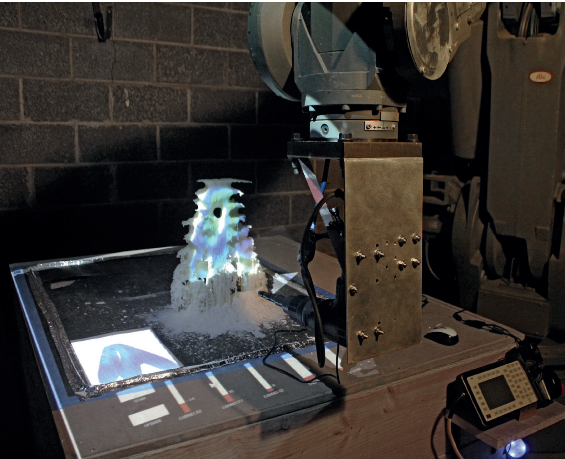
Fig.1: Mixed reality modelling: prototypical set-up for recursive wax forming.
