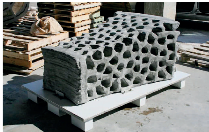
Figs. 10, 11: A large mock-up of the regolith shield was fabricated on the D-shape printer.
