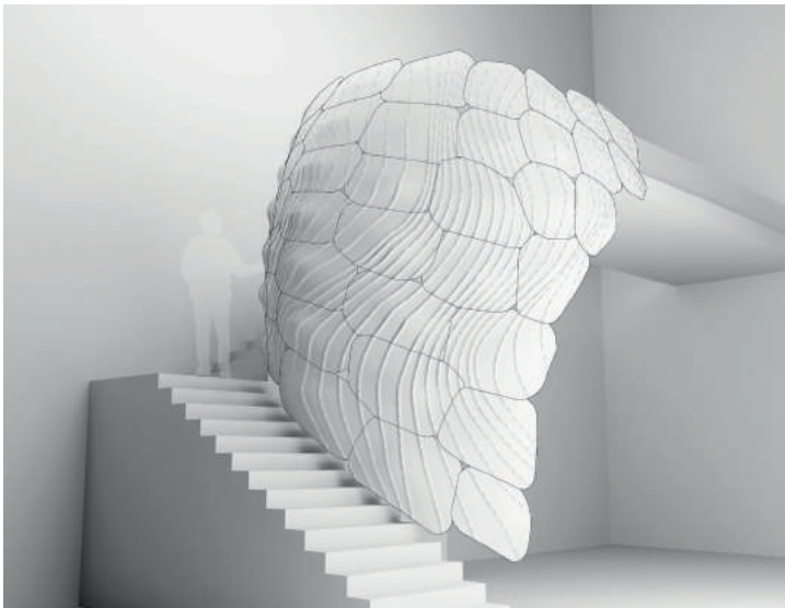
Fig. 10: A proposal for an aggregated interior skin formed with performative ribs.
