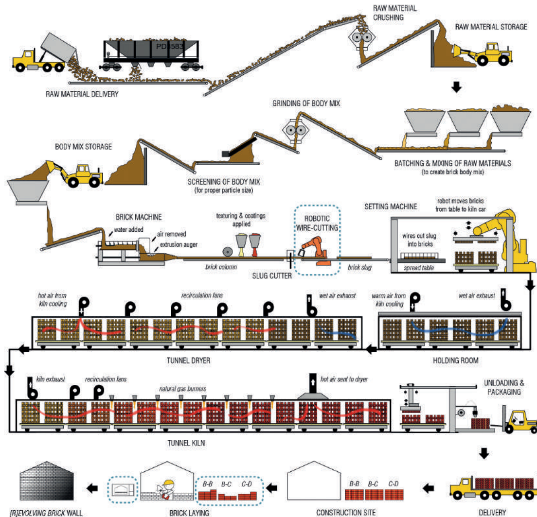
Fig. 4: Envisioned extrusion manufacturing and construction scenario.
