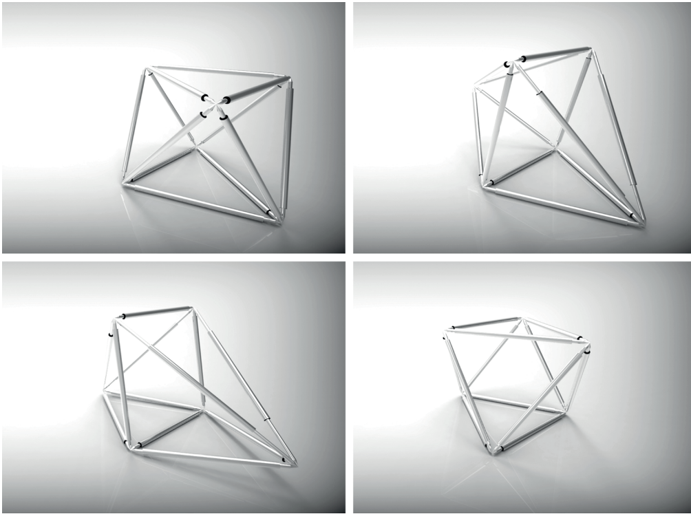
Fig. 11: Simulation for an adaptive octahedral truss.
