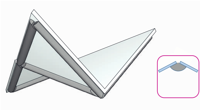
Fig. 8: Structural hypothesis 3 – chamfered tube with chamfer axis using the average vertex normal.
