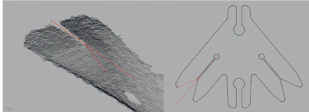
Fig. 8: Data of geometry of deformation through inflation informs the articulation of the receiving node components.
