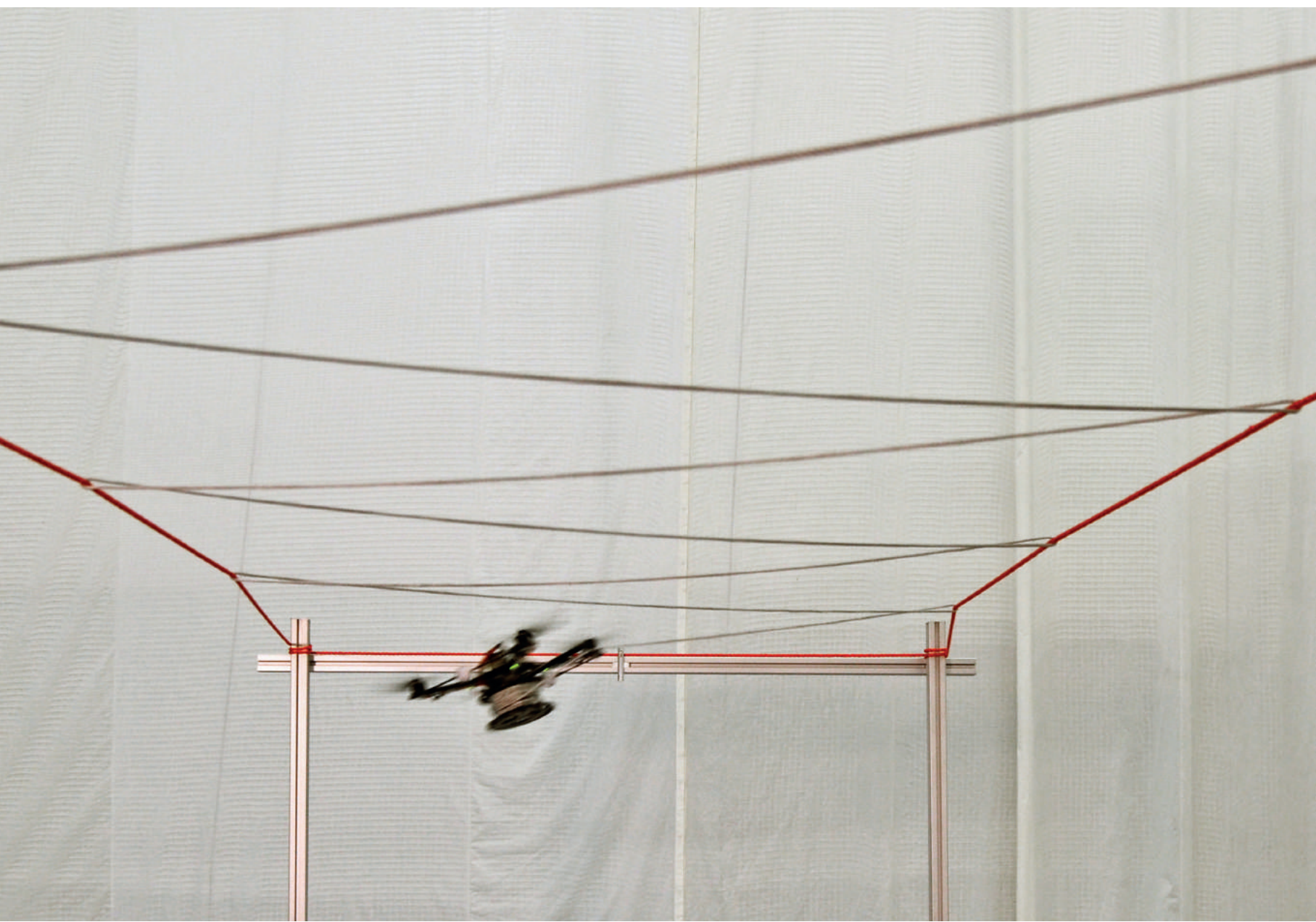
Fig.1: Weaving of a tensile surface structure by flying around already constructed members.
