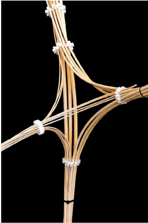
Fig. 9: Physical prototype for testing the digital system and providing materially driven feedback through empirical observation.
