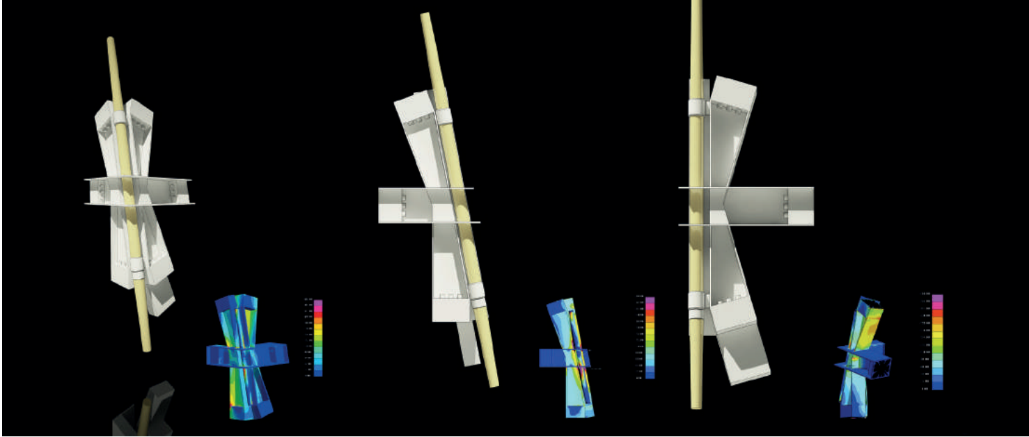
Fig. 8: Architectural model of node 6. The geometry is driven by concurrent analysis. GC was used to capture geometric logic and update the model with plate thicknesses that changed throughout the design process. The analysis, with gradually increasing levels of sophistication, defined the geometry in keeping with an emerged tectonic language.
