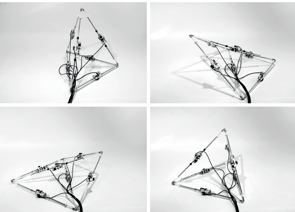
Fig. 5: Step cycle for the adaptive truss.
