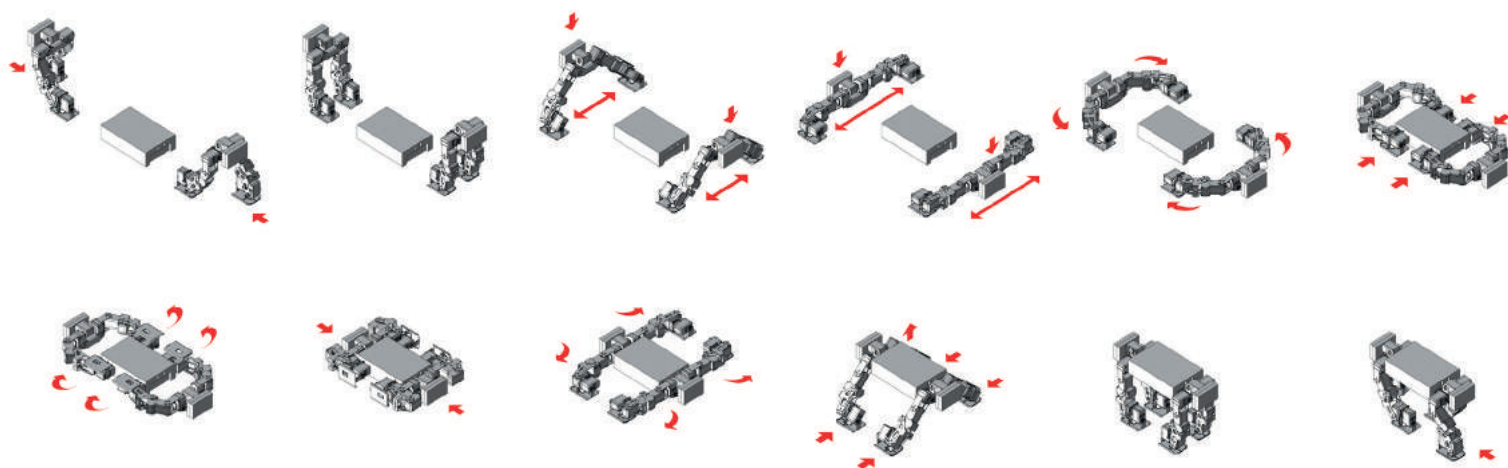
Fig. 5: Two bipeds can combine to form a more stable quadruped that can carry large payloads.
