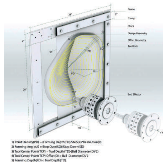
Fig. 3: Basic principles for the parametric toolpath programme.
