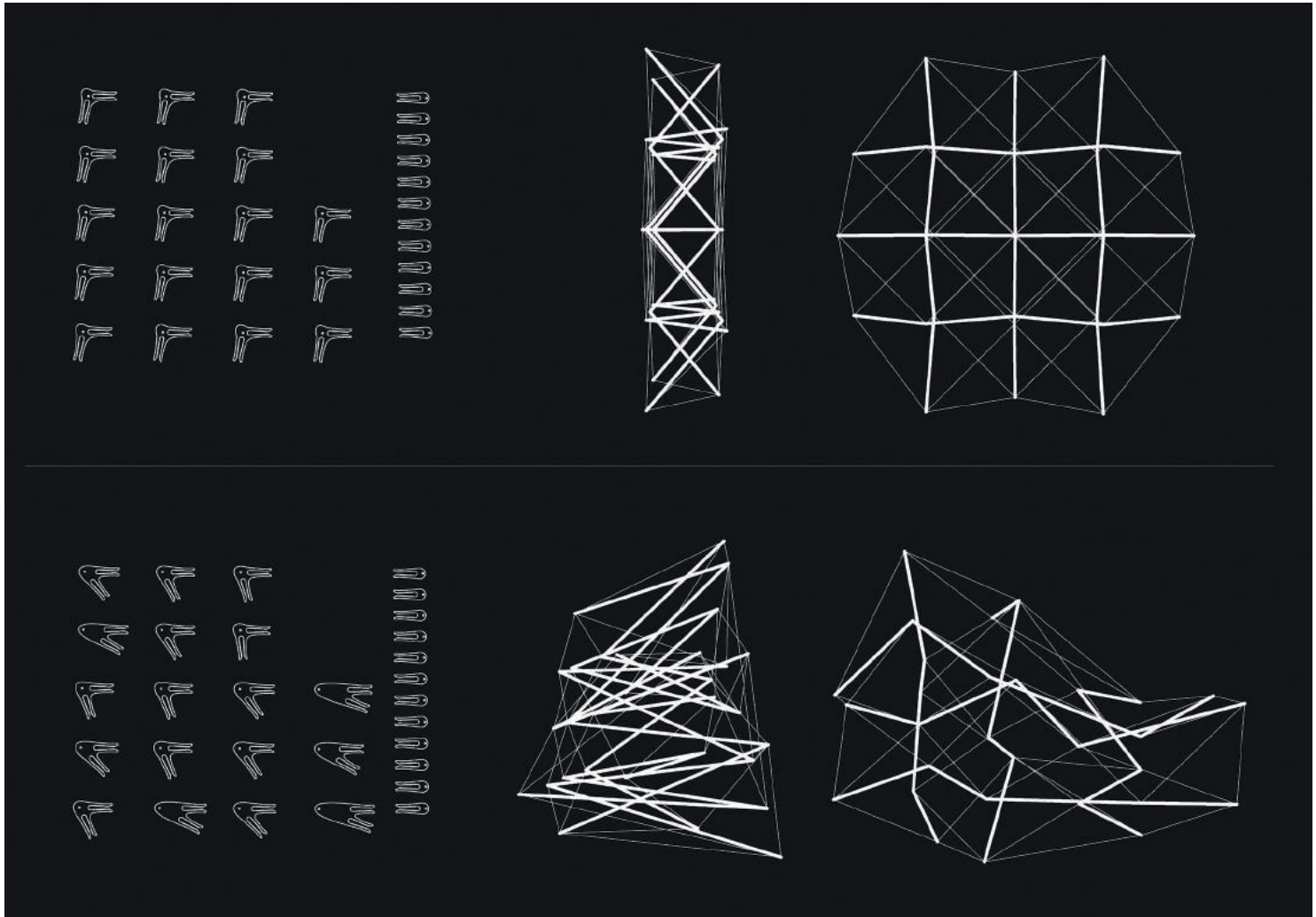
Fig. 4: A double-layer tensegrity topology is encoded in a digital design space permitting the investigation of geometric manipulations and dependencies upon fabrication, in this instance for the production of scale models.
