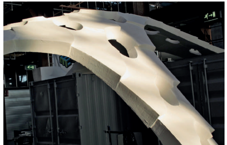
Fig. 2: Discrete components merge into a continuous shell, lacking tectonics.
