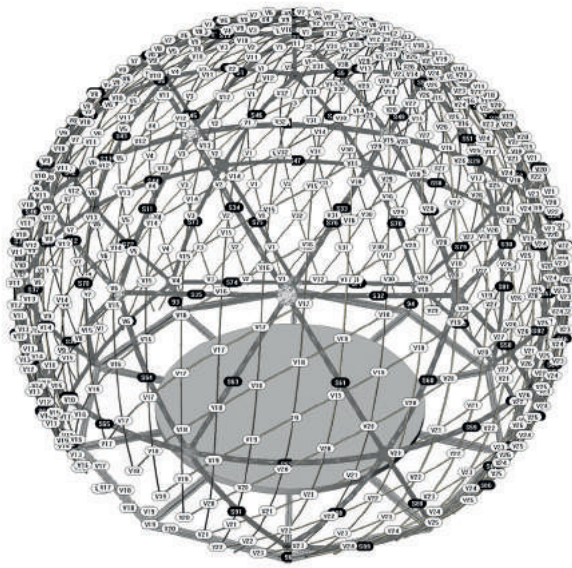
Fig. 4: Intersections between primary and secondary structure.
