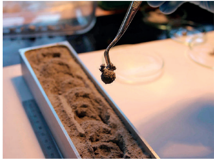
Fig. 13: A small sample was successfully printed in a vacuum by injecting the binder underneath the regolith surface.
