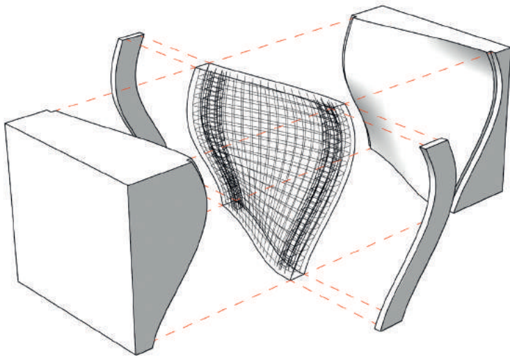
Fig. 3: Conventional formwork and Mesh-Mould.
