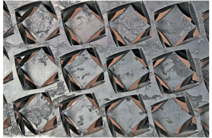
Fig. 6: Prototype in steel.
