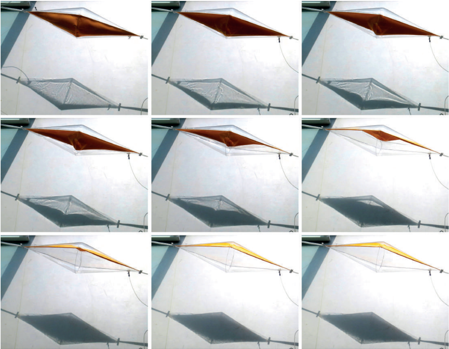
Fig. 11: A preliminary physical test of a triple-wall cushion in which the central wall can be driven by a pressure differential. This generic form of actuation can be tuned to perform a range of environmental mediation tasks – in this case, active shading.
