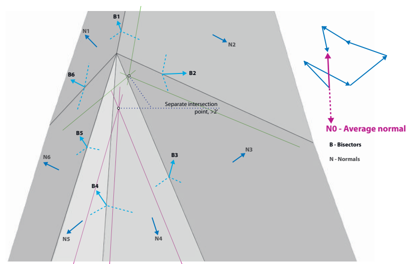
Fig. 3: Characteristics of non-torsion-free geometry, average node vertex normal principle and edge face bisectors.
