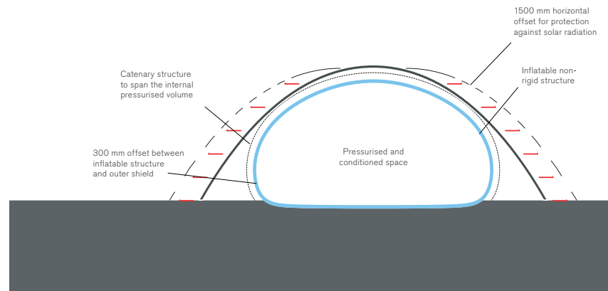
Fig. 7: The lunar outpost is protected from solar radiation by a 1500 mm layer of regolith. 13
