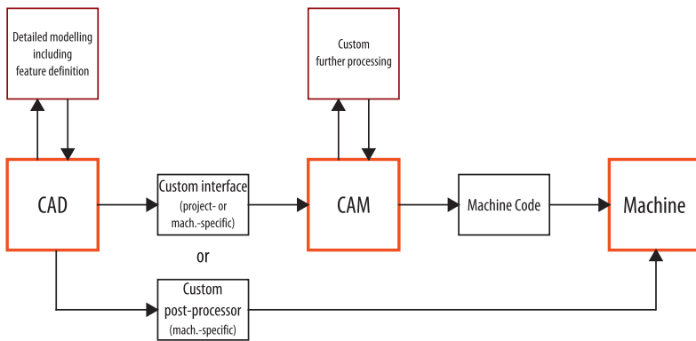
Fig. 4: Digital fabrication workflow using project-specific interfaces or custom post-processors. (Drawing by the authors.)
