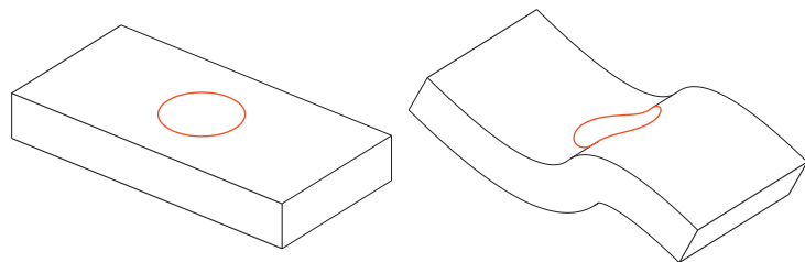
Fig. 3: A hole drilled through a straight beam can be easily recognised from its circular or elliptical edges. On a curved surface, however, the edges are distorted, making automatic recognition of the drilling much harder, not to mention more complex features like five-axis contours or situations with intersecting features. (Drawing by the authors.)
