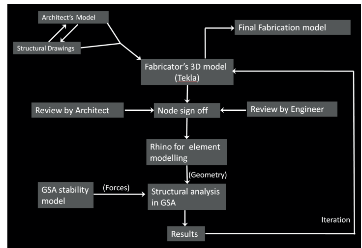
Fig. 11: Diagram of workflow for model sign-off.
