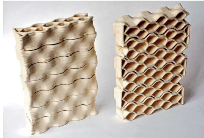
Fig. 9: Honeycomb brick: scale model of screen wall application.
