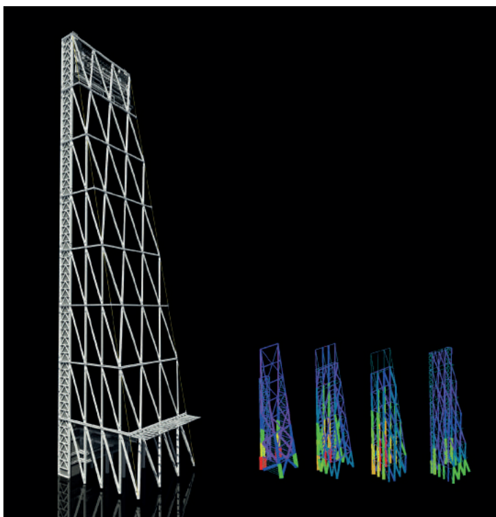
Fig. 3: The base geometry of the Megaframe with analysis diagrams by Arup describing the development of the geometric layout; they illustrate that an introduction of columns to the flank and north elevations of the building reduced the eccentricity effects of the asymmetric geometry significantly, spreading the loads more equally.
