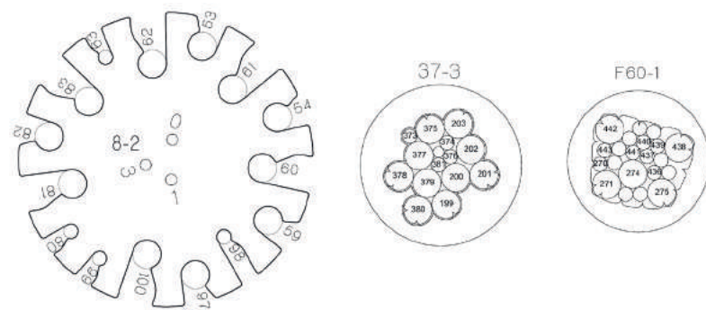
Fig. 17: Sample drawings of various star and packing nodes, from left to right: star node, tight packing node, and loose packing node for the connection of a strut to a flower.
