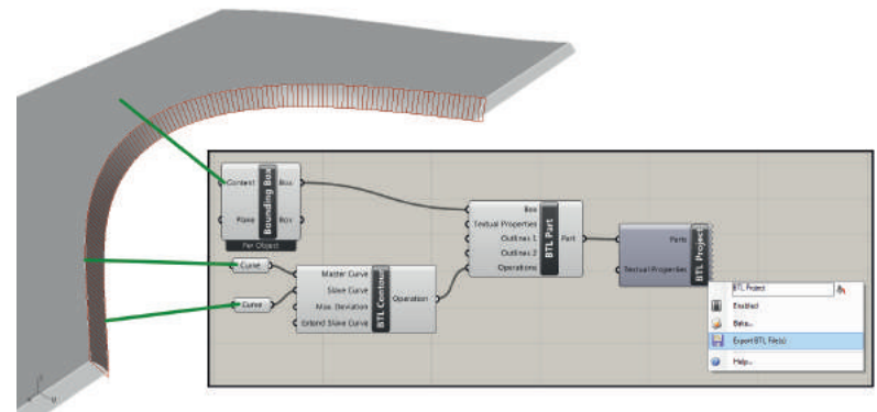
Fig. 10: For the definition of five-axis contours, edges can be taken directly from the final volume. Combined with the raw (bounding box) volume of the piece, a set of information sufficient for digital fabrication is formed. (Screenshot by the authors.)
