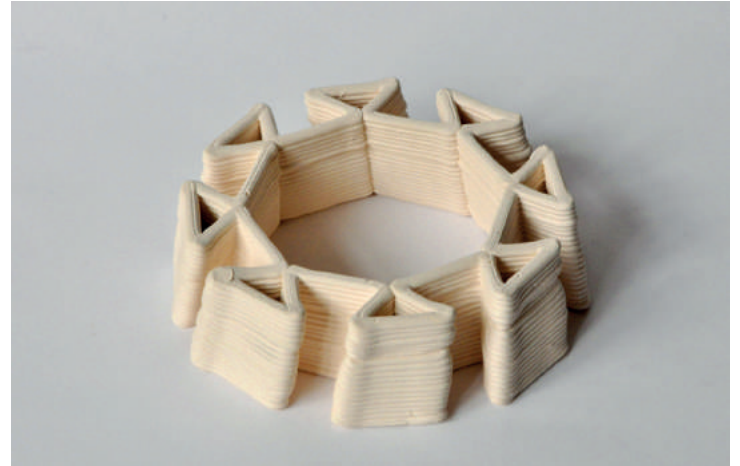
Fig. 12: Ribbed brick: prototype.
