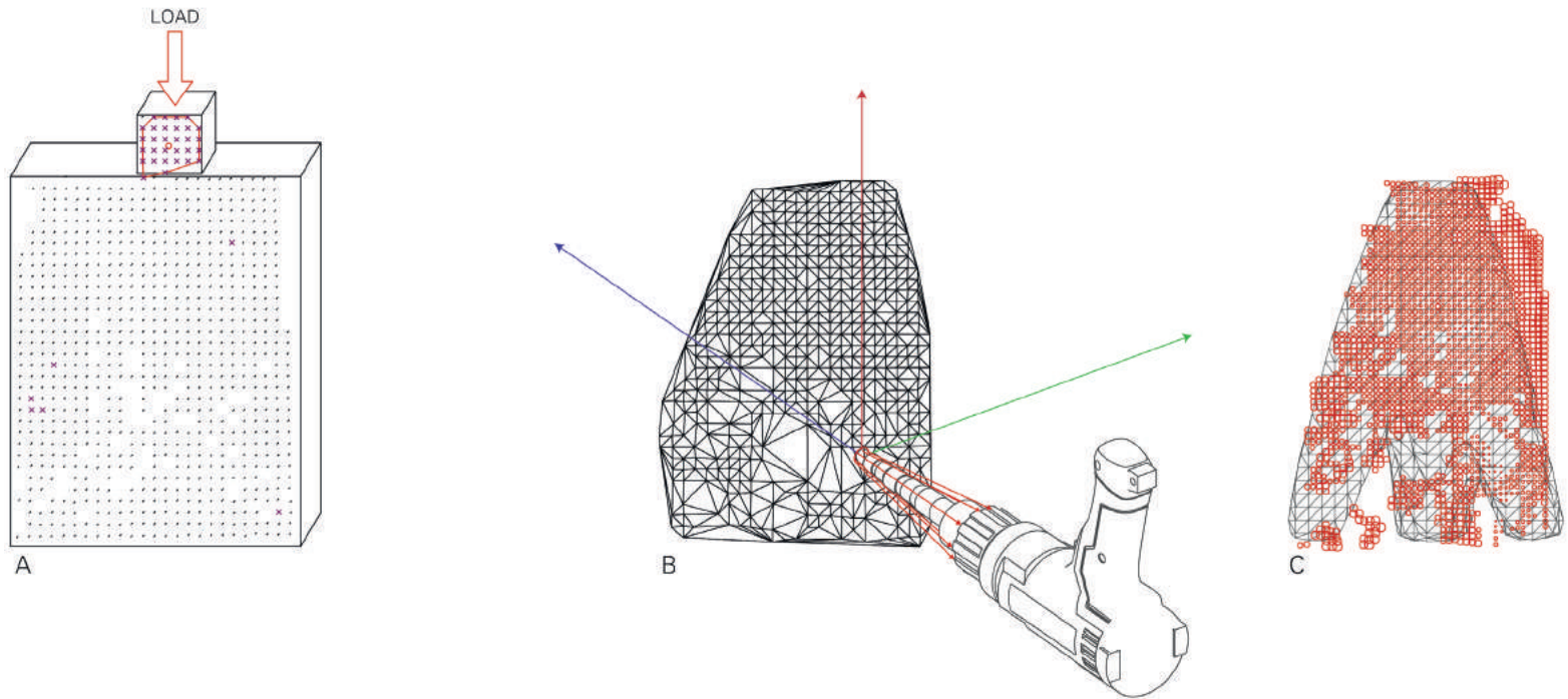
Fig. 5: Select software operations: a) Separate specifically coloured points (purple) and isolate clusters of a given size. Find centroid of convex hull and place virtual load. b) Triangle mesh created from Kinect scan for ray-based collision test. c) Sort scan points by distance to nearest vertex.
