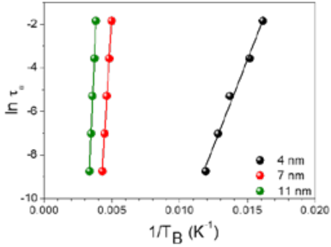
Figure 4.13: \ln \tau_\omega vs. 1/T_{B0} curves for 4, 7 and 11 nm cobalt ferrite nanoparticles. The straight lines represent the best fit to the Arrhenius law (Equation 4.6)
