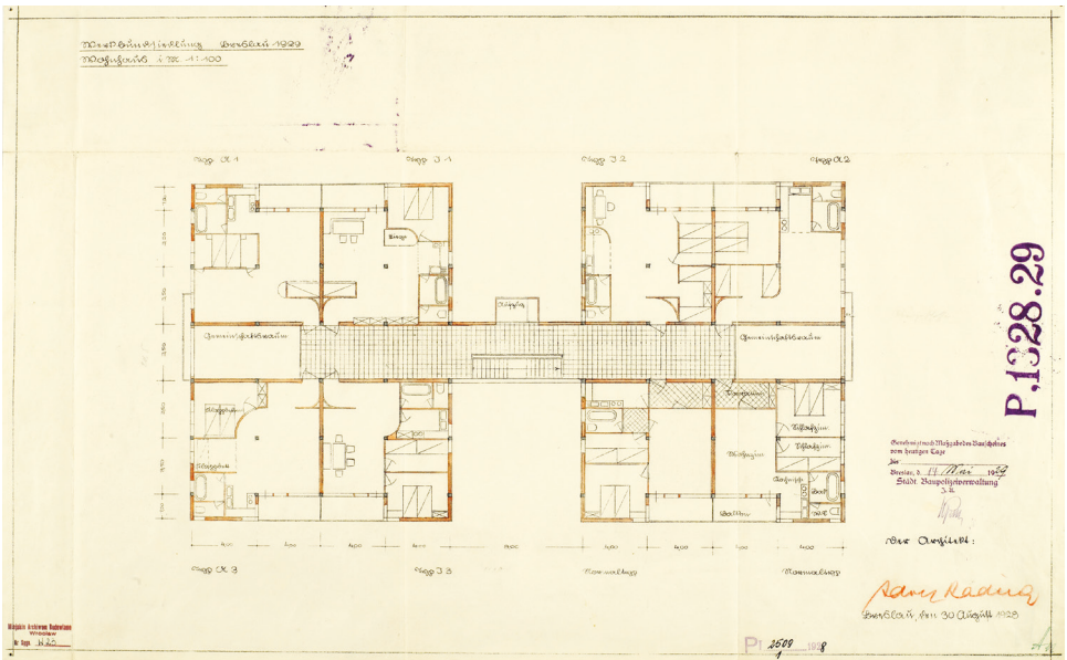
Fig. 25. Rading’s Turmhaus , typical floor plan (Museum of Architecture in Wroclaw).
