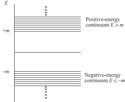
FIGURE 3.1 Energy levels for Dirac particle.
