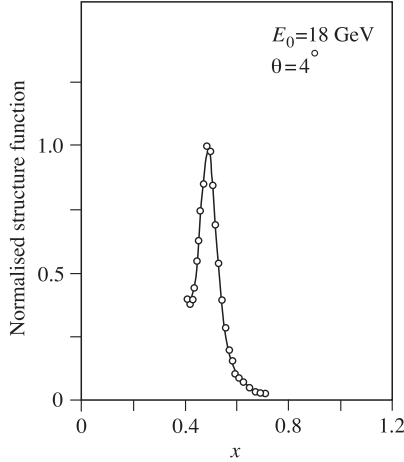
FIGURE 9.5 Structure function for quasi-elastic ed scattering, plotted against x (Attwood 1980, courtesy SLAC).
