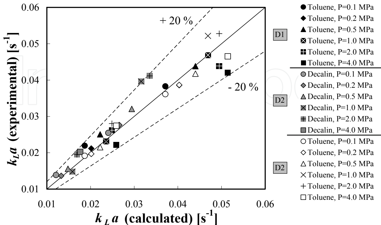
Fig. 10b. Parity plot of k_L a values measured in toluene and decalin at pressures up to 4 MPa (Gas distributors: D1 and D2)
