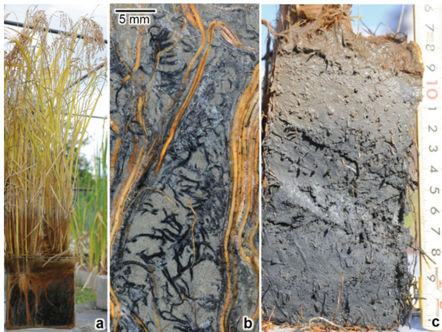
Fig. 5.24 Rice cultivation in a glass container using 1.6 kg soil with N, P, K fertilizers and 8 g \text{CaSO}_4 \cdot 2\text{H}_2\text{O} . (a) soil and rice plants at harvest time, (b) close-up photograph of rice roots darkened by noncrystalline ferrous sulfide, (c) cross-section of soil removed from the glass container
