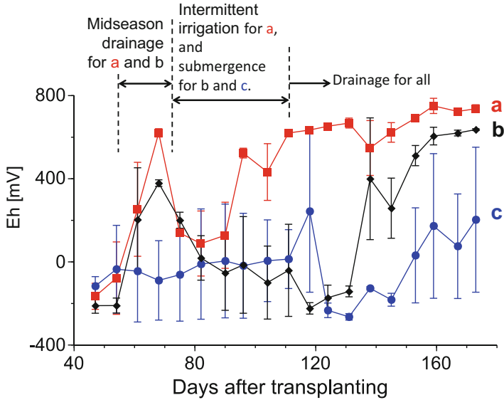
Fig. 5.4 Changes in soil redox potential values (Eh) with different water management schemes. (a) Midseason drainage and intermittent irrigation (MI), (b) midseason drainage and submergence (MS), (c) continuous submergence (CS). The error bars show the absolute deviation from the mean ( n = 2 )
