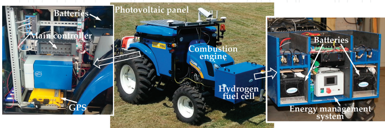
Figure 1. Autonomous robot.
