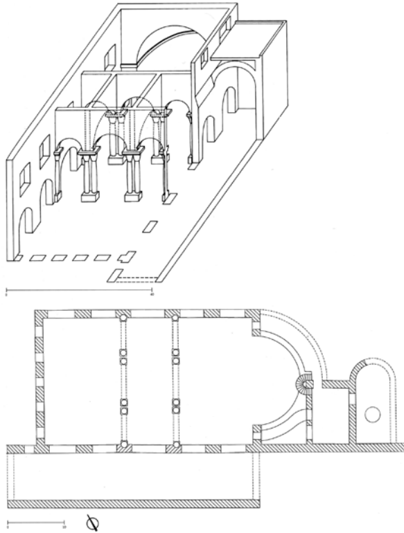
FIGURE 6.1 Rome, S. Croce in Gerusalemme, ca. 320-50, reconstruction of fourth-century plan and elevation (AFTER KRAUTHEIMER AND CECHELLI).
