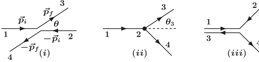
Figure 2.4 Scattering kinematics in (i) the center of mass, (ii) the lab, and (iii) the Breit frames.
