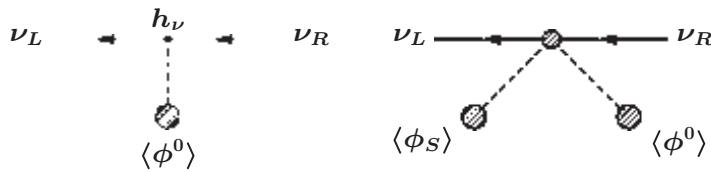
Figure 9.1 Mechanisms for generating a Dirac neutrino mass. Left: an elementary Yukawa coupling to the neutral Higgs doublet field \phi^0 . Right: a higher-dimensional operator leading to a suppressed Yukawa coupling.
