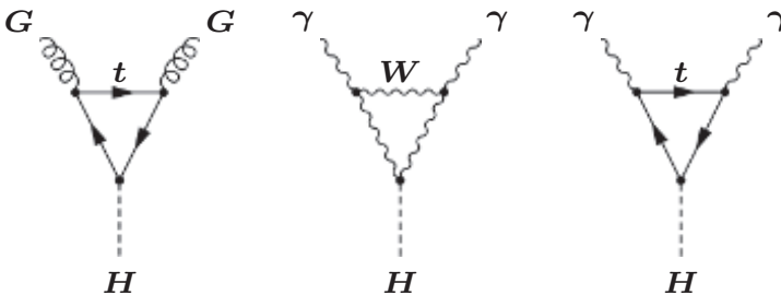
Figure 8.37 Diagrams for the loop-induced decays H \rightarrow GG and H \rightarrow \gamma\gamma .
