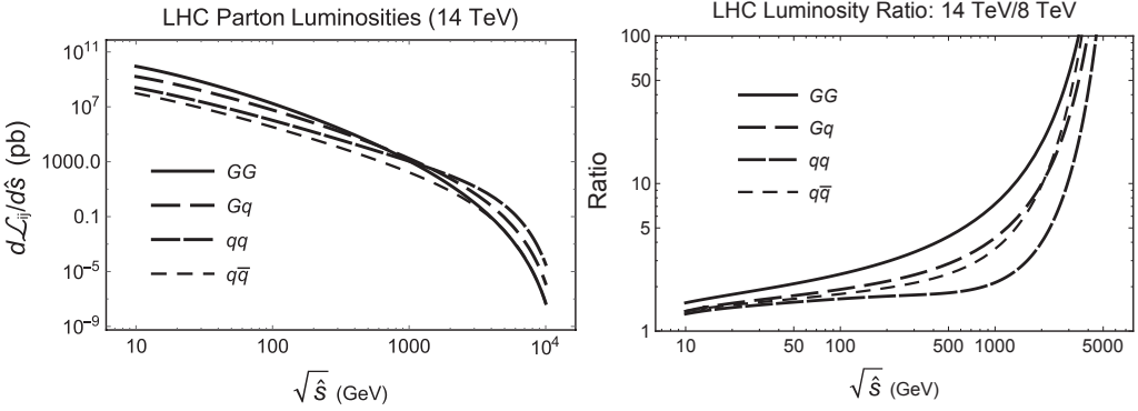
Figure 6.6 Left: LHC parton luminosities at \sqrt{s} = 14 TeV as a function of \sqrt{\hat{s}} , computed using the MMHT2014 NNLO PDFs (Harland-Lang et al., 2015). Gq refers to G_u + G_d , qq to uu + ud + du + dd , and q\bar{q} to u\bar{u} + d\bar{d} . Right: ratios of the parton luminosities at 14 and 8 TeV.
