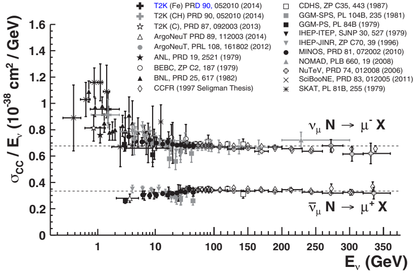
Figure 8.10 Total charged current neutrino cross sections \bar{\sigma}_{cc}^{\nu,\bar{\nu}}/E_\nu vs E_\nu . The simple parton model or QCD predict that these should be \sim constant at high energy. Plot courtesy of the Particle Data Group (Patrignani, 2016).
