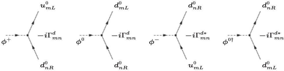
Figure 8.1 Yukawa couplings associated with \Gamma_{mn}^d \bar{q}_{mL}^0 \phi d_{nR}^0 + h.c.
