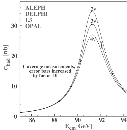
Figure 8.23 Lineshape for Z \rightarrow \text{hadrons} , compared with the expectation for 2, 3, and 4 ordinary neutrinos lighter than \sim M_Z/2 . The asymmetry is due to the explicit factor of s in the numerator of the Breit-Wigner formula (cf. Equation F.7) and to radiative corrections. Reprinted with permission from (Schael et al., 2006a).
