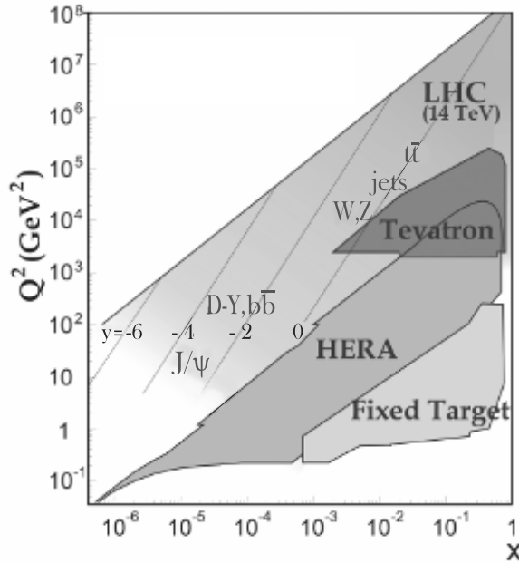
Figure 6.1 Kinematic regions probed by deep-inelastic, pp , and pp\bar{} scattering experiments. Plot courtesy of the Particle Data Group (Patrignani, 2016).
