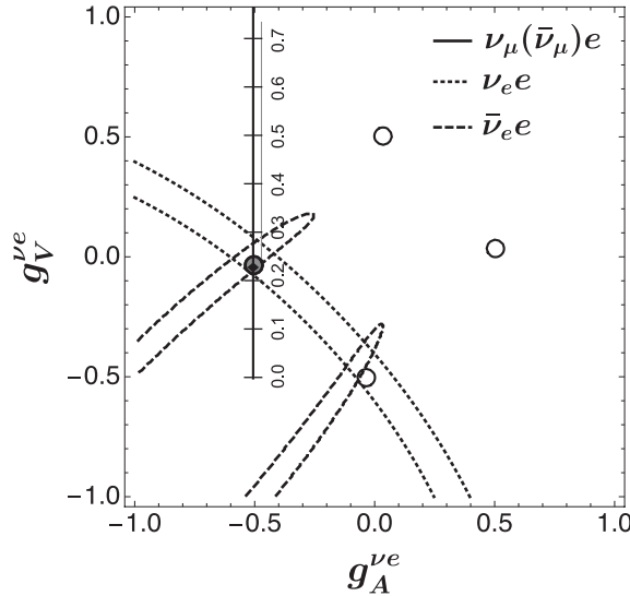
Figure 8.8 Allowed regions in g_V^{\nu e} and g_A^{\nu e} from (\bar{\nu}_\mu)^- e^- , \nu_e e^- , and reactor \bar{\nu}_e e^- elastic scattering, compared to the predictions of the SM as a function of \sin^2 \theta_W in the \overline{MS} scheme. The SM best fit (shaded area) is almost identical to the experimental region. The \nu_\mu e regions are at 90% c.l., and the bands are at 1\sigma . Plot courtesy of the Particle Data Group (Patrignani, 2016).
