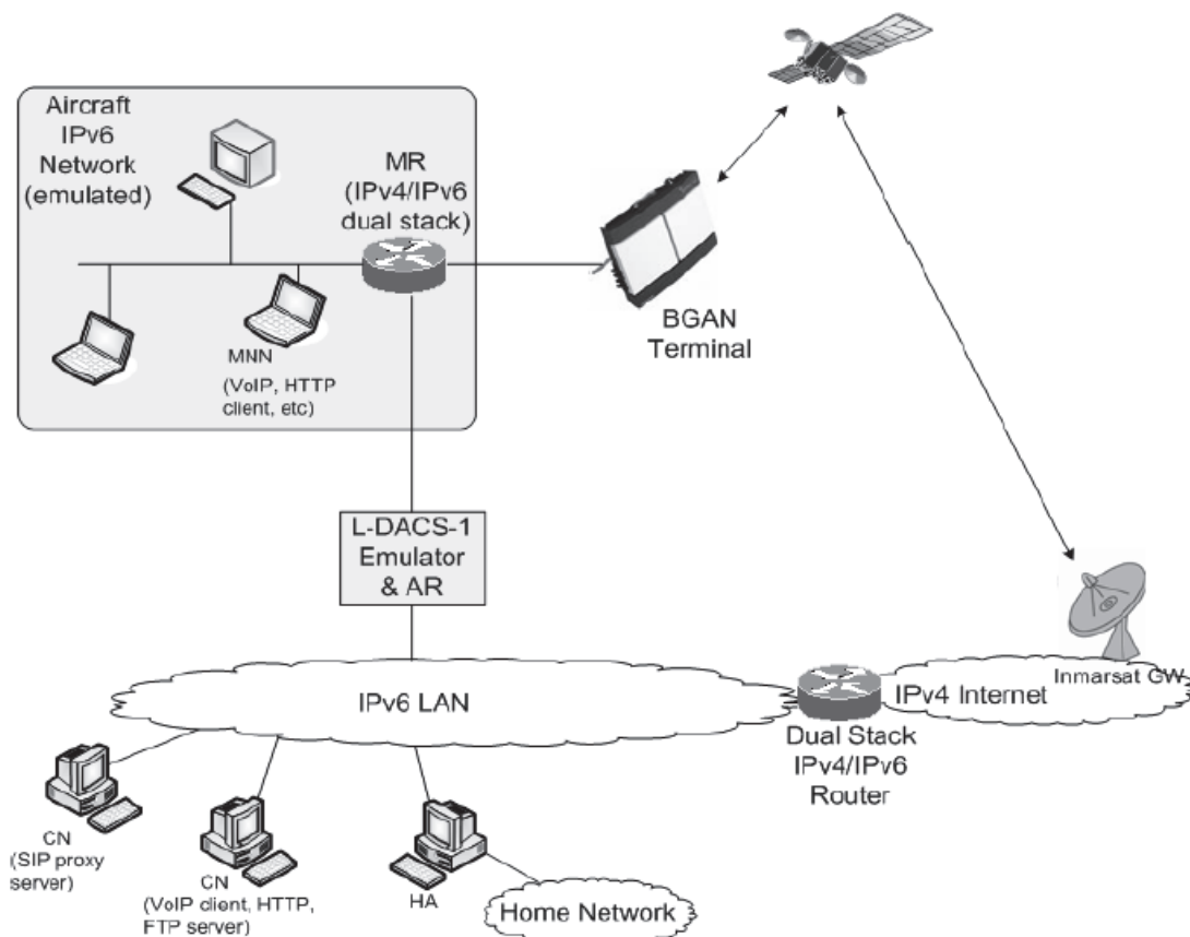
Fig. 1. NEWSKY laboratory testbed network architecture.
