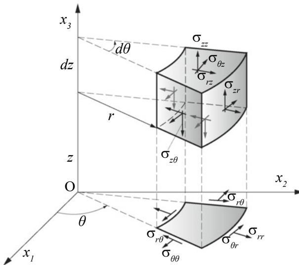
Fig. A.1 Stress tensor components in a cylindrical coordinate system
