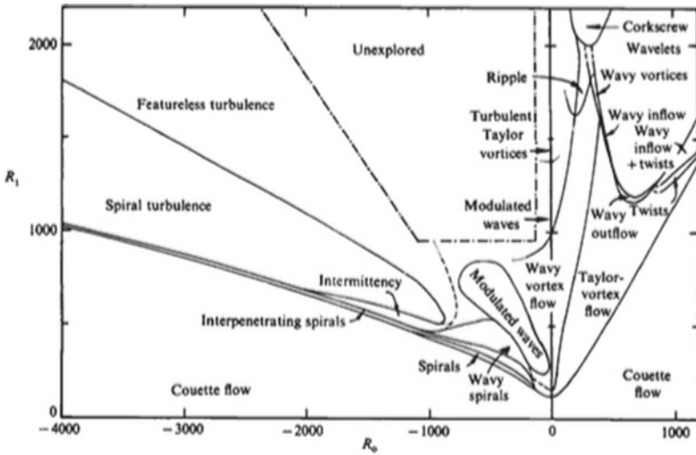
Fig. 8.4 Flow regimes in a Couette apparatus with long co-rotating cylinders. Reproduced from [2]
