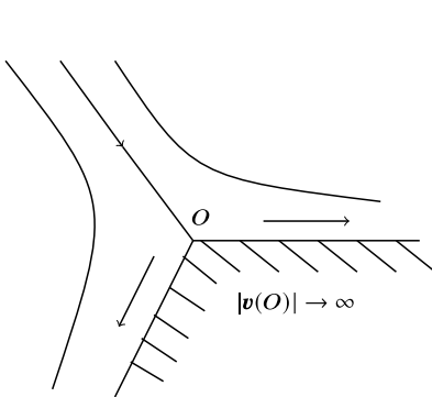
Fig. 6.10 Convex dihedron
