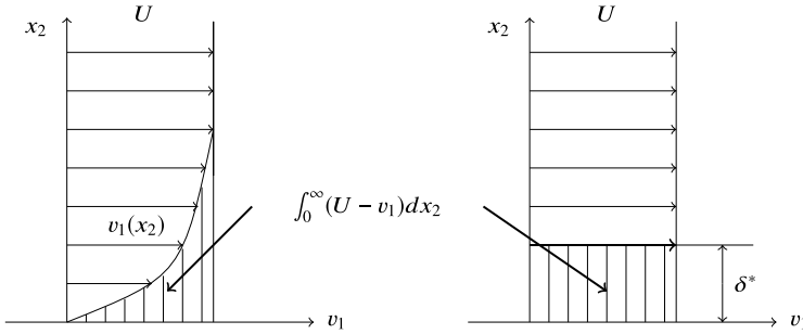
Fig. 7.4 Displacement thickness \delta^* in relation with the velocity v_1 at position x_1
