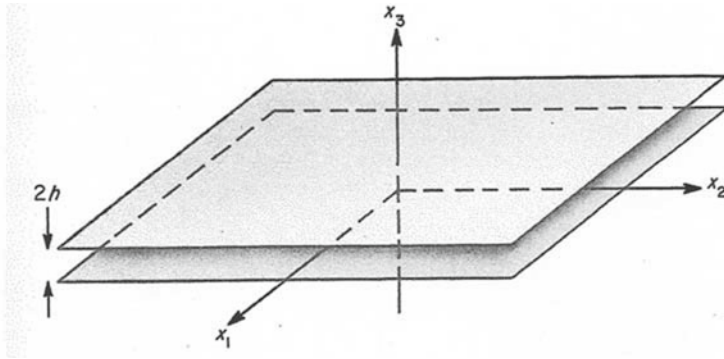
Fig. 5.7 Geometry for flow between parallel plates
