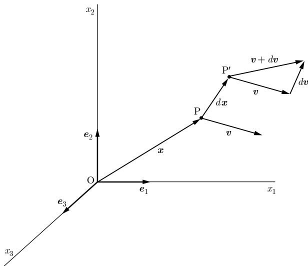
Fig. 1.9 Relative motion of two fluid particles
